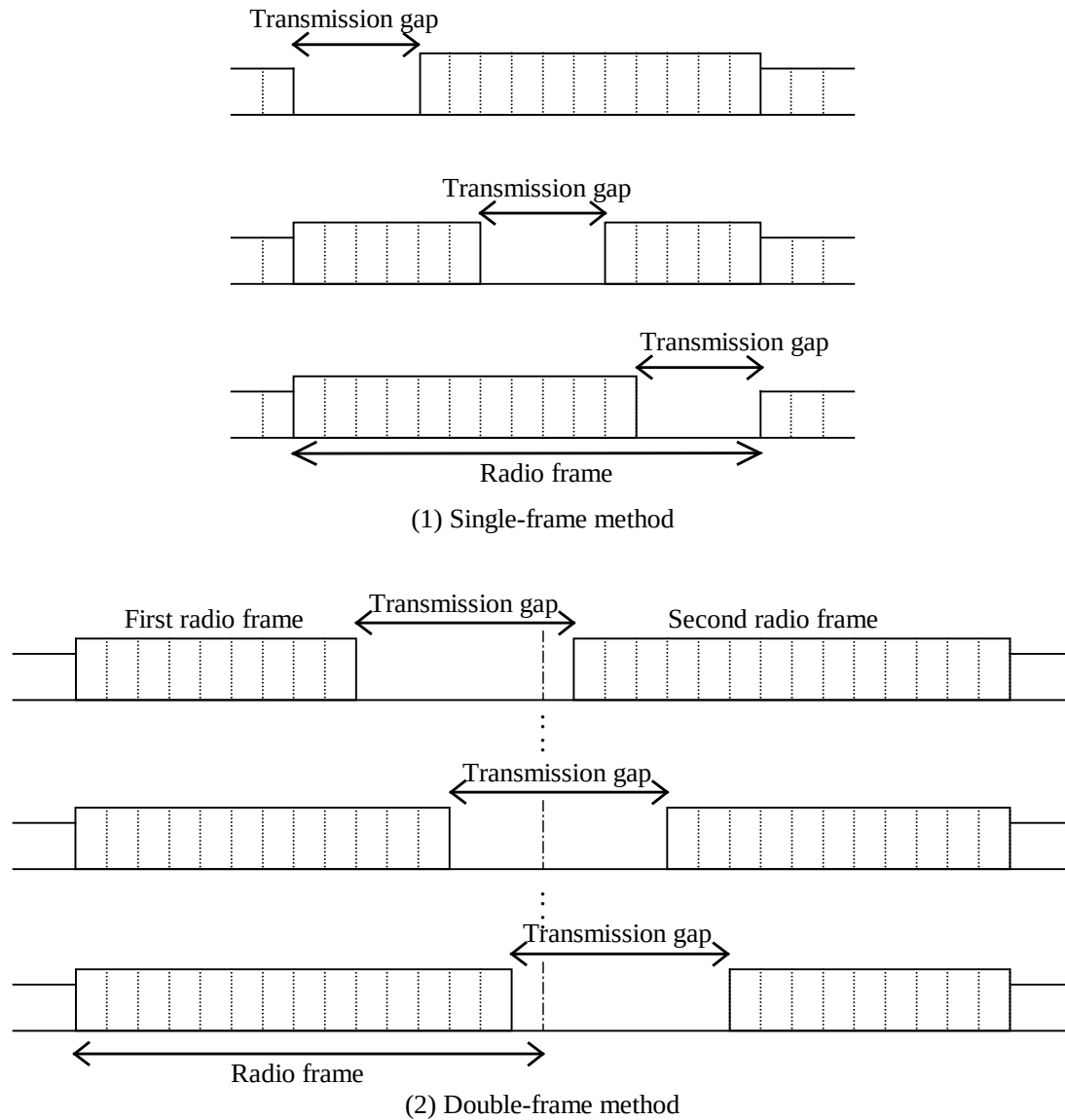
Figure 15: Transmission gap positions with different N_{\text{first}}
