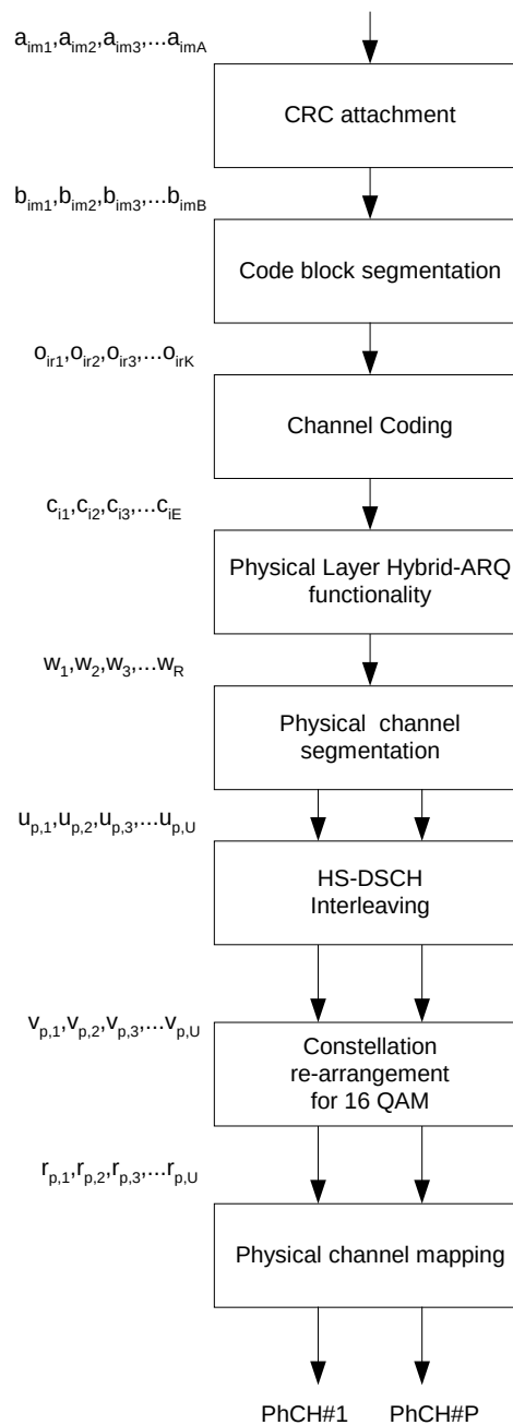
Figure 16: Coding chain for HS-DSCH
