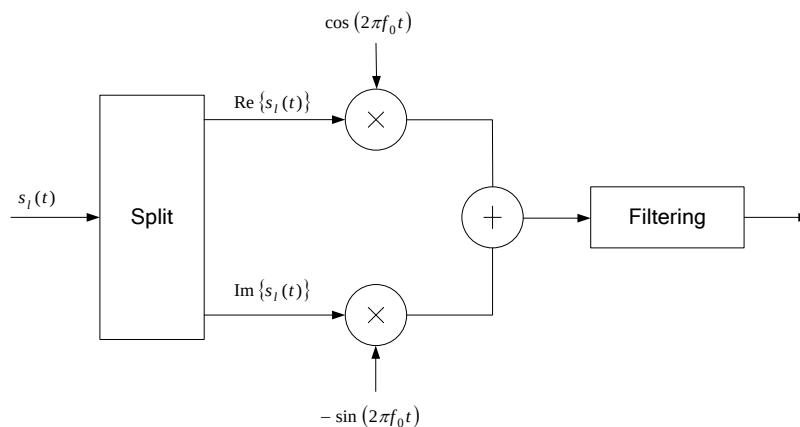
Figure 5.8-1: Uplink modulation.
