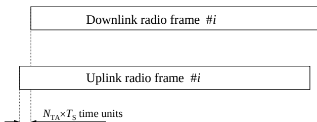
Figure 8.1-1: Uplink-downlink timing relation
