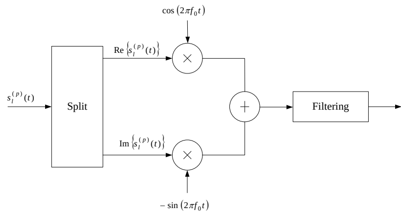
Figure 6.13-1: Downlink modulation.
