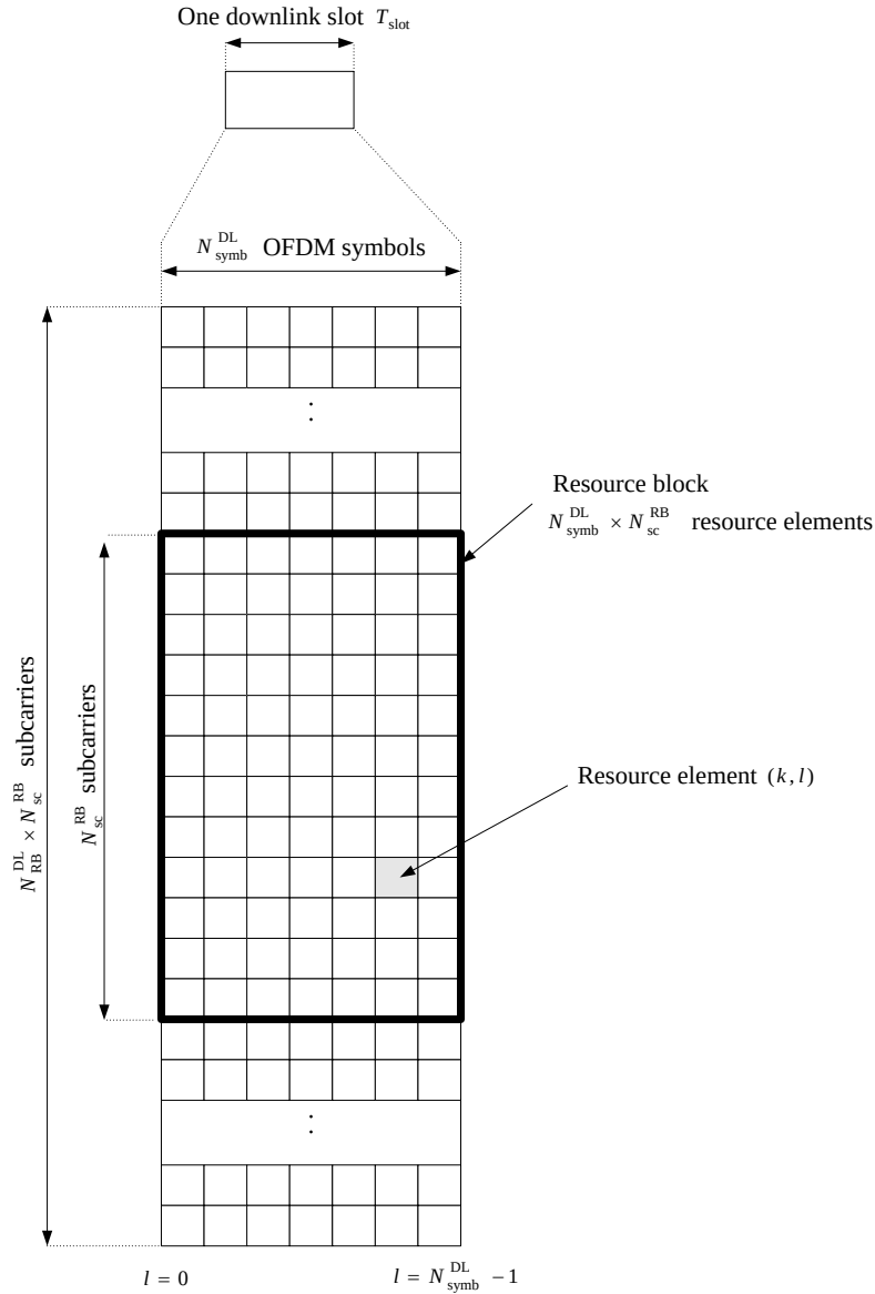
Figure 6.2.2-1: Downlink resource grid.
