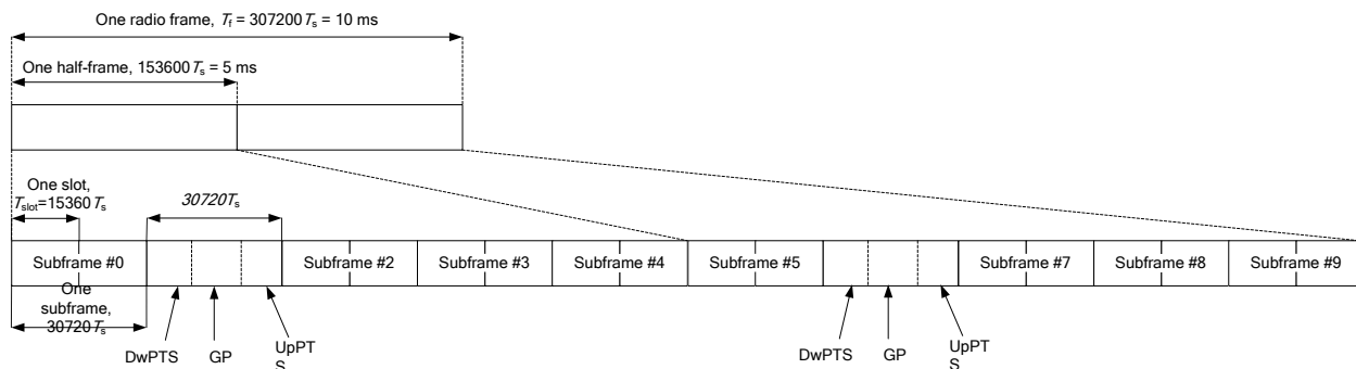
Figure 4.2-1: Frame structure type 2.
