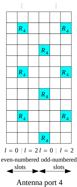
Figure 6.10.2.2-3: Mapping of MBSFN reference signals (extended cyclic prefix, \Delta f = 7.5\text{ kHz} )
