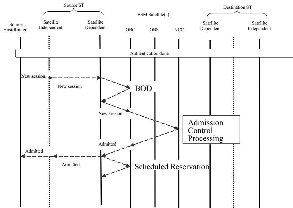
Figure 16: Admission Control process for RSM
