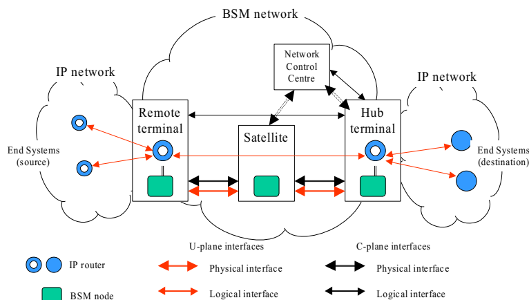
Figure 5: Access BSM [11], [12]
