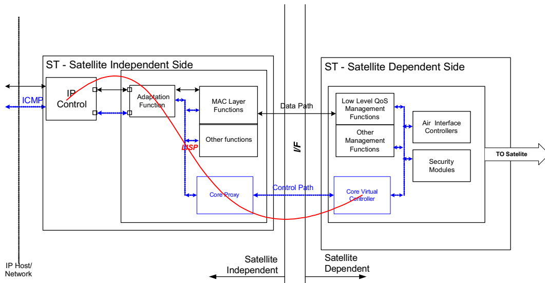
Figure C.1: LISP overview
