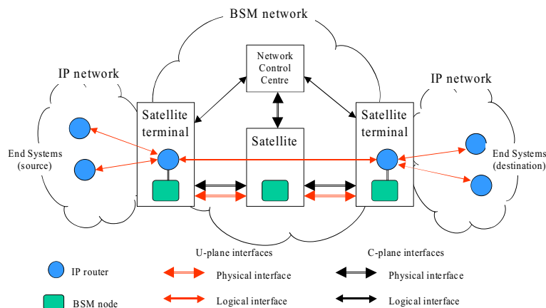
Figure 7: Meshed BSM [11], [12]
