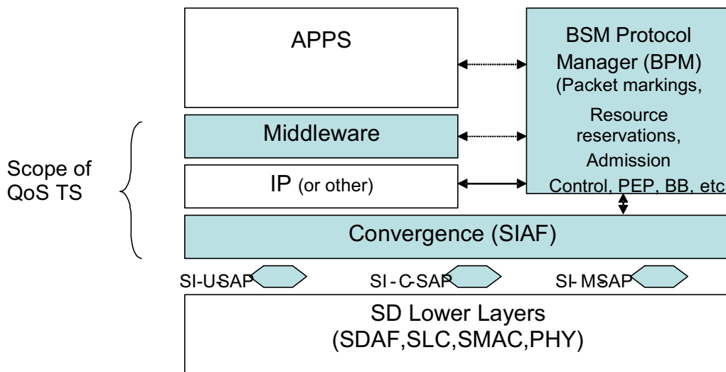
Figure 19: Protocol manager - System architecture
