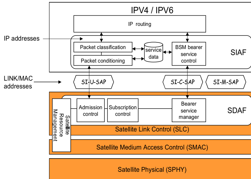
Figure 8: QoS functional model [12]
