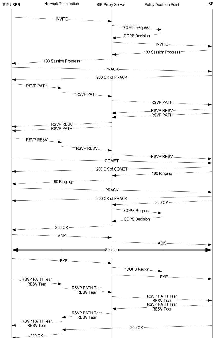
Figure 12: Interaction of SIP, COPS and RSVP
