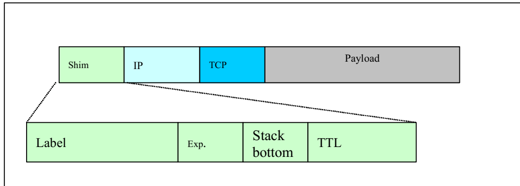
Figure 15: MPLS packet formats
