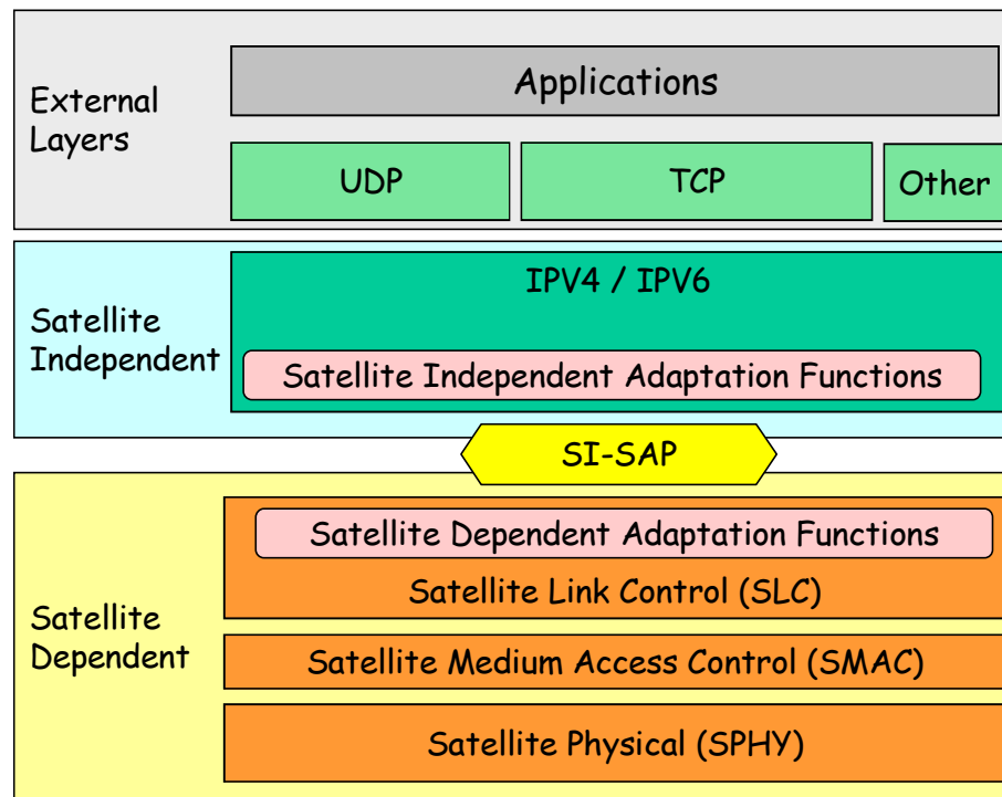
Figure 3: Protocol architecture [11]
