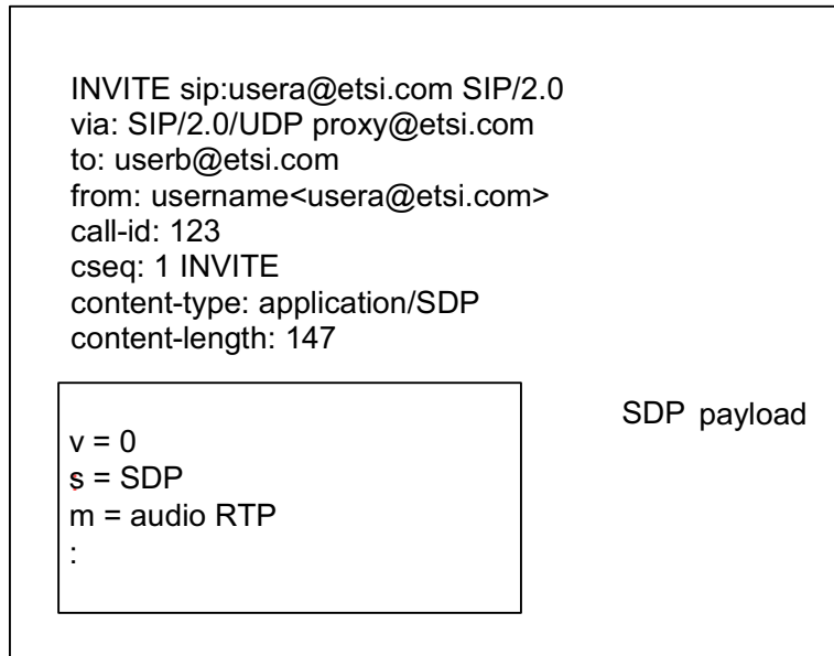
Figure 11: SIP syntax [67]
