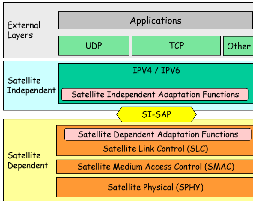
Figure 5.3.1: Protocol architecture
