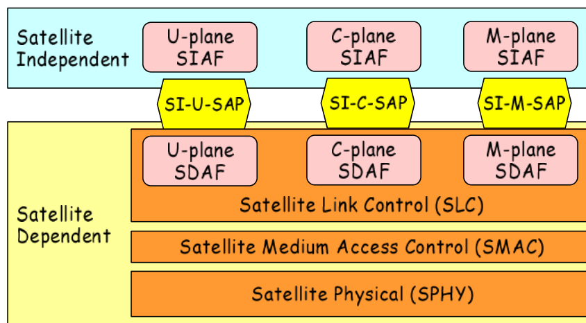
Figure 5.3.2: SI-SAP reference model
