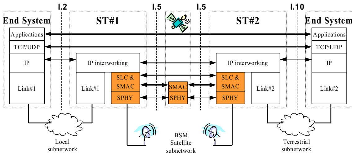
Figure 5.3.3.3: IP interworking functions
