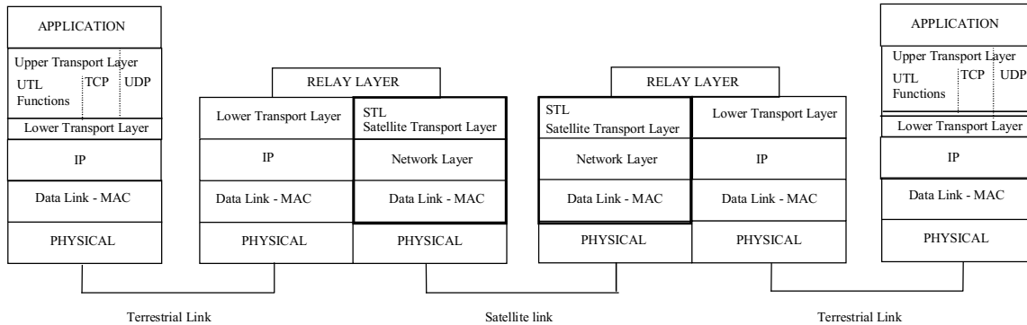
Figure 12.4.1: Example of modified Transport Layer protocol
