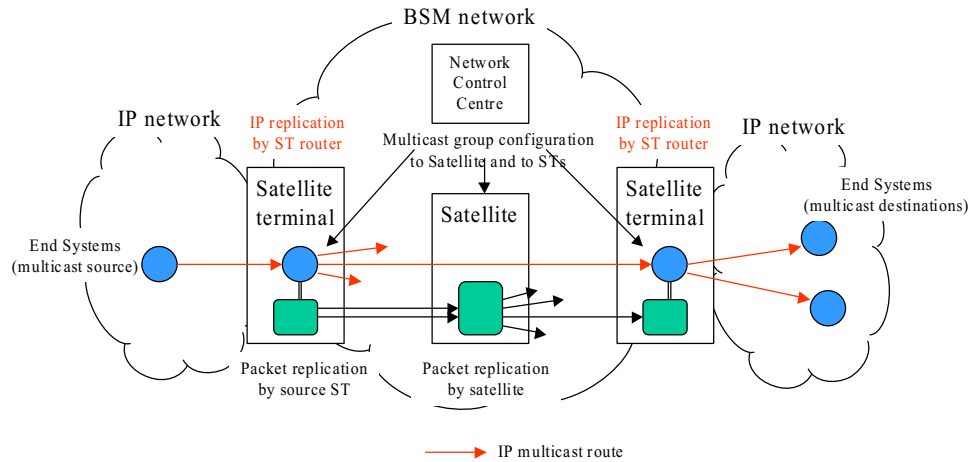
Figure 10.2.1: IP Multicast model (forward direction)
