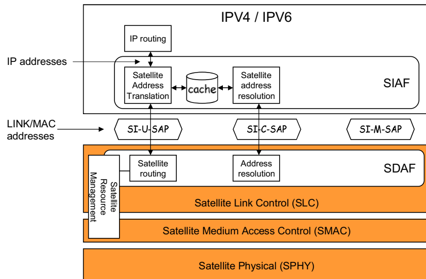
Figure 9.2.2: Address and Routing reference model
