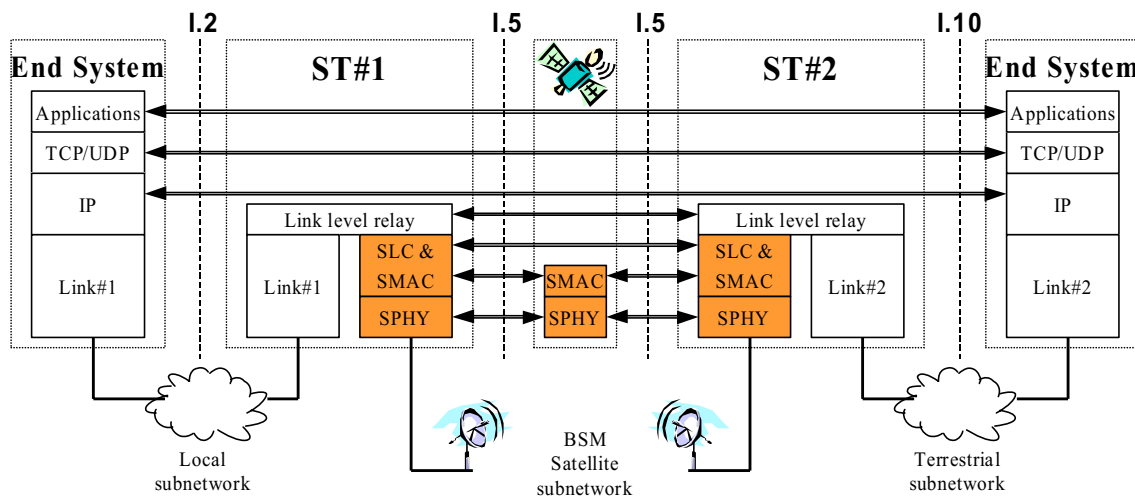
Figure 5.3.3.2: Bridge interworking functions
