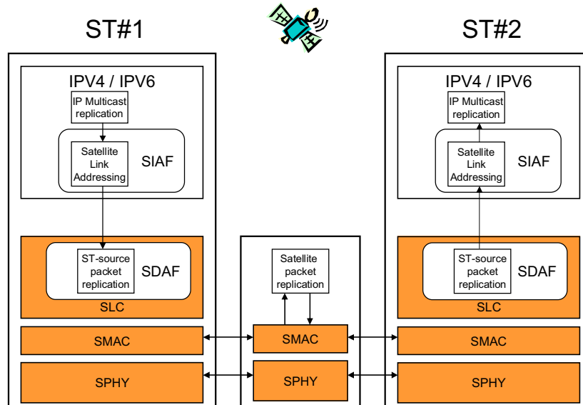
Figure 10.2.3: Replication functional model
