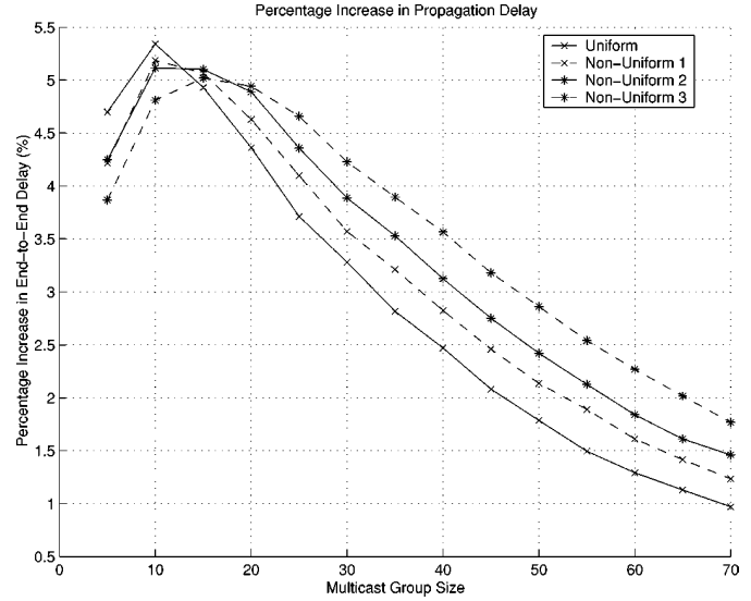
Fig. 6. Percentage increase in propagation delay.
