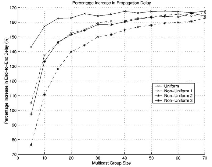
Fig. 11. Percentage increase in propagation delay for CBT.
