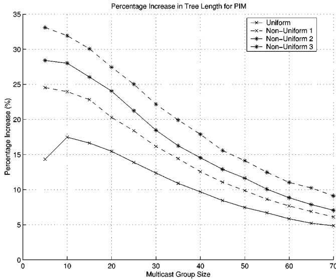
Fig. 9. Percentage increase in tree length for PIM.
