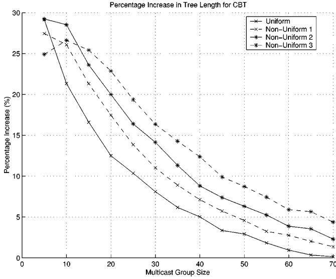
Fig. 10. Percentage increase in tree length for CBT.
