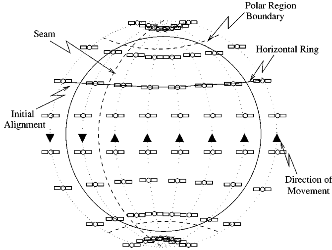
Fig. 1. Orbital planes around the Earth.
