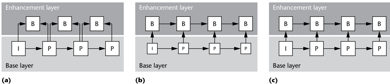
Figure 5. Examples of frame-based scalabilities. (a) Temporal scalability, (b) spatial scalability, and (c) signal-to-noise ratio scalability.
