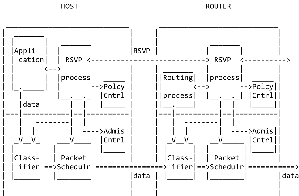
Figure 1: RSVP in Hosts and Routers
