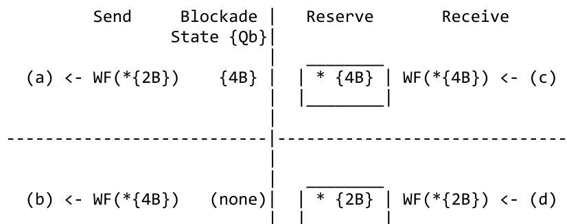
Figure 12: Blockading with Shared Style
