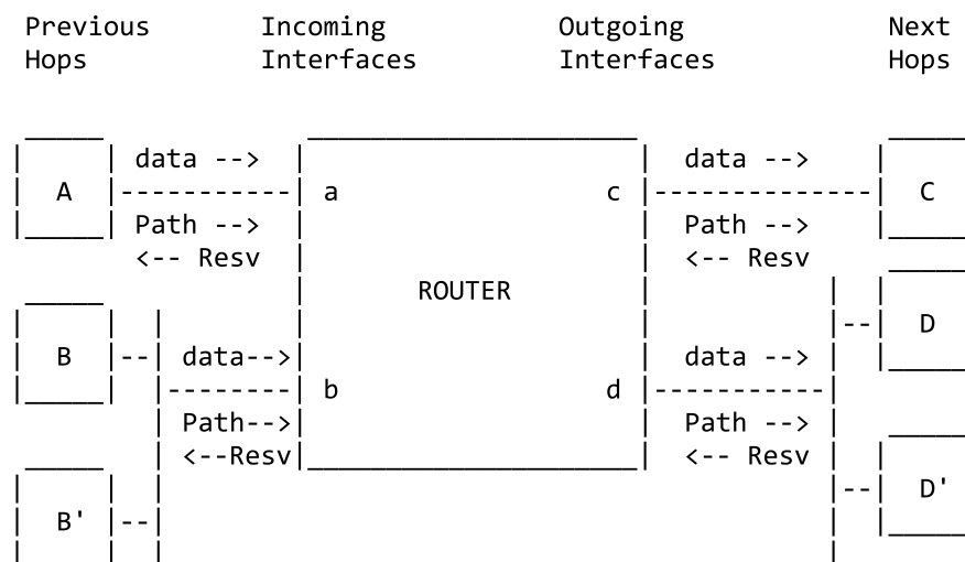
Figure 9: Router Using RSVP
