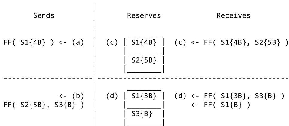
Figure 6: Fixed-Filter (FF) Reservation Example
