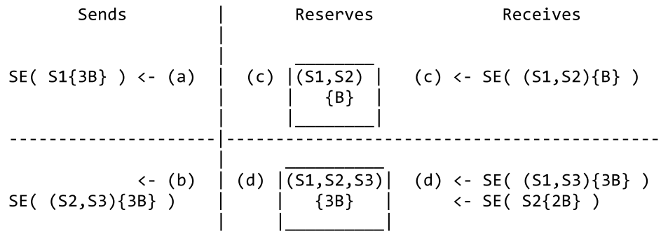
Figure 7: Shared-Explicit (SE) Reservation Example
