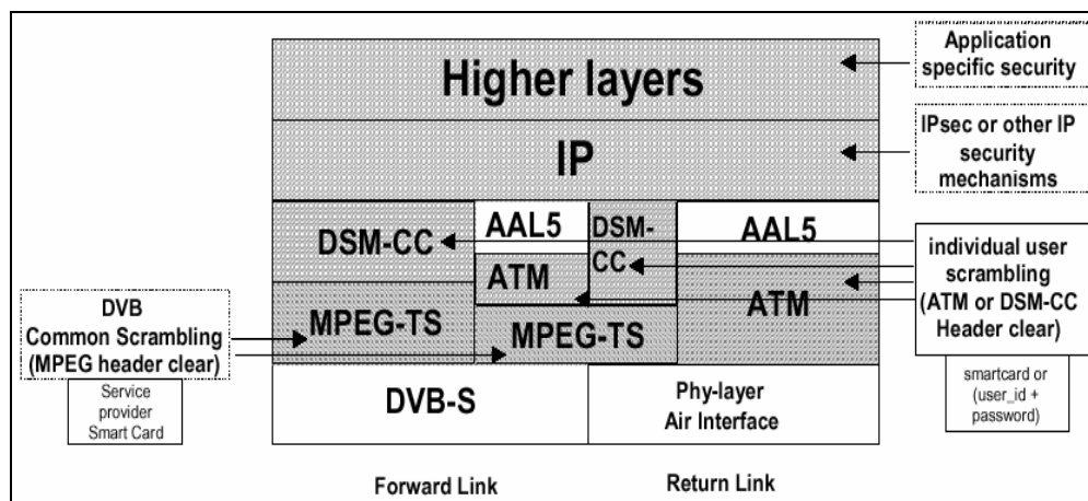
Figure A.1: IP stack in DVB-RCS
