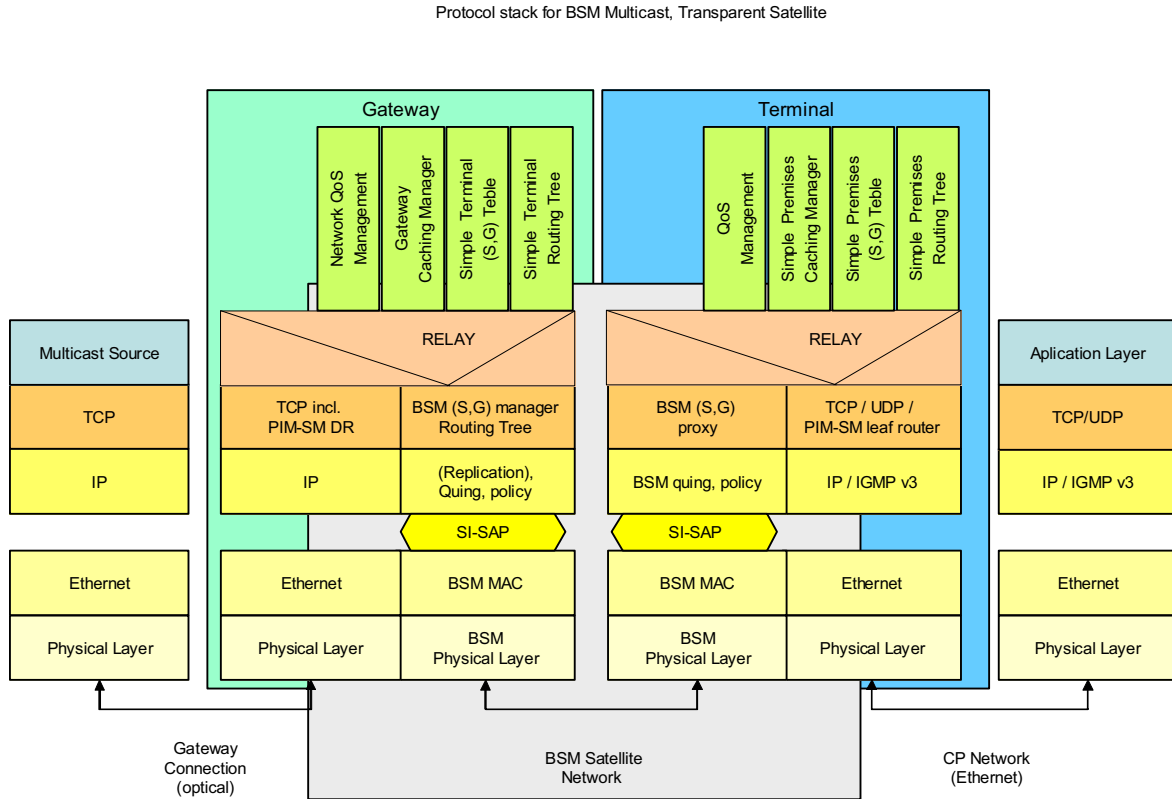
Figure 44: Draft sketch of a BSM Multicast protocol stack concept for bent pipe satellite
