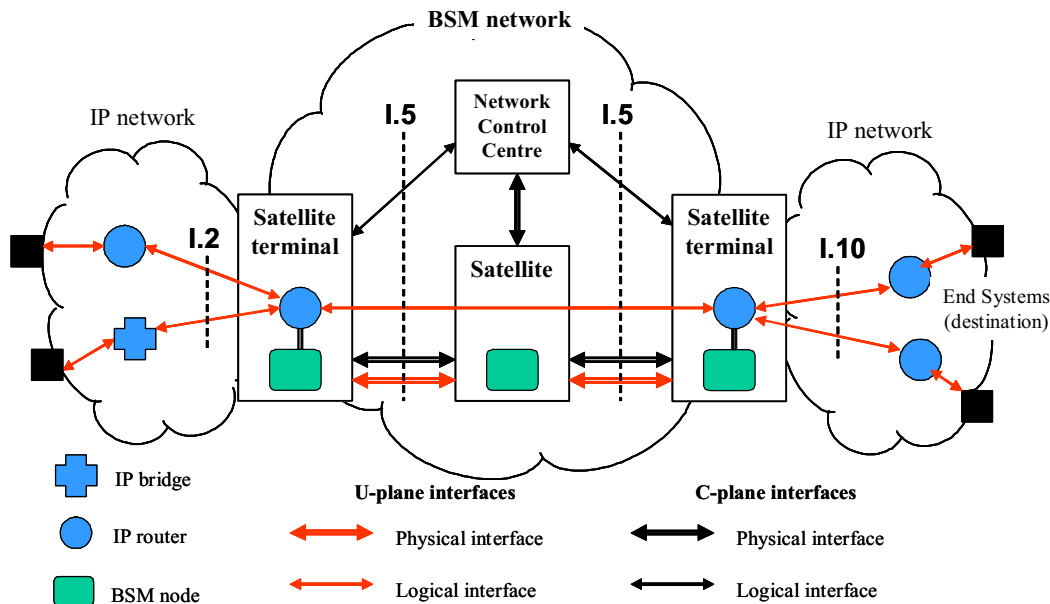
Figure 25: BSM mesh network reference
