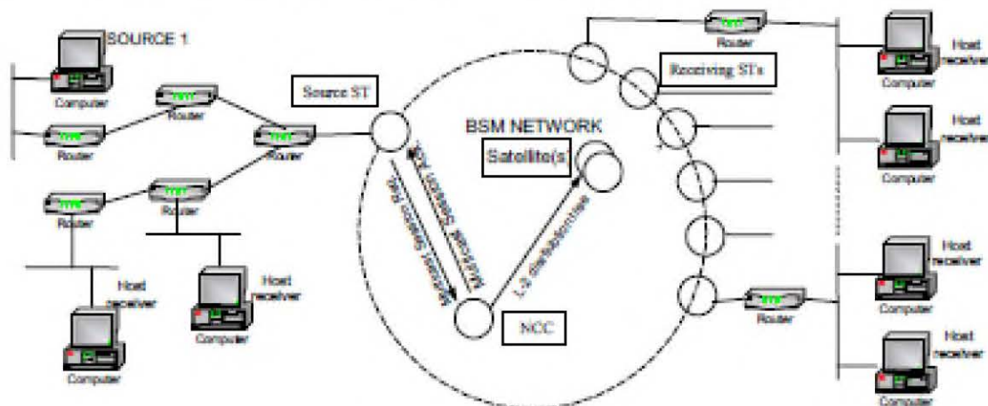
Figure 47: BSM multicast concept with drawing details
