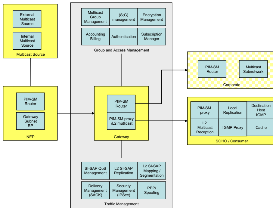
Figure 46: BSM Multicast functions
