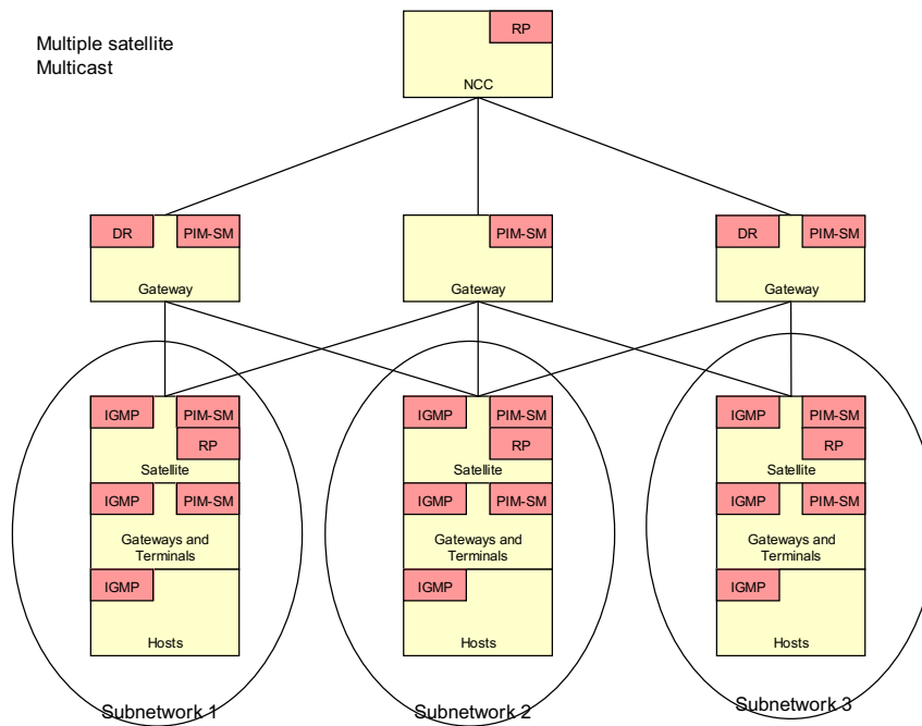
Figure 43: BSM multicast and sub-networks
