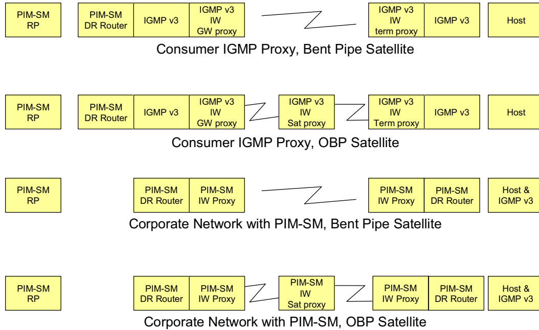
Figure 29: Alternative join/leave configurations
