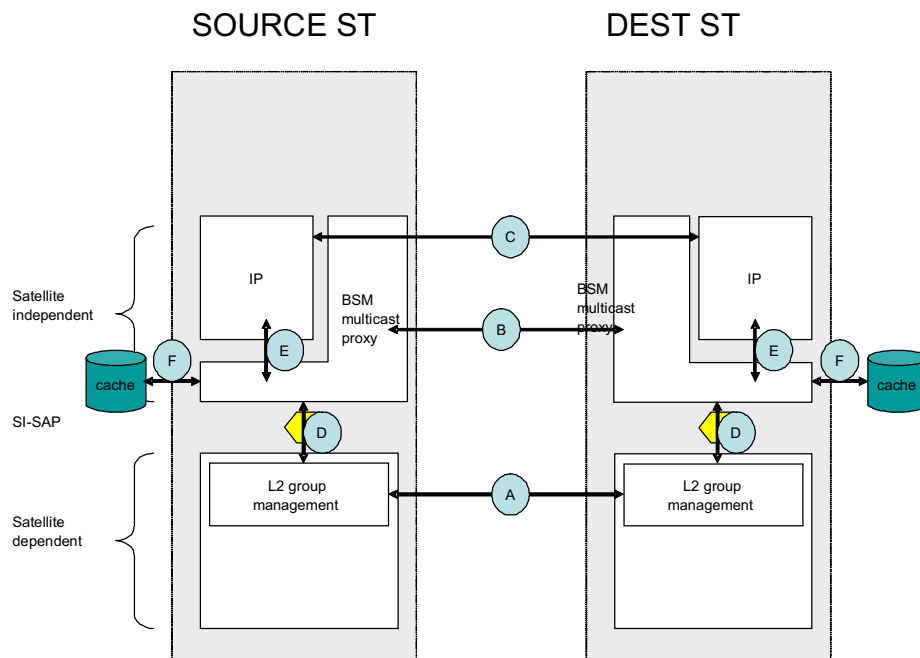
Figure 35: BSM proxy concept
