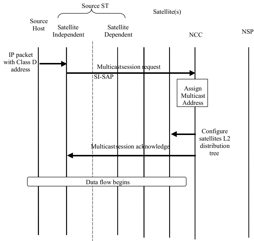
Figure 49: Setup of on-demand multicast session scenario
