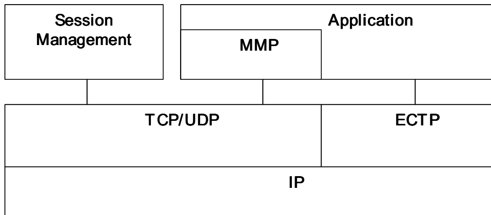
Figure 30: ITU group management overview
