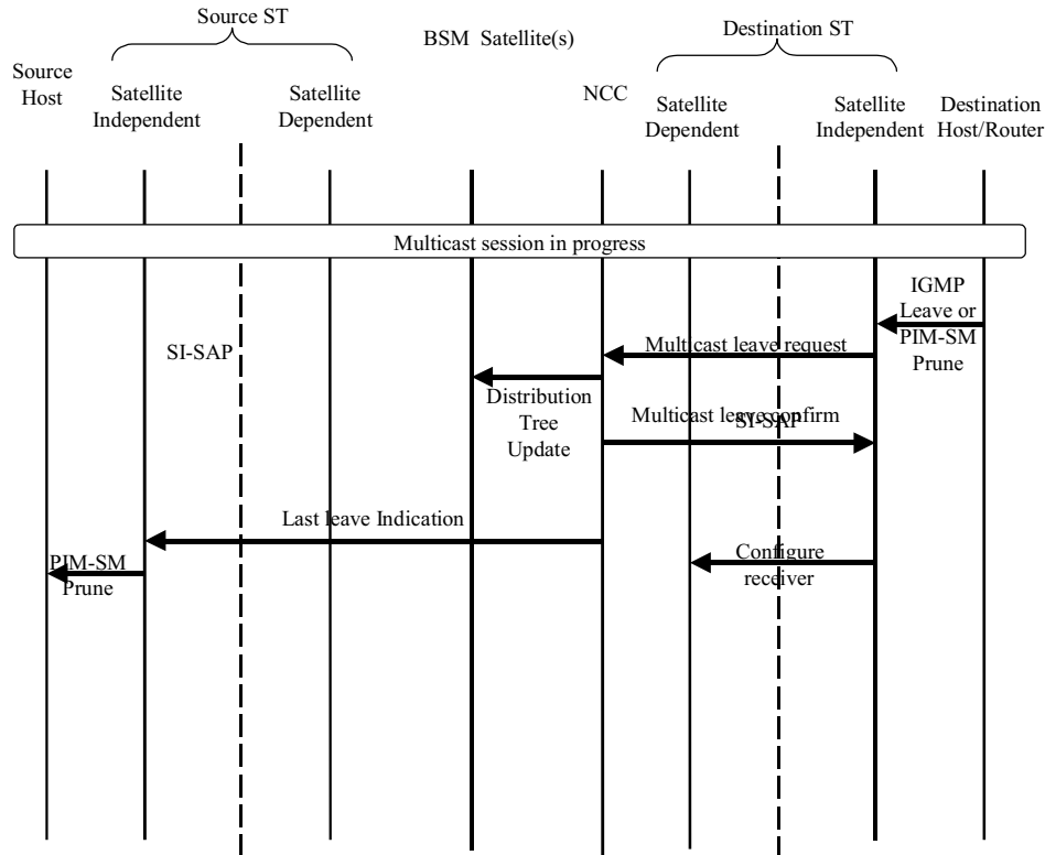
Figure 51: Dynamic leave of multicast session
