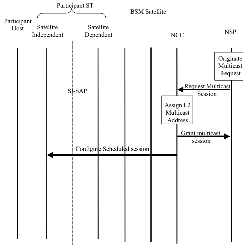
Figure 48: Setup of scheduled multicast sessions scenario
