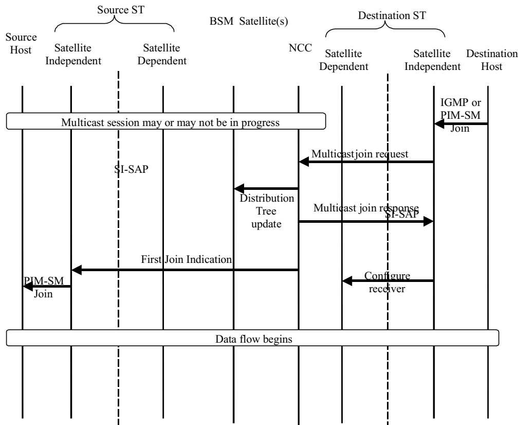
Figure 50: Dynamic join
