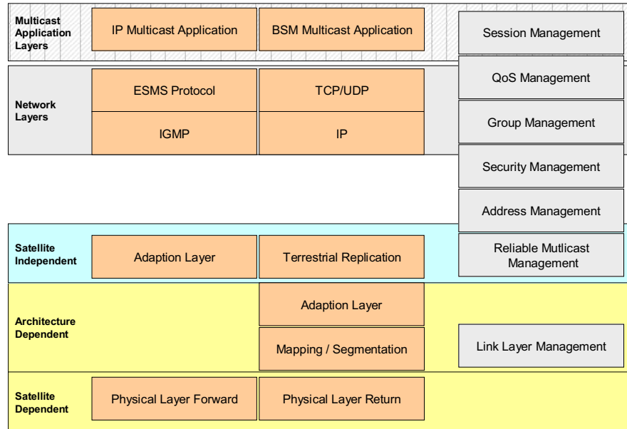
Figure 53: BSM multicast protocol layers and management functions
