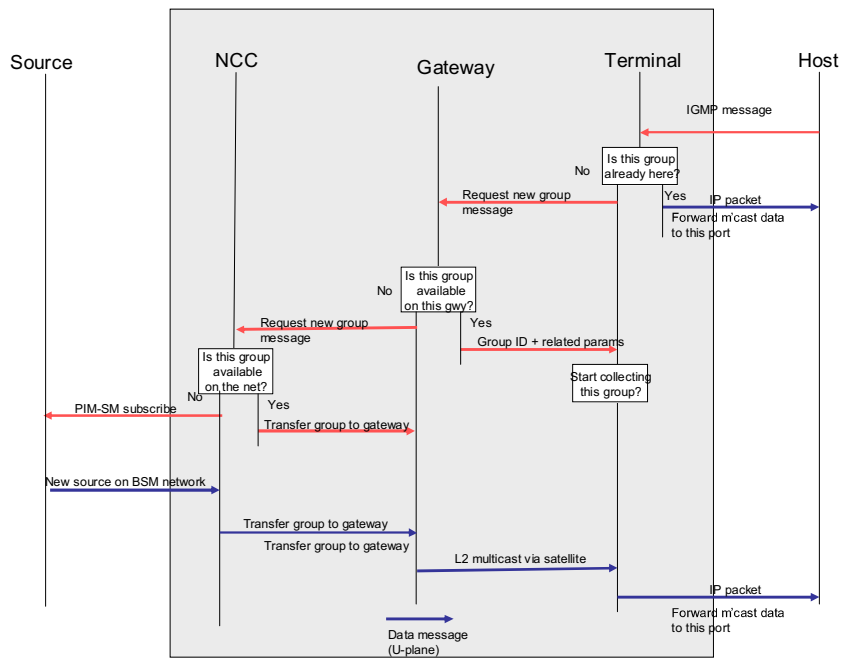
Figure 38: Interworking example
