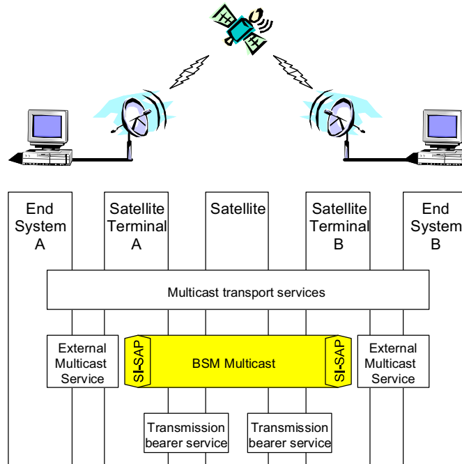
Figure 7: BSM services
