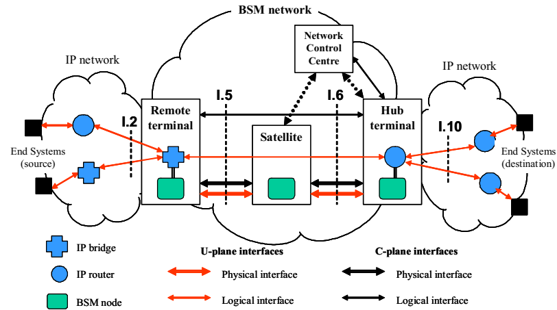
Figure 18: Star network architecture from TR 101 984
