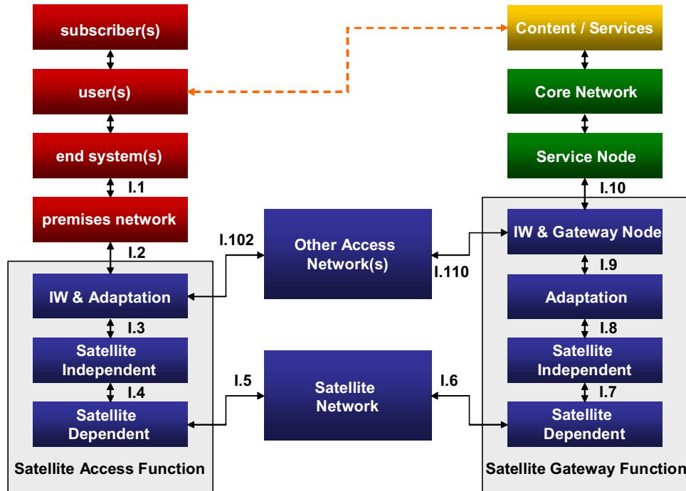
Figure 13: Detailed BSM reference architecture
