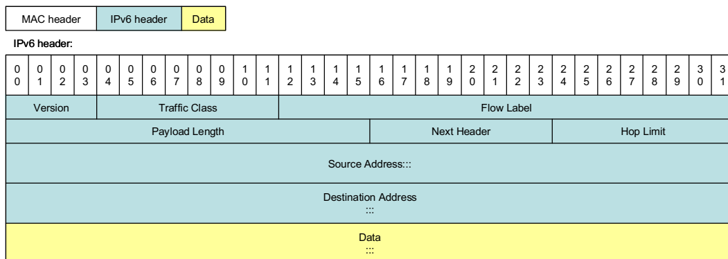
Figure 6: IPv6 header
