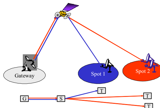
Figure 21: Single gateway, multiple spot beams
