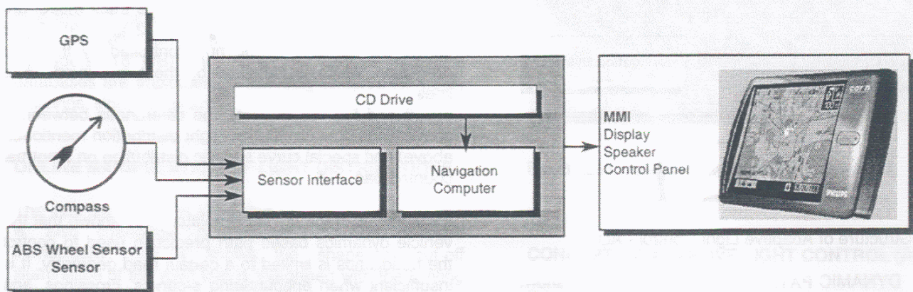
Fig. 11: Structural diagram of the navigation system
