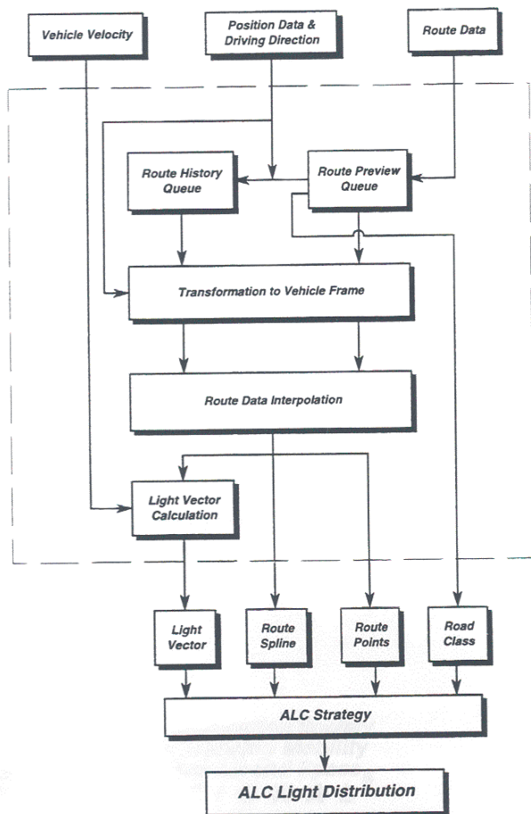
Fig.13: Interface of ALC and Navigation
