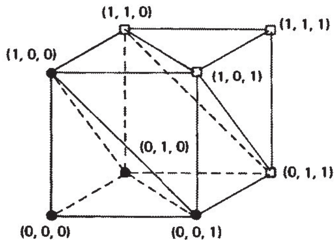
Figure 3-6.1 Three-dimensional spheres about (0, 0, 0) and (1, 1, 1)
