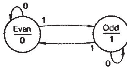
Figure 2.2-1 Parity count circuit
