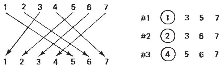
Figure 3-5.1 Hamming code positions
