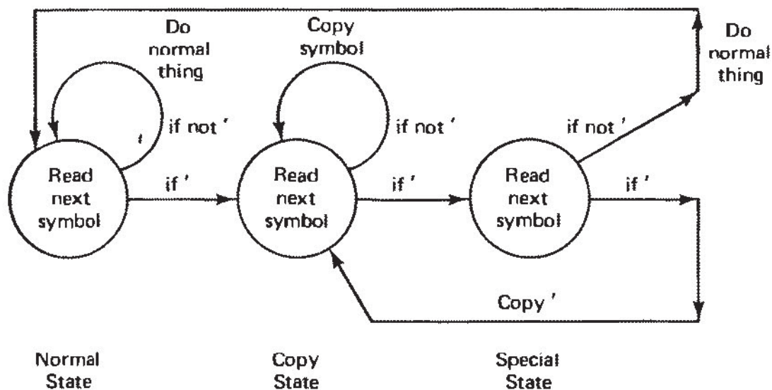
Figure 1.10-1 Reserved symbol automata
