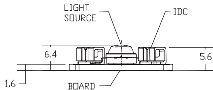
Batwing
