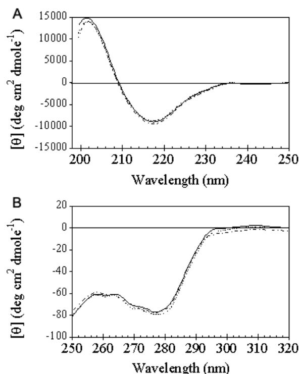
Figure 7. Circular dichroism of freeze-dried excipient-free antibody that has been stored at 30°C for 1 year and reconstituted. The rhuMAb sample was fractionated by SEC (Figure 1), and circular dichroism spectra in the (a) far- and (b) near-UV region are shown from an analysis of rhuMAb monomer (—) peak 1 as well as soluble aggregate samples (-----) peak 2 and (— — —) peak 3.
