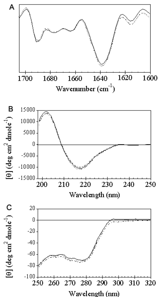
Figure 6. The effect of reconstitution on rhuMAb structure as determined by (a) second-derivative FT-IR absorbance and circular dichroism in the (b) far- and (c) near-UV regions. Samples analyzed include (—) excipient-free antibody that had not undergone lyophilization, and freeze-dried and reconstituted rhuMAb formulated (—) excipient-free and (----) with sucrose at a molar ratio of 500:1 excipient:protein.
