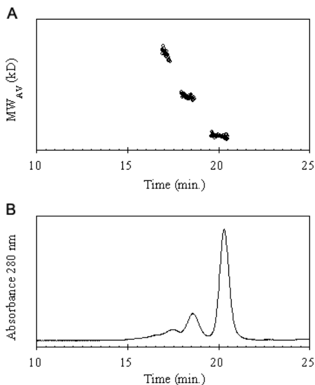
Figure 1. SEC-LS of excipient-free freeze-dried rhuMAb that had been stored for 1 year at 30°C: (A) MW AV ; (B) column elution monitored by the absorbance at 280 nm.
