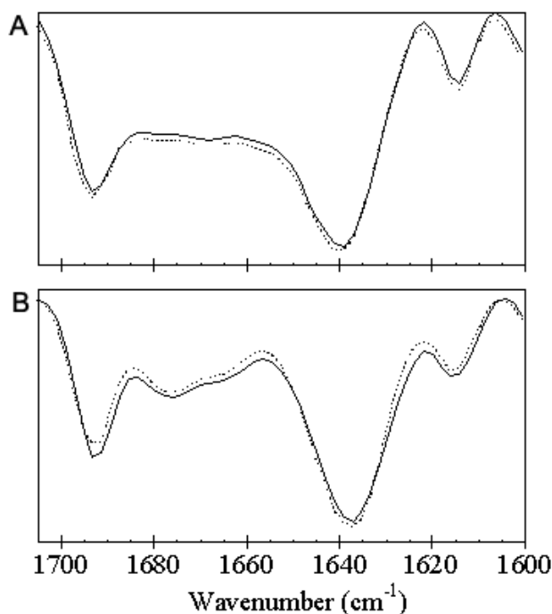
Figure 5. The effect of storage on solid-state rhuMAb structure. Second-derivative FT-IR absorbance spectra of freeze-dried protein formulated (a) excipient-free and (b) with sucrose at a molar ratio of 500:1 excipient:protein were analyzed (—) after freeze-drying and (----) following storage at 30°C for 1 year.
