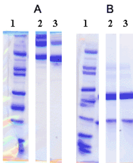
Figure 2. SDS PAGE of freeze-dried rhuMAb run under (A) nonreducing and (B) reducing conditions. Samples consists of (Lane 1) molecular weight standards and freeze-dried rhuMAb formulated (Lane 2) excipient-free and (Lane 3) with sucrose at a molar ratio of 500:1 excipient:protein. Freeze-dried rhuMAb samples were stored at 30°C for 1 year prior to the analysis.
