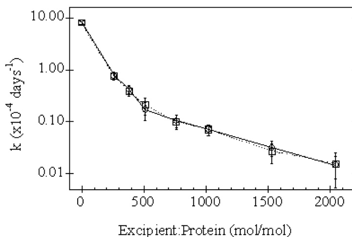
Figure 3. Soluble aggregation kinetics of freeze-dried rhuMAb formulated excipient-free and with various concentrations of (open circles) sucrose and (open squares) trehalose. Pseudo first-order rate constants were determined from samples stored at 30°C for up to 1 year.
