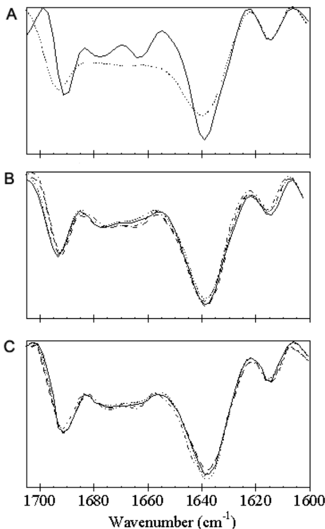
Figure 4. The effect of freeze-drying on rhuMAB secondary structure. Second-derivative FT-IR absorbance spectra are shown from an analysis of (a) excipient-free (—) aqueous and (----) freeze-dried rhuMAB as well as freeze-dried protein formulated with (b) sucrose and (c) trehalose at a molar ratio of (—) 260:1, (----) 384:1, (.....) 500:1, and (— · — · —) 1000:1 excipient:protein.
