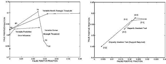
Figure 4. ROC curves showing the effect of various program parameters.
