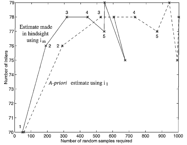
Figure 3. Inliers after motion calculation against an estimate of the number of random samples required, under different stereo match multiplicity. Each '*' represents a different stereo match multiplicity.
