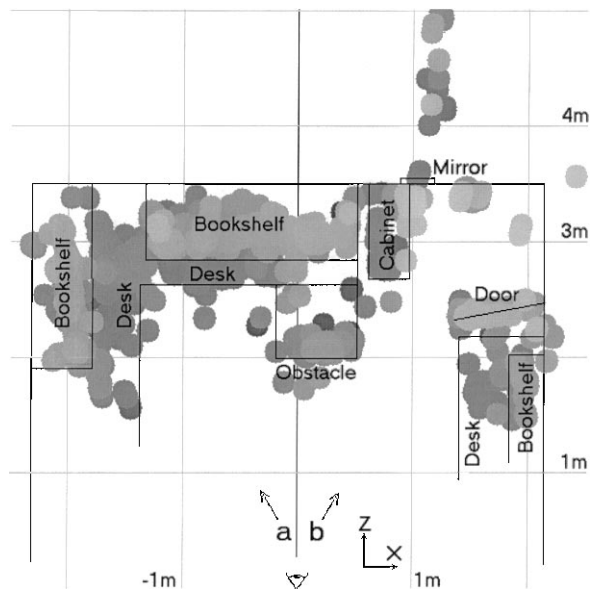
Figure 7. Point reconstruction of the indoor scene.
