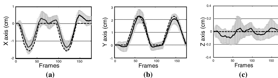
Fig. 4. Simulation based analysis of camera motion estimation. The graphs shown in (a-c) illustrate the recovered stereoscope movement in the X, Y and Z axes, respectively against the ground truth. The solid black line shows the estimated motion with the grey bars indicating the uncertainty associated with the estimate. The dotted line displays the ground truth motion.
