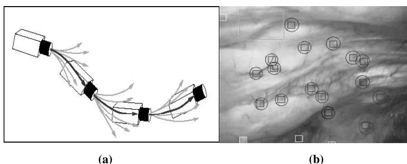
Fig. 2. (a) Visualization of the model for ‘smooth’ motion: at each camera position a most likely path is predicted together with alternatives with small deviations. (b) A MIS scene where 25×25 pixel box represent feature patches detected using the Shi and Thomasi operator [10] and ellipses represent the estimated search regions for the landmarks.
