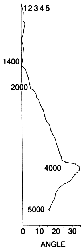
Fig. 8.135—Data showing constant inclination.
