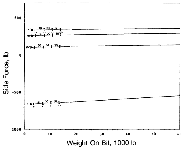
Fig. 8.141—Effect of geology on performance of Holding BHA No. 2 (12 1/2-in. hole, 9-lbm/gal mud, 8-in. collar).
