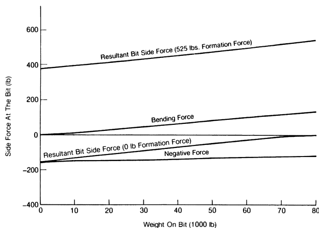
Fig. 8.127—Results of BHA calculation for slick BHA.
