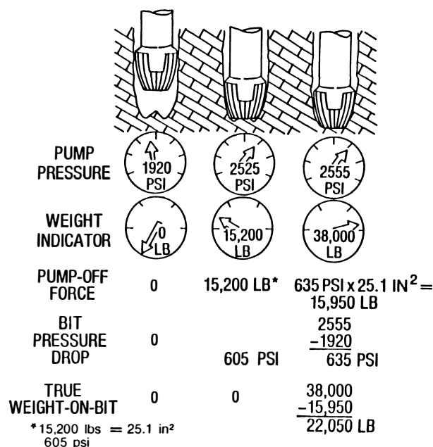
Fig. 8.110—Pumpoff pressure and weight (after Winters and Warren 16 ).
