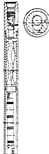
1/2 Lobe PDM
