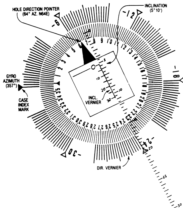
Fig. 8.71—Gyroscope face.
