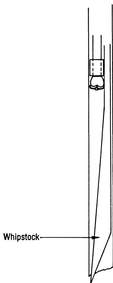
Fig. 8.86—Openhole whipstock.
