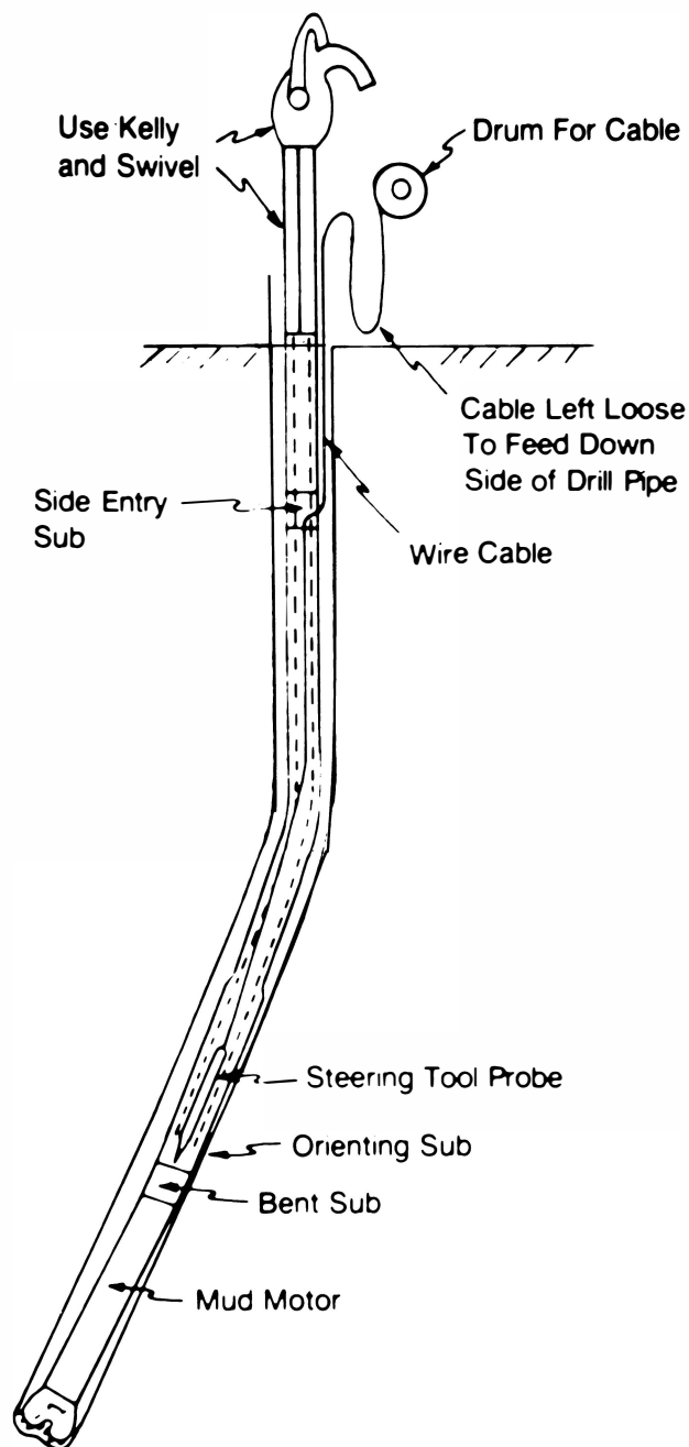
Fig. 8.55—Using a side-entry sub with a steering tool.
