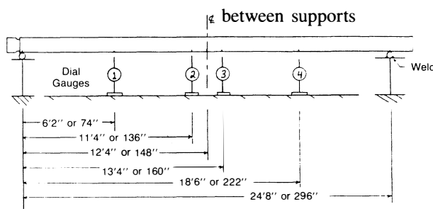
Fig. 8.166—Deflections measured in testing a mud motor—Problem 8.74.
