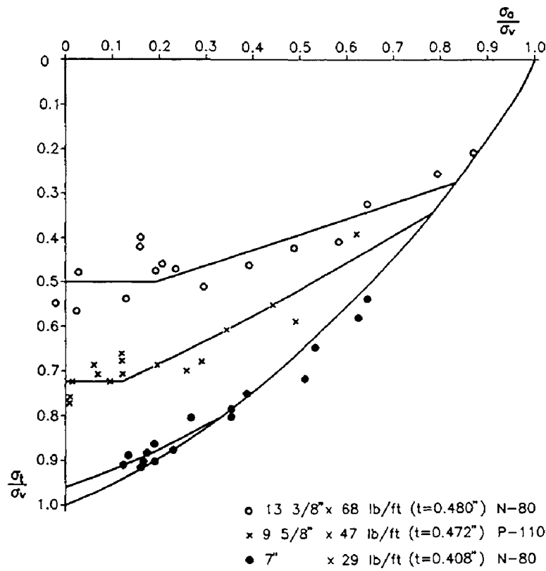
Fig. 2.21: Collapse strength under combined loads. (After Krug, 1982; courtesy of IPE-TU Clausthal.)
