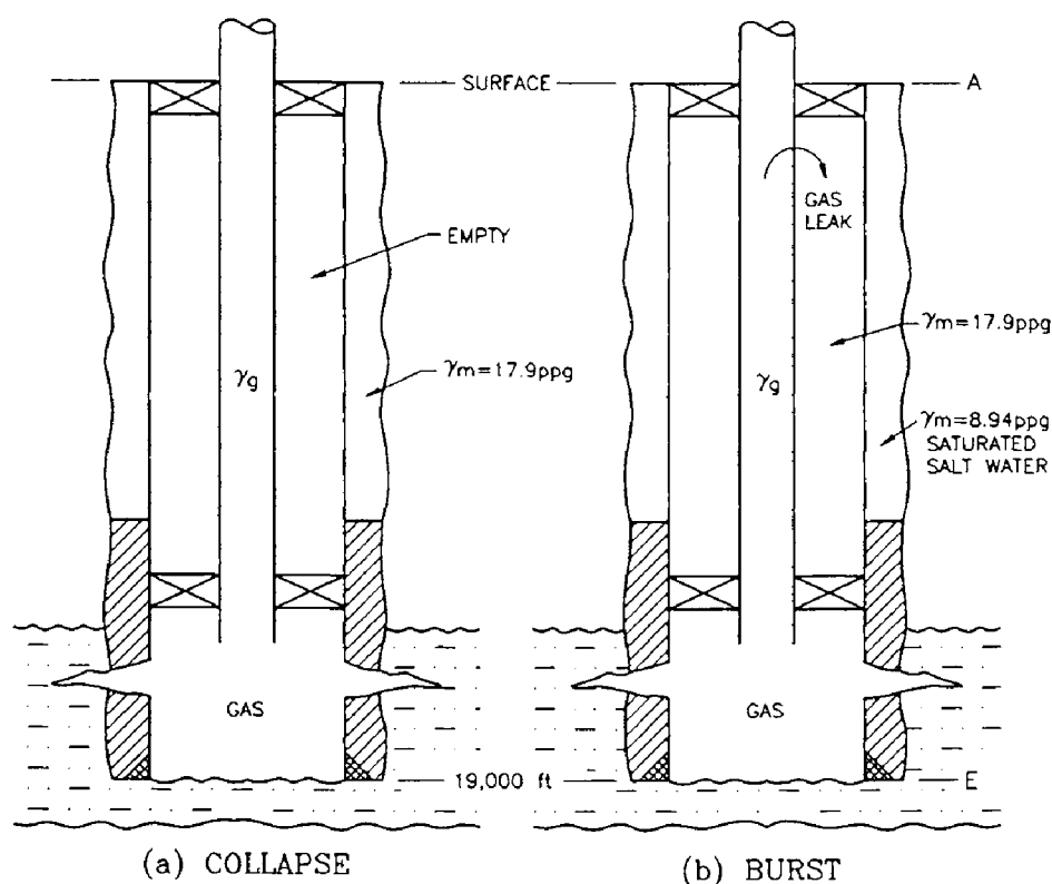
Fig. 3.13: Collapse and burst loads on the production casing.
