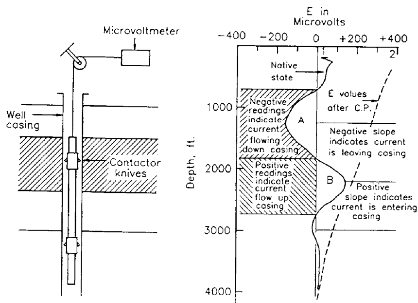
Fig. 6.1: Casing potential profile test equipment and example of plotting data. (After Jones, 1988, p.66, fig 1.8-2; courtesy of OGCI Publications, Tulsa, OK.)
