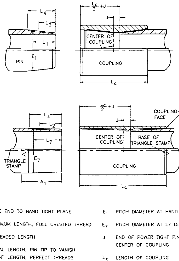
Fig. 1.6: Basic axial dimensions of casing couplings: API Round threads (top), API Buttress threads (bottom).
