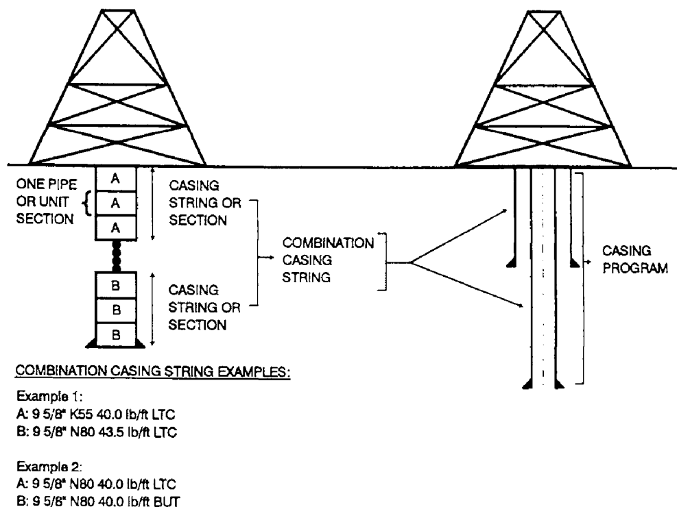
Fig. 5.1: Casing nomenclature.
