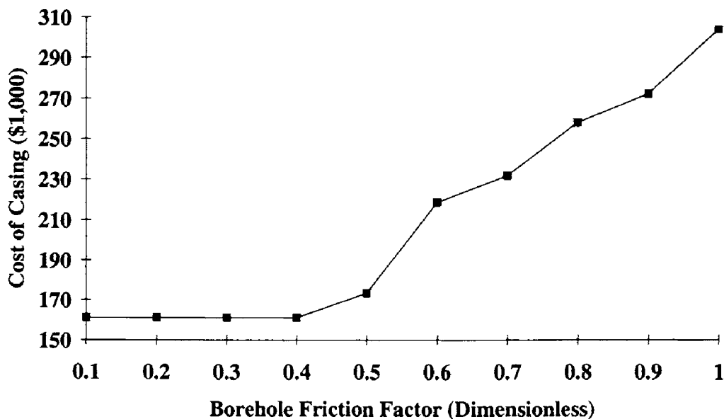
Fig. 5.10: Effect of the pseudo-friction factor on casing cost.
