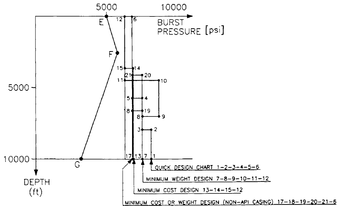
Fig. 5.6: Casing load study for burst.
