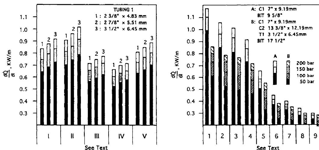
Fig. 4.37: Radial heat flow as a function of completion techniques, Emsland. Northern Germany. (After Goetzen, 1987; courtesy of ITE-TU Clausthal.)
