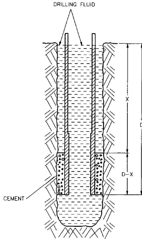
Fig. 2.27: Partially cemented casing string.
