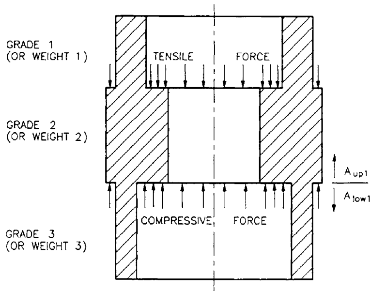
Fig. 2.28: Diagrammatic presentation of the piston effect arising from a change in internal diameter.
