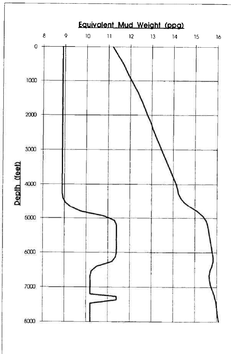
Fig. 5.13: Pore pressures and fracture gradient predictions for Exercise 13.
