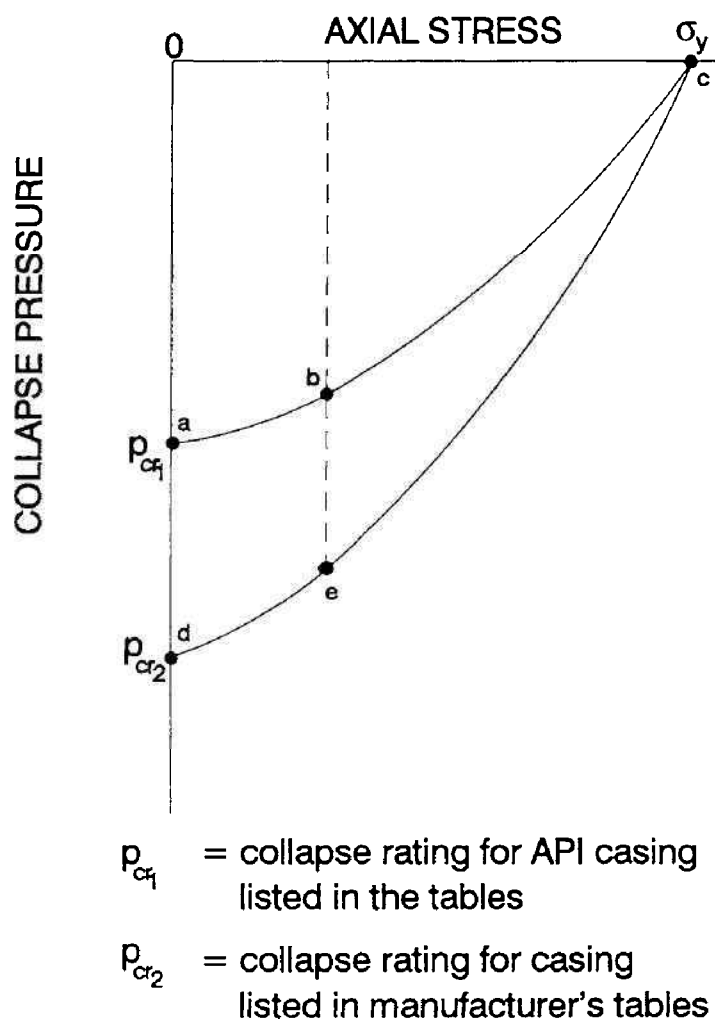
Fig. 5.7: Diagram of non-API casing collapse pressure correction.
