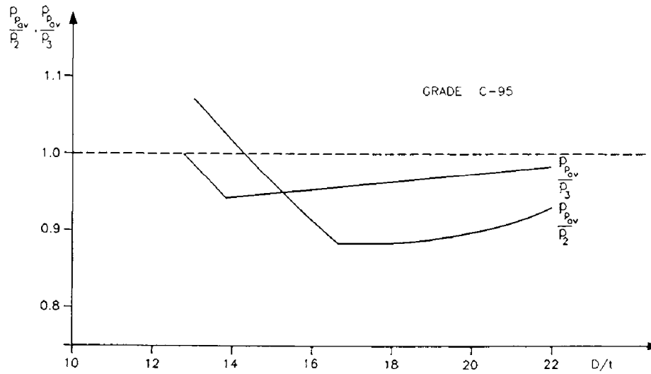
Fig. 2.17: Comparison of the average collapse strength determined in the test p_{av} , with that calculated by the methods of API ( P_2 ) and Clinedinst ( P_3 ). (After Krug and Marx, 1980; courtesy of ITE-TU Clausthal.)
