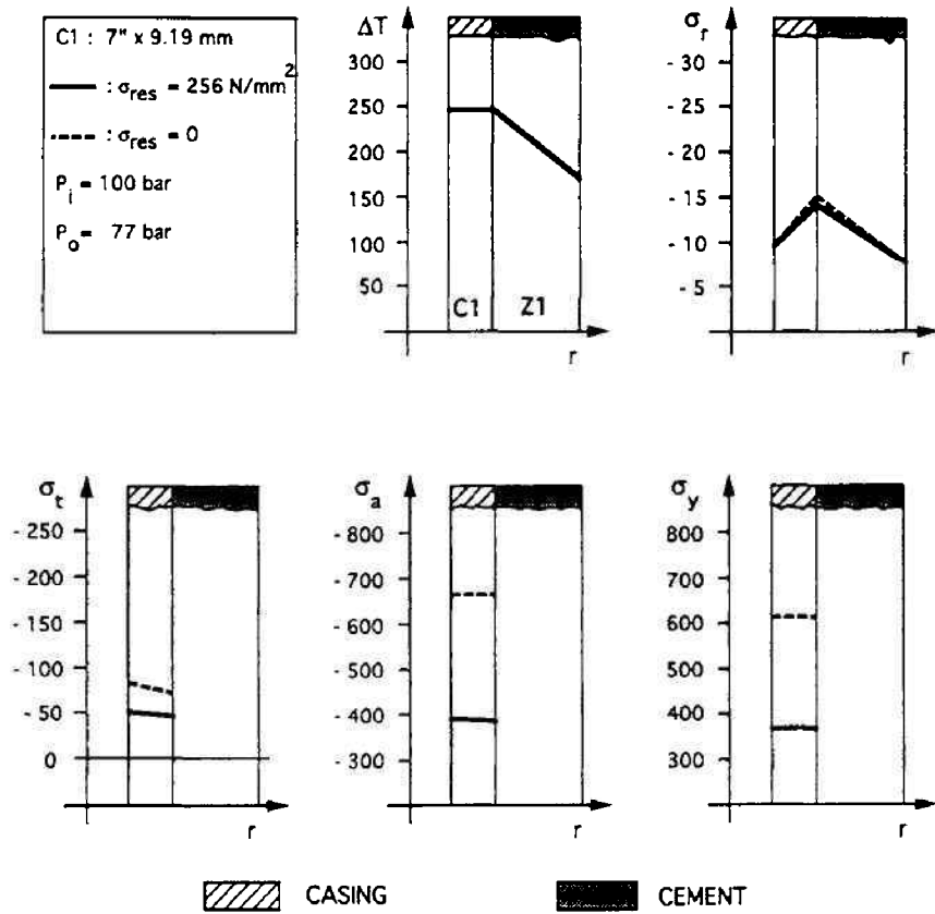
Fig. 4.30: Stress distribution in a single-casing completion with packed-off annulus ( \Delta T in ^{\circ}\text{C} and \sigma in \text{N/mm}^2 ). (After Goetzen, 1987; courtesy of ITE-TU Clausthal.)
