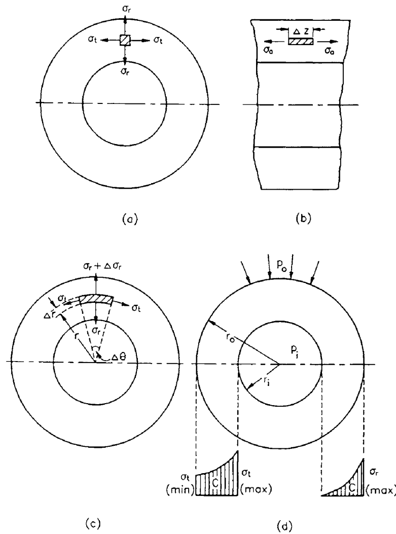
Fig. 2.10: Stresses in thick-walled casing under external pressure.
