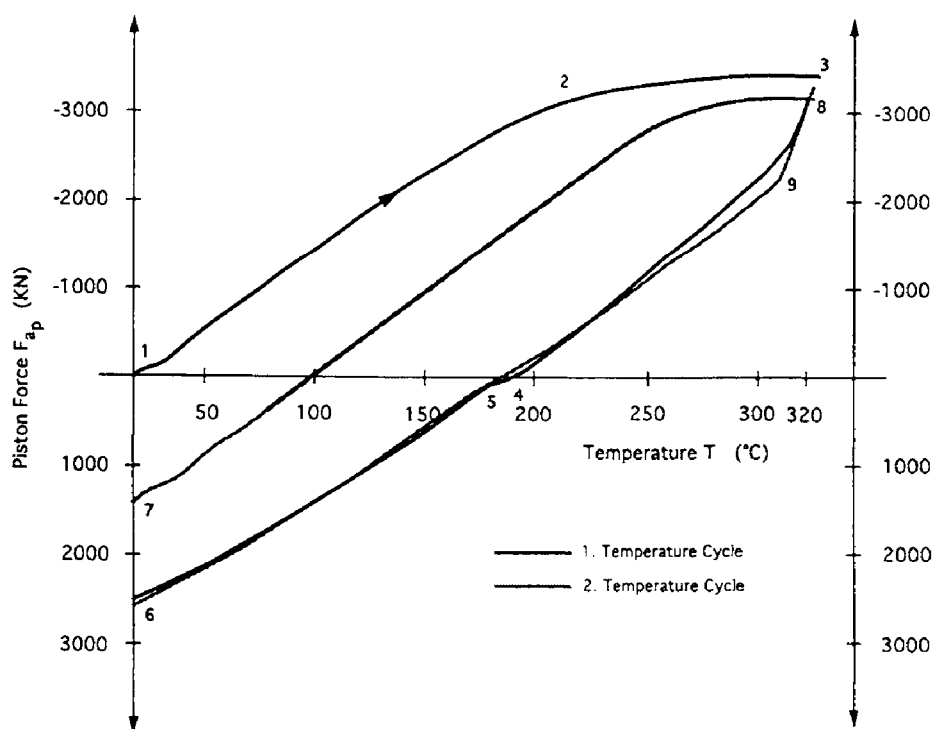
Fig. 4.40: Stress-temperature diagram for the MUST connection during cyclic heating and cooling operation. (After Goetzen, 1987; courtesy of ITE-TU Clausthal.)
