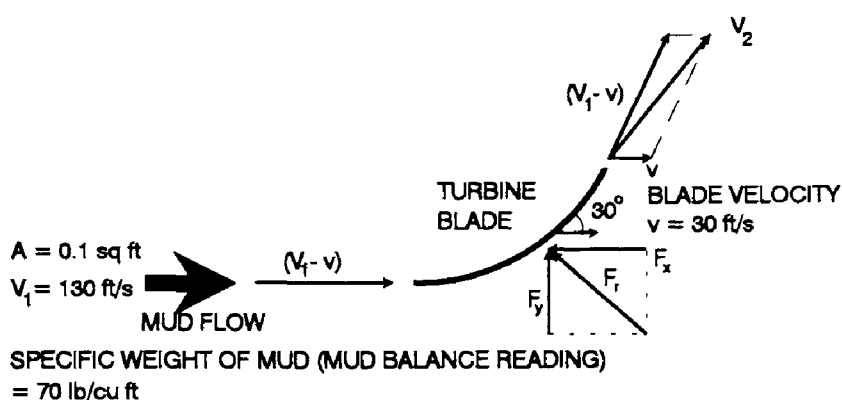
Fig. D.1: Diagram of mud jet striking blade. Example 1.
