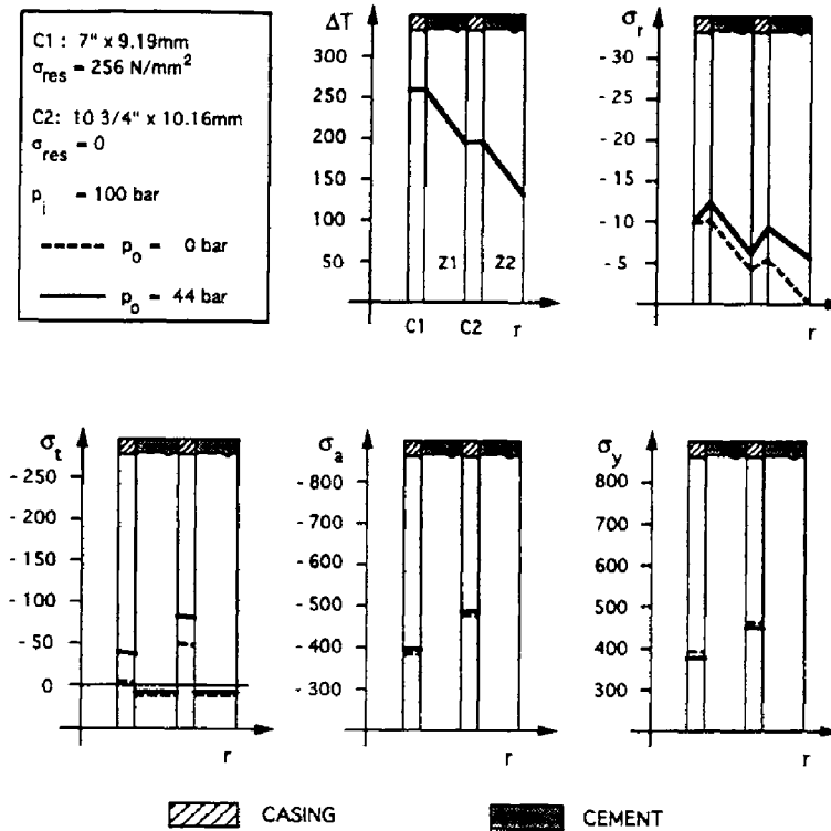
Fig. 4.31: Stress distribution in a double-casing completion with packed-off annulus ( \Delta T in ^{\circ}\text{C} and \sigma in \text{N/mm}^2 ). (After Goetzen, 1987; courtesy of ITE-TU Clausthal.)
