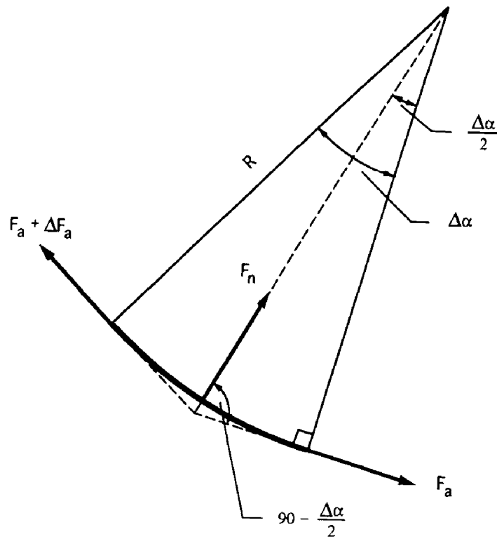
Fig. 4.3: Determination of normal force in buildup section.
