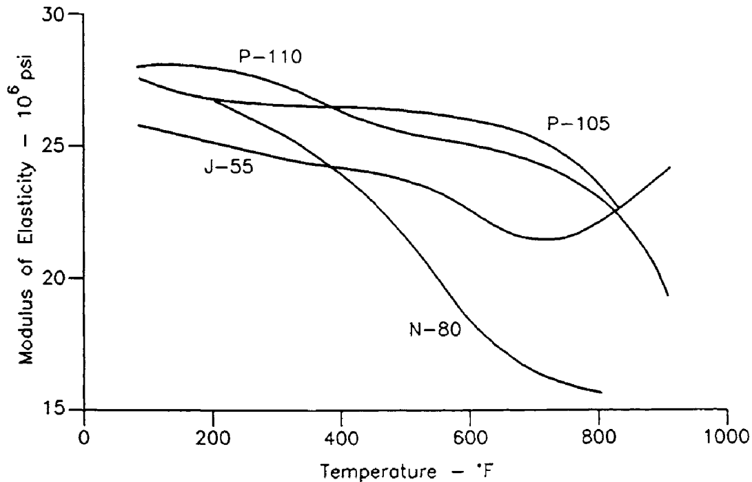
Fig. 2.29: Modulus of elasticity of steel grades as a function of temperature. (After Shryock and Smith, 1980.)
