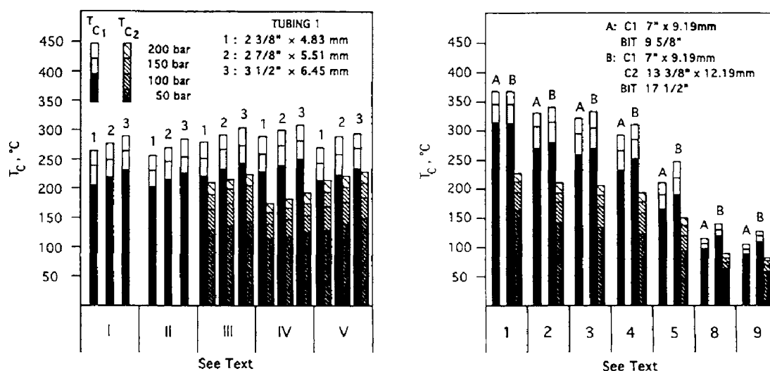
Fig. 4.38: Radial heat flow as a function of completion techniques, Emsland, Northern Germany. (After Goetzen, 1987; courtesy of ITE-TU Clausthal.)
