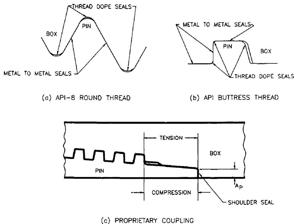
Fig. 1.8: Metal-to-metal seal: (a) API 8-Round thread, (b) API Buttress thread, (c) proprietary coupling. (After Rawlins, 1984.)
