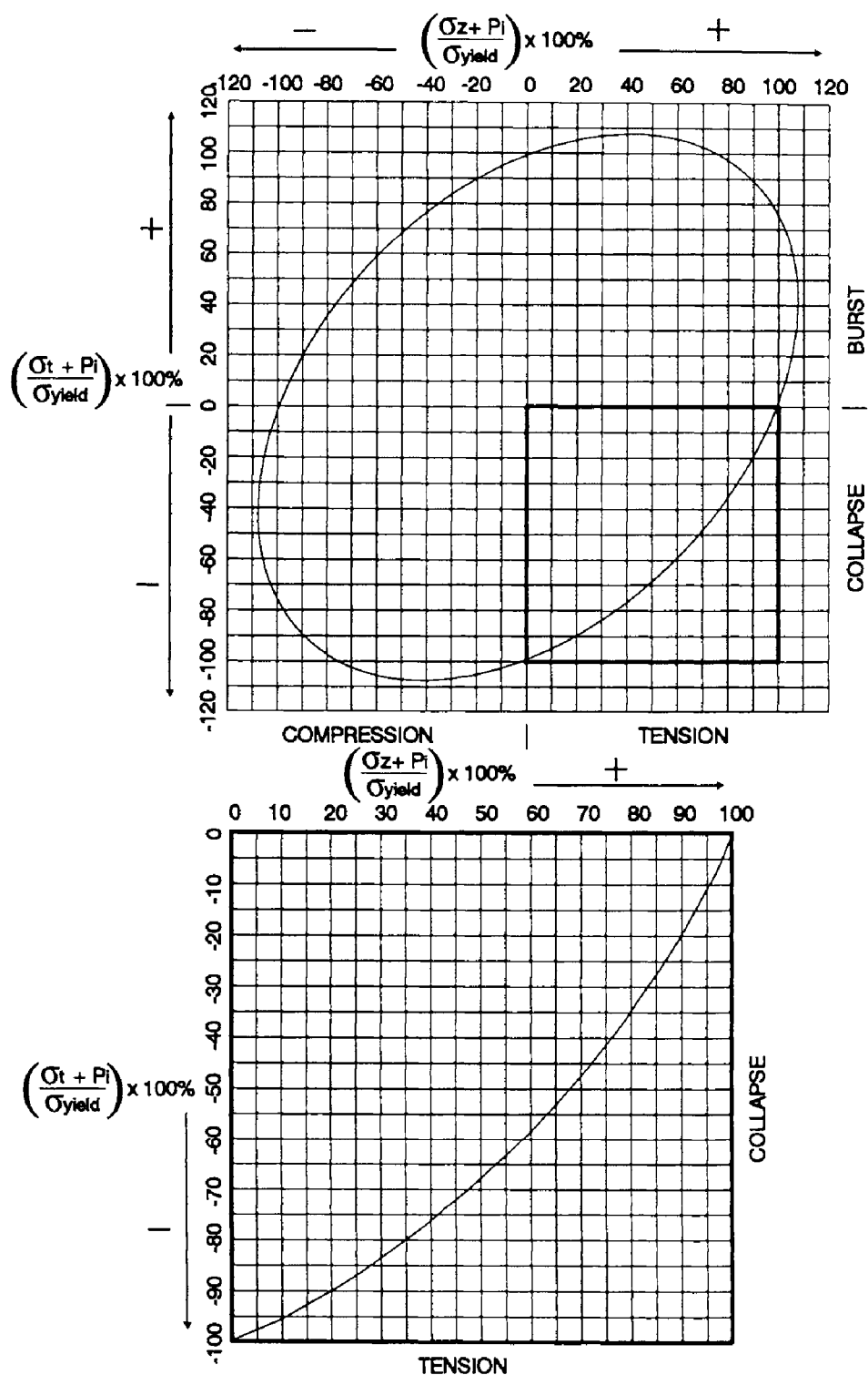
Fig. 2.19: Ellipse of plasticity showing the effect of axial load on both the collapse and burst pressures.
