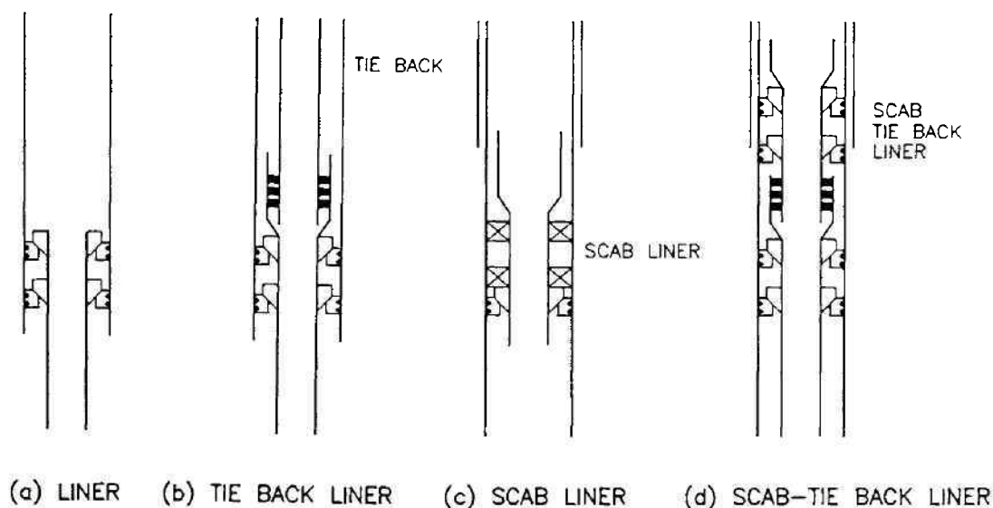
Fig. 1.2: Basic liner system. (After Brown – Hughes Co., 1984.)
