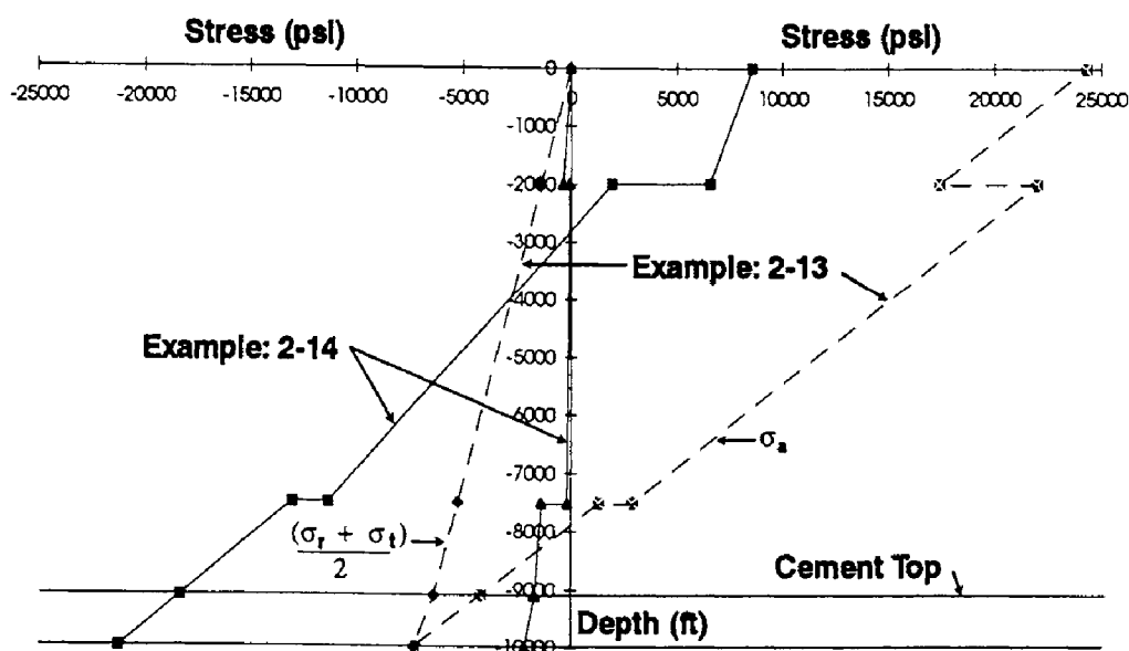
Fig. 2.30: Graphical solution of Examples 2-13 and 2-14.
