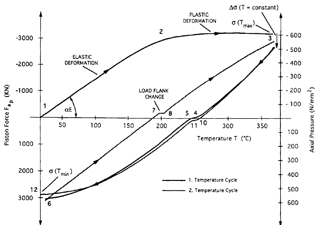
Fig. 4.39: Stress-temperature diagram of API Buttress connection during cyclic heating and cooling. (After Goetzen, 1987; courtesy of ITE-TU Clausthal.)
