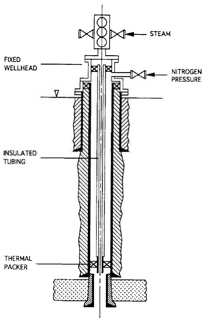
Fig. 4.42: Typical completion of a steam injection well.
