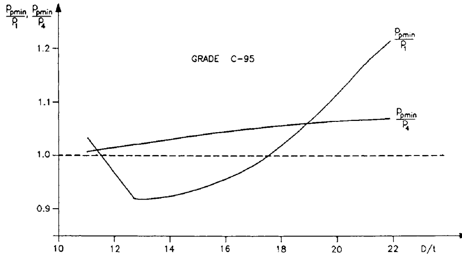
Fig. 2.18: Comparison of experimentally determined minimal collapse strength, p_{pmin} , with that calculated by the methods of API ( P_1 ) and Clineinst ( P_4 ). (After Krug and Marx, 1980; courtesy of ITE-PU Clausthal.)
