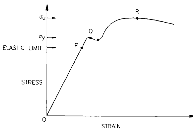
Fig. 2.1: Elastoplastic material behavior with transition range.
