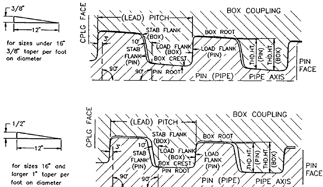
Fig. 1.11: (a) API Buttress thread configuration for 13 \frac{3}{8} in. outside diameter and smaller casing; (b) API Buttress thread configuration for 16 in. outside diameter and larger casing. (After API RP 5B1, 1988.)
