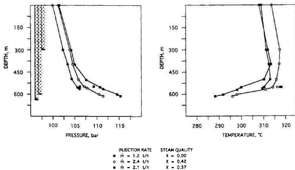
Fig. 4.36: Pressure and temperature distributions in a typical steam injection well Rolermohr steam injection project, Emsland, Northern Germany. (After Goetzen, 1987; courtesy of ITE-TU Clausthal.)
