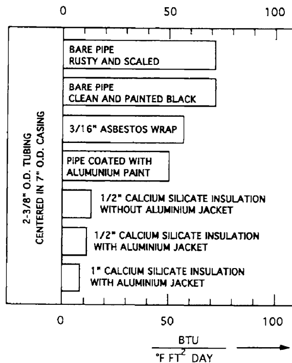
Fig. 4.41: Overall heat transfer coefficient for tubing with different types of insulation. (After Leutwyler, 1966; courtesy J. Petrol. Technol.)
