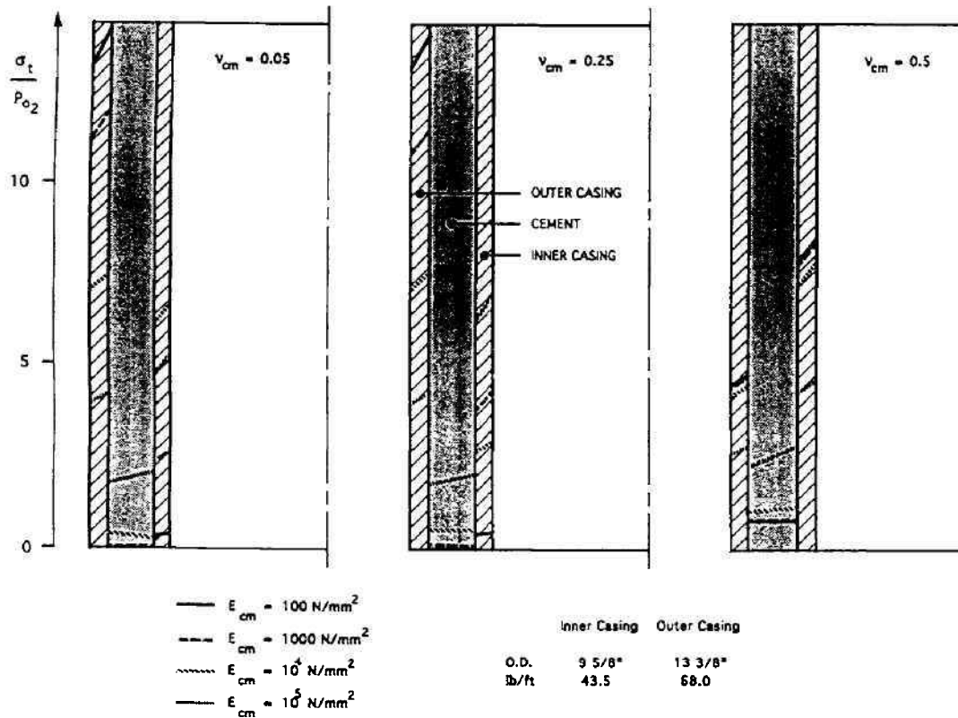
Fig. 4.18: Tangential stress in 13\frac{3}{8} – 9\frac{5}{8} -in. composite casing as a function of modulus of elasticity and Poisson's ratio of cement sheath. (After El-Sayed, 1985; courtesy of ITE-TU Clausthal.)
