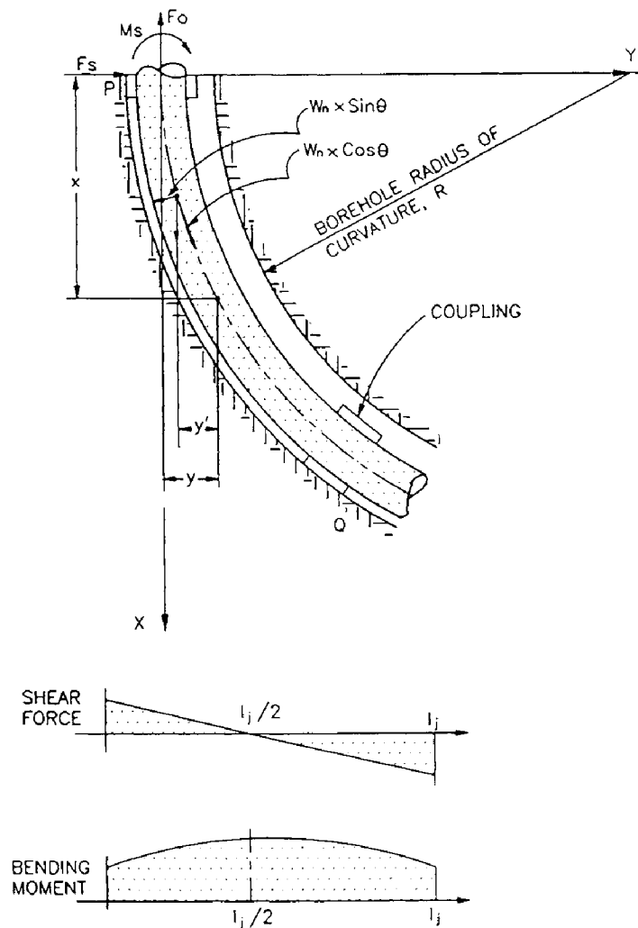
Fig. 2.4: Bending of casing supported at casing collars.
