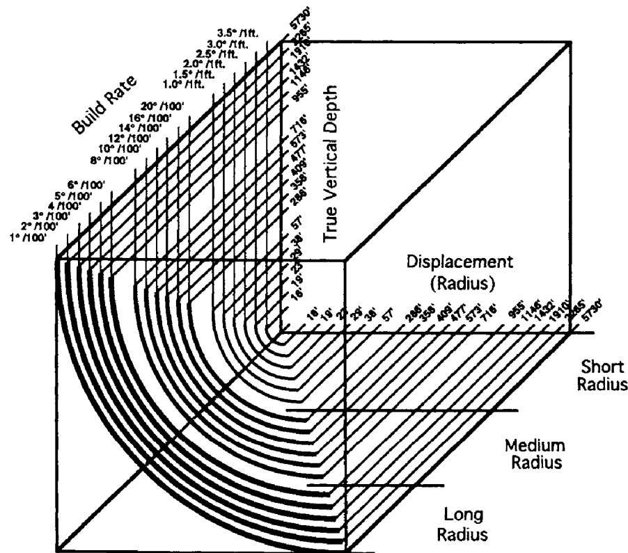
Fig. 4.16: Typical buildup rates for horizontal drainholes. (After Fincher, 1989.)
