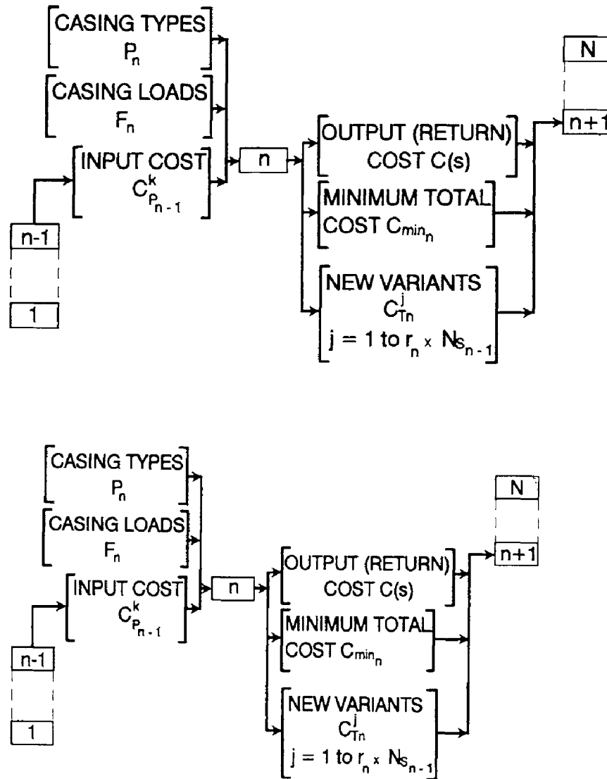
Fig. 5.3: Recurrent calculation procedure for optimum casing design.
