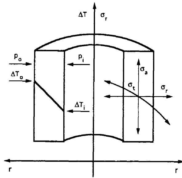
Fig. 4.28: Rotationally symmetric pipe under pressure and temperature.
