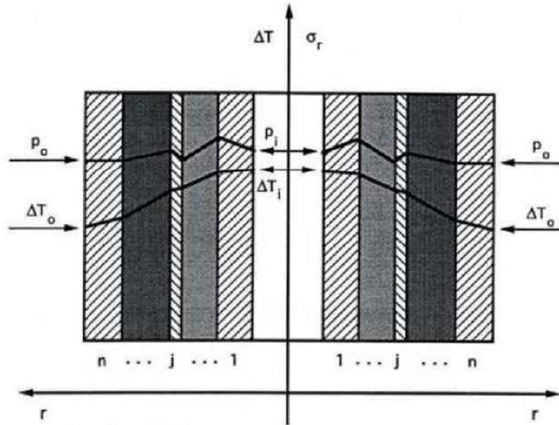
Fig. 4.29: Rotationally symmetric composite pipe under pressure and temperature.
