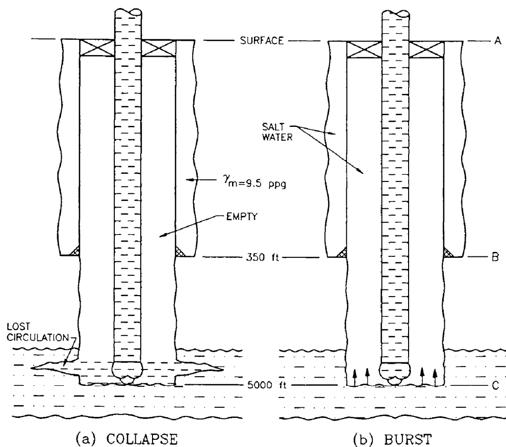
Fig. 3.15: Collapse and burst loads on conductor.
