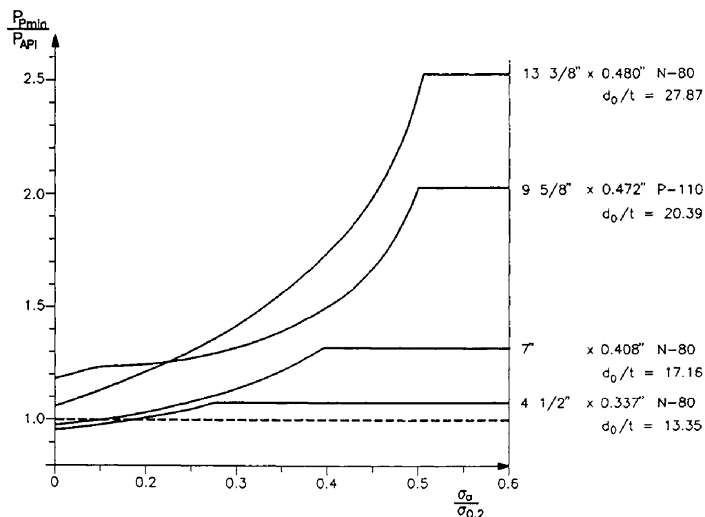
Fig. 2.23: Combined stress due to external pressure and tension: comparison between results obtained using the API Bul. 5C3 (1989) formulas and those of Krug and Marx (1980) and Krug (1982). (Courtesy ITE -PU Clausthal.)
