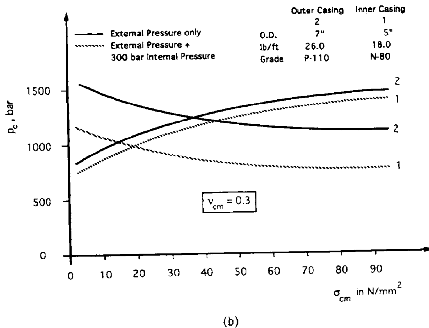
Fig. 4.22: Collapse resistance of the outer and inner pipe as a function of compressive strength of cement; (a) 13 \frac{3}{8} - 9 \frac{5}{8} in. and (b) 7 - 5 in. (After El-Sayed, 1985; courtesy of ITE-TU Clausthal.)
