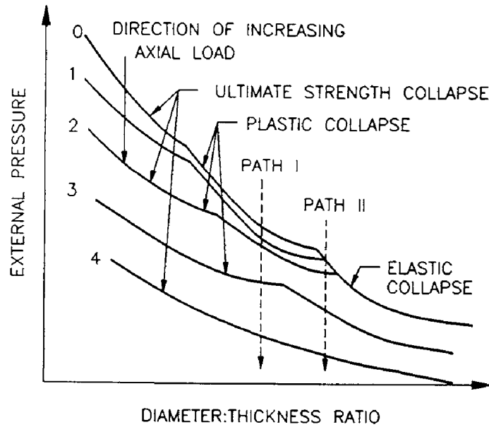
Fig. 2.20: Manifold of collapse curves in the presence of axial load. (After Pattilo and Huang, 1982; courtesy of JPT.)
