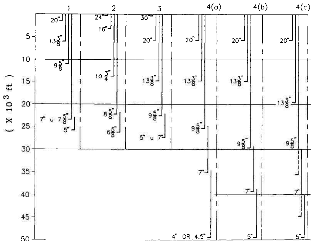
Fig. 3.4: Typical casing program for different depths.
