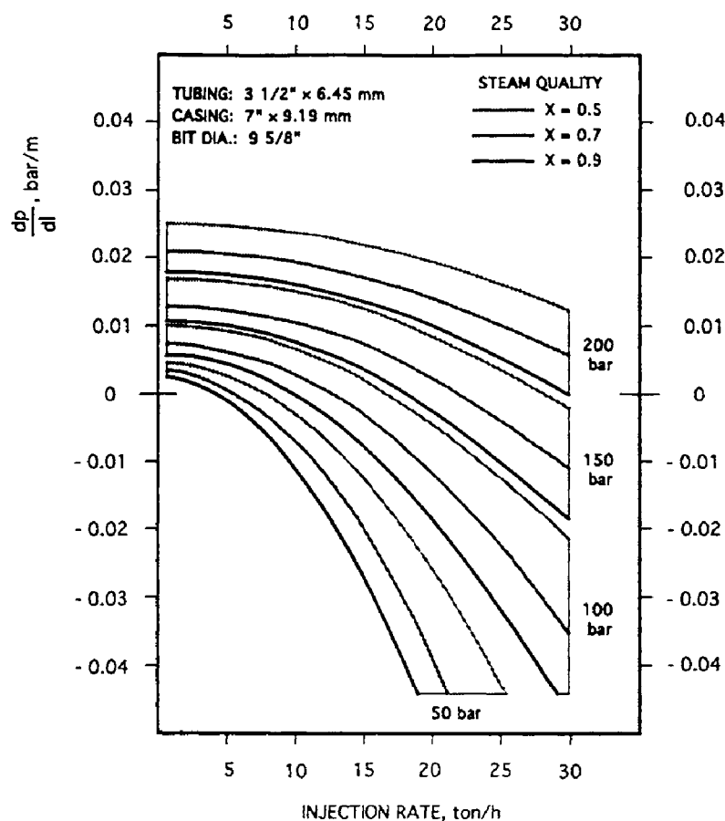
Fig. 4.34: Wet steam pressure gradient as a function of steam pressure, injection rate, and steam quality, Emsland, Northern Germany. (After Goetzen, 1987; courtesy of ITE-TU Clausthal.)
