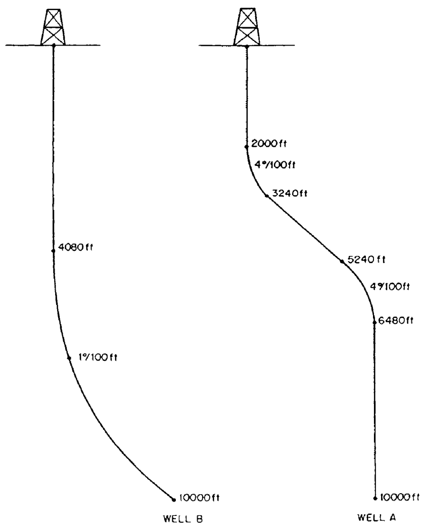
Fig. 5.11: Well trajectories for Example 5-7.
