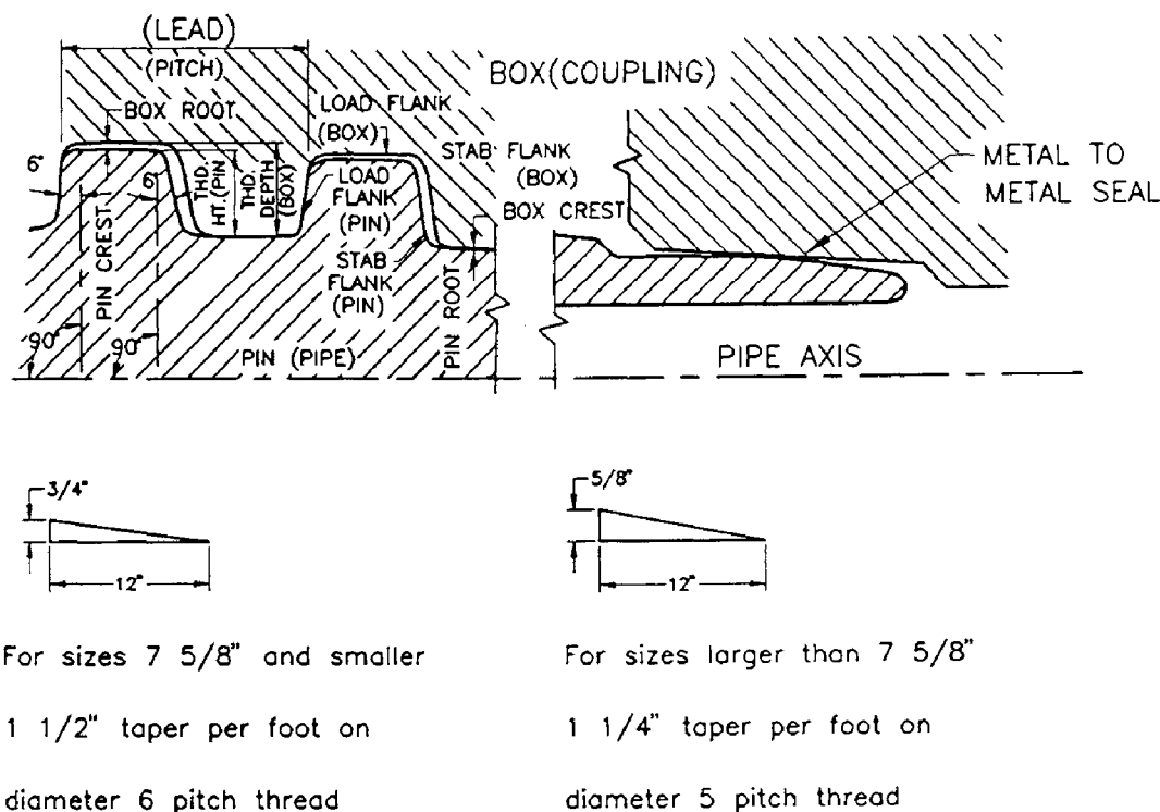
Fig. 1.13: API Extreme-line casing thread configuration. (After API RP 5B1, 1988.)
