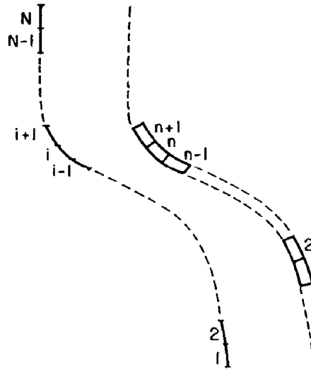
Fig. 5.9: Instantaneous i th position of the n th unit section of casing in a directional well. (After Wojtanowicz and Maidla, 1987; courtesy of SPE.)
