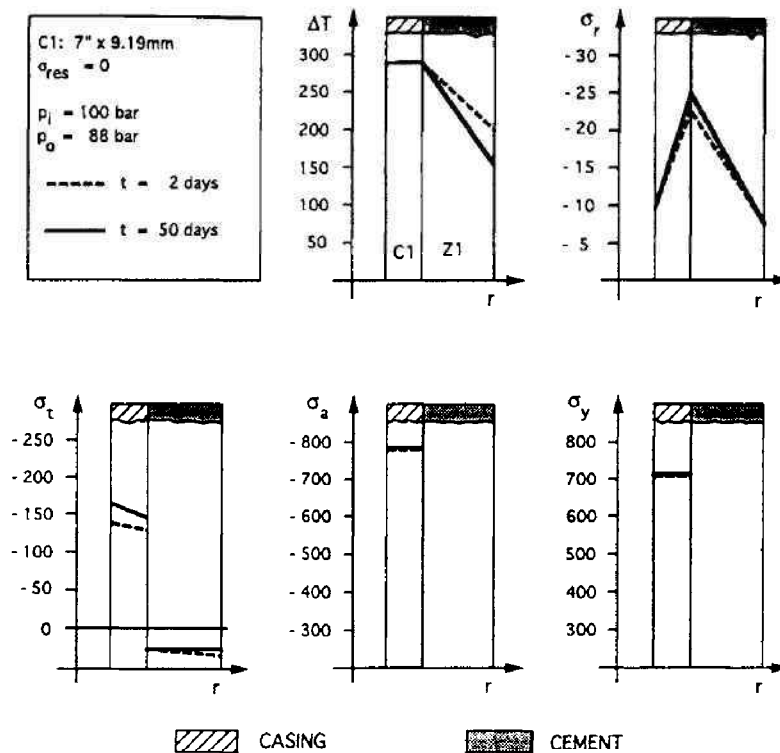
Fig. 4.32: Stress distribution in a single-casing completion and the casing exposed directly to the injected steam ( \Delta T in ^{\circ}\text{C} and \sigma in \text{N/mm}^2 ). (After Goetzen, 1987; courtesy of ITE-TU Clausthal.)
