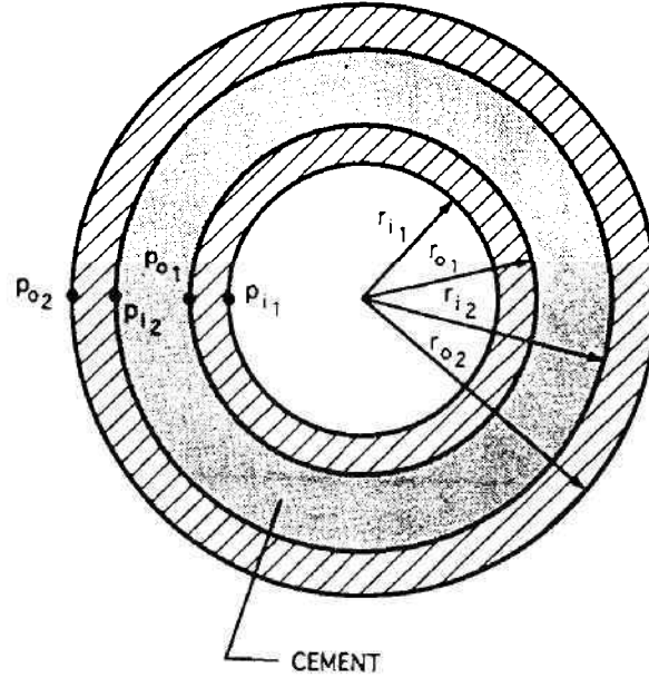
Fig. 4.17: Cross-sectional view of composite casing.
