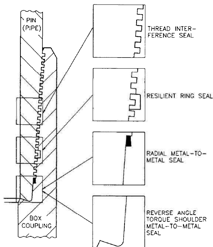
Fig. 1.9: Combination seals. (After Biegler, 1984.)
