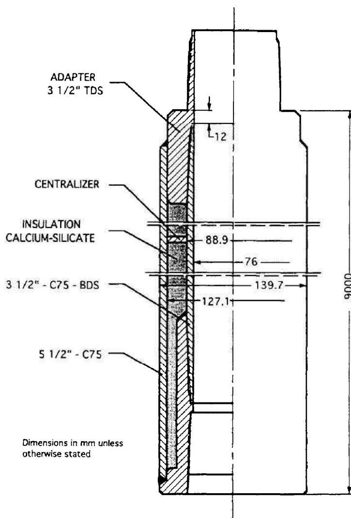
Fig. 4.43: Typical insulated tubing. (After Goetzen, 1987; courtesy of ITE-TU Clausthal.)
