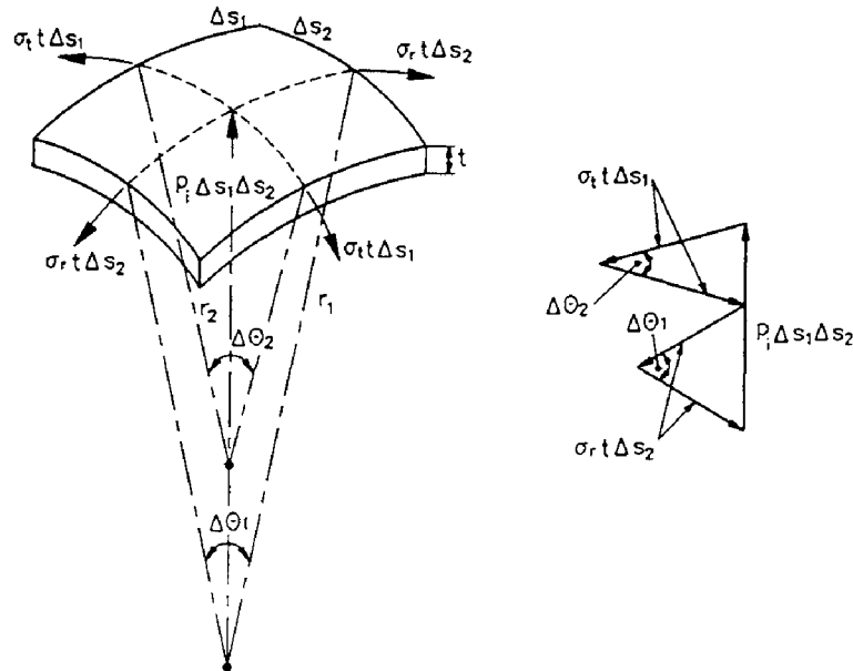
Fig. 2.7: Free body diagram of a rectangular shell element under internal pressure.
