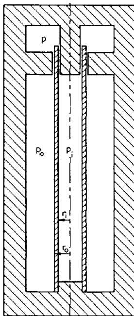
Fig. 2.26: Pipe subjected to three principal forces: internal, external and axial.
