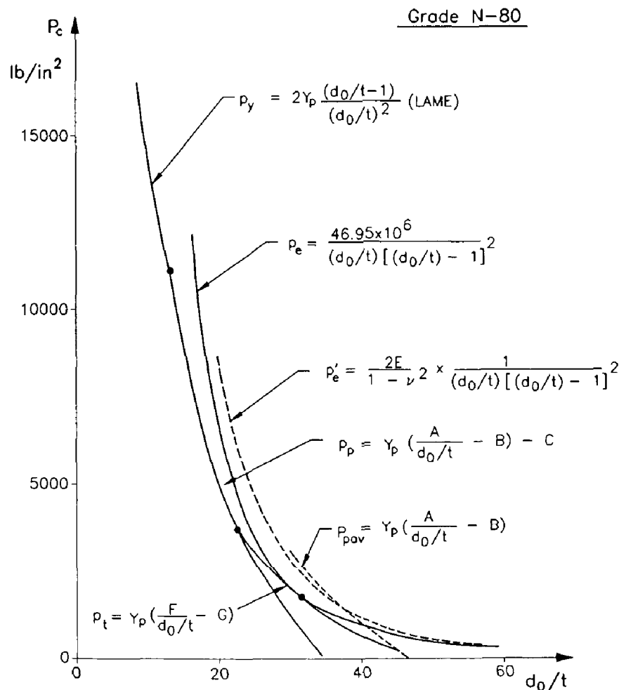
Fig. 2.14: Critical collapse pressure according to API.
