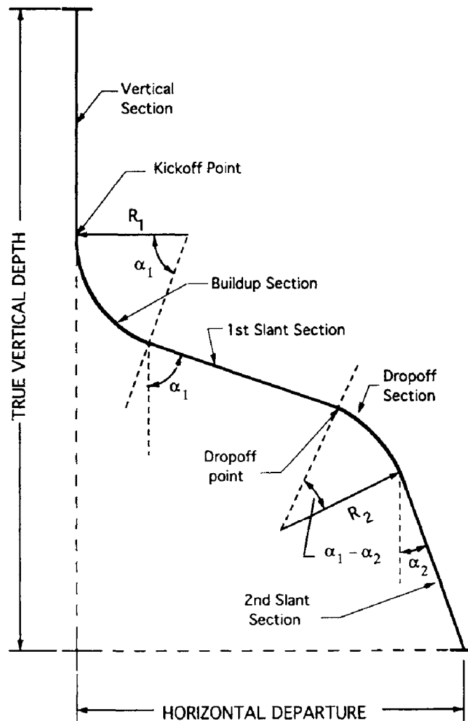
Fig. 4.1: Typical deviated well profile.
