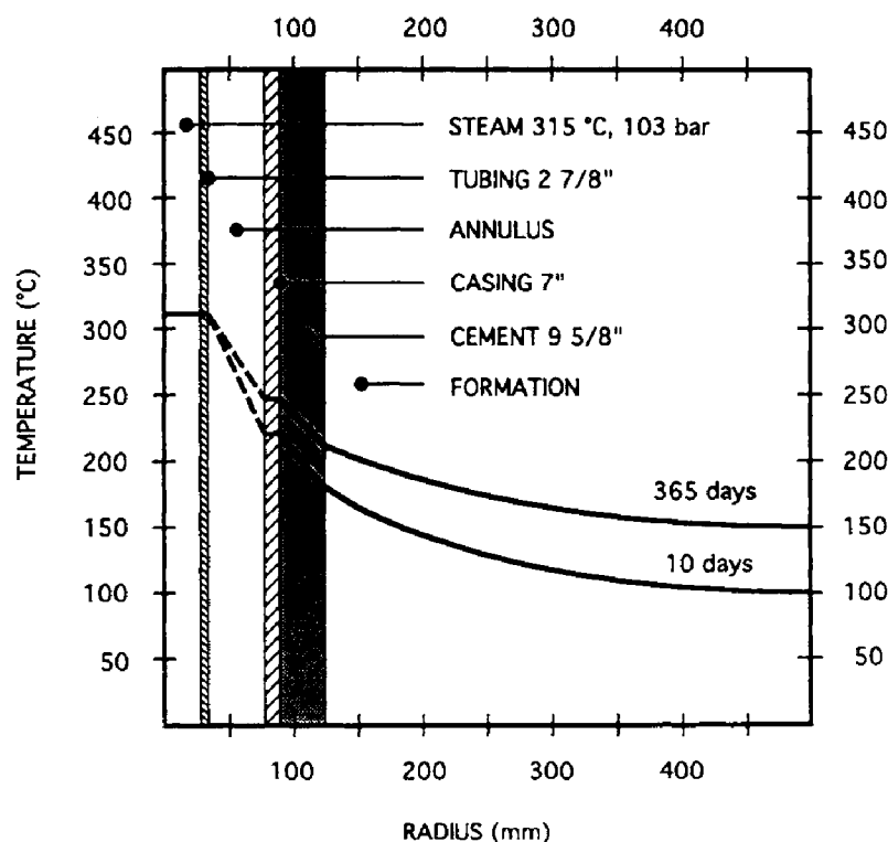
Fig. 4.33: Temperature distribution in a typical steam injection well. (After Sugiura and Farouq Ali, 1978.)
