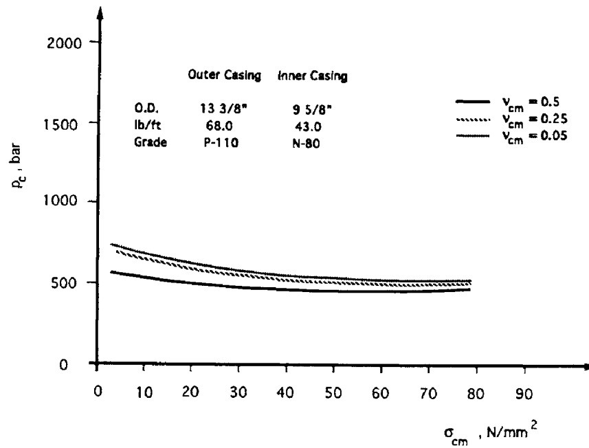
Fig. 4.20: Collapse resistance of the composite pipe as a function of compressive strength and Poisson's ratio of cement. (After El-Sayed, 1985; courtesy of ITE-TU Clausthal.)
