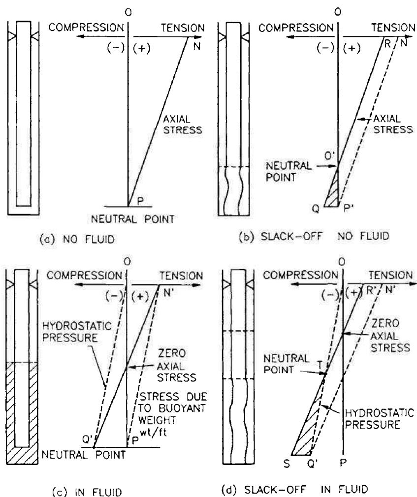
Fig. 2.25: Basic forces acting on casing under different bottom hole conditions. (After Hammerlindl, 1980.)
