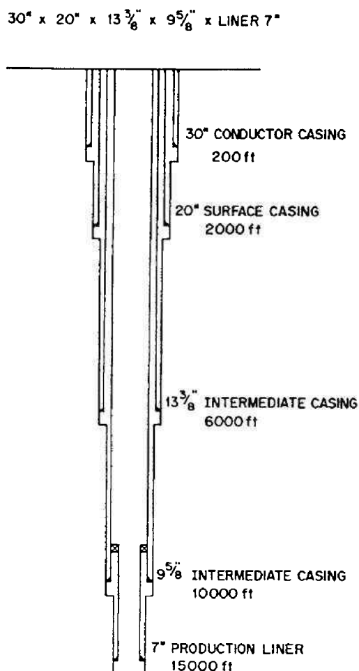
Fig. 5.12: Casing program for Example 5-9.
