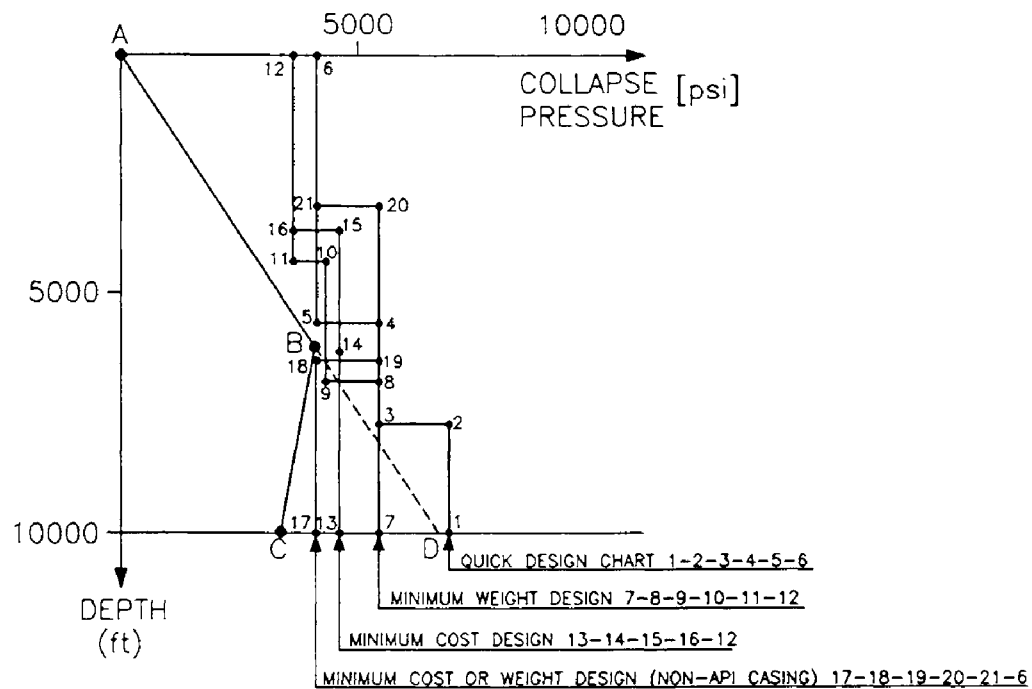
Fig. 5.5: Casing load study for collapse.
