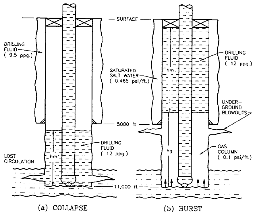
Fig. 3.6: Collapse and burst load on surface casing.
