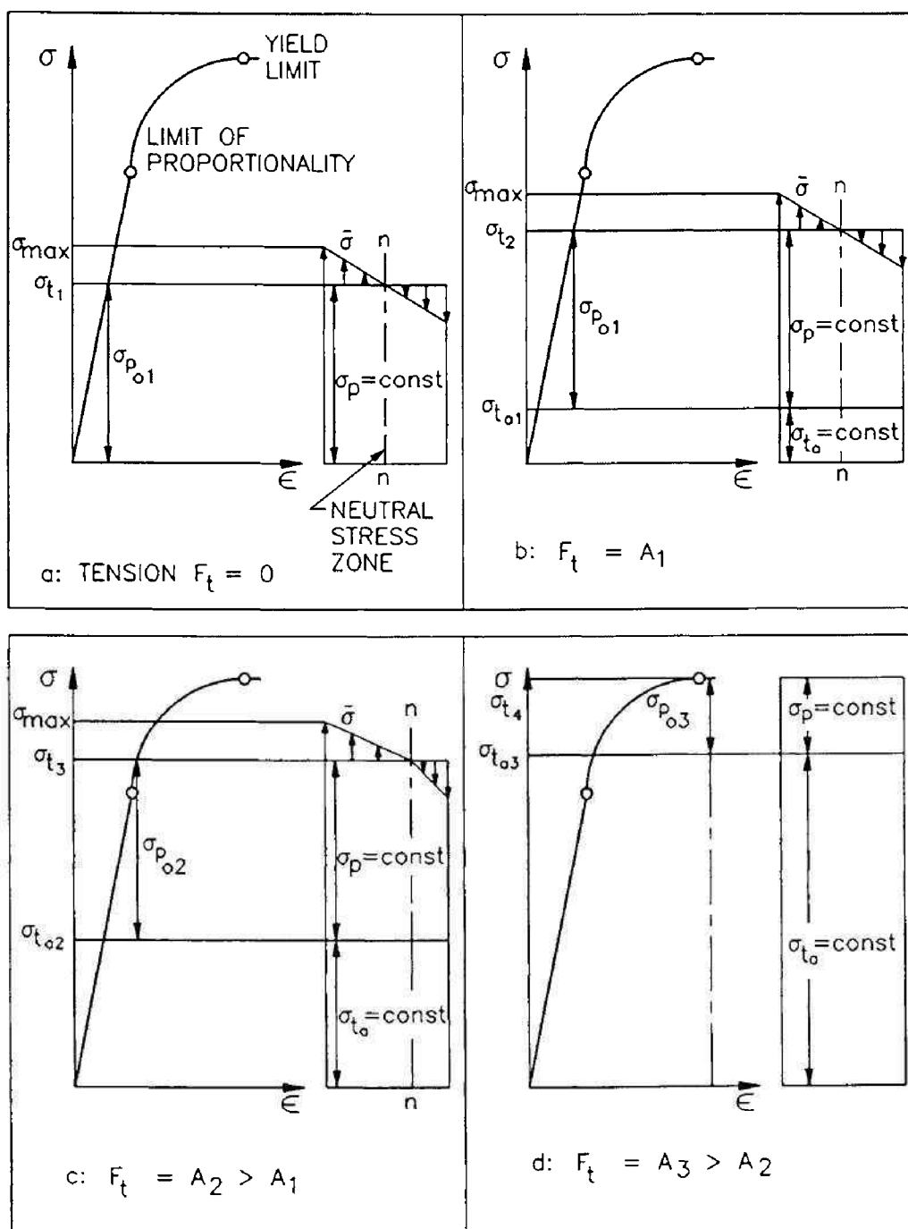
Fig. 2.22: Collapse behavior of casing subjected to external pressure and superimposed tension. Stress-strain plots and assumed distribution of stress over the pipe wall.
