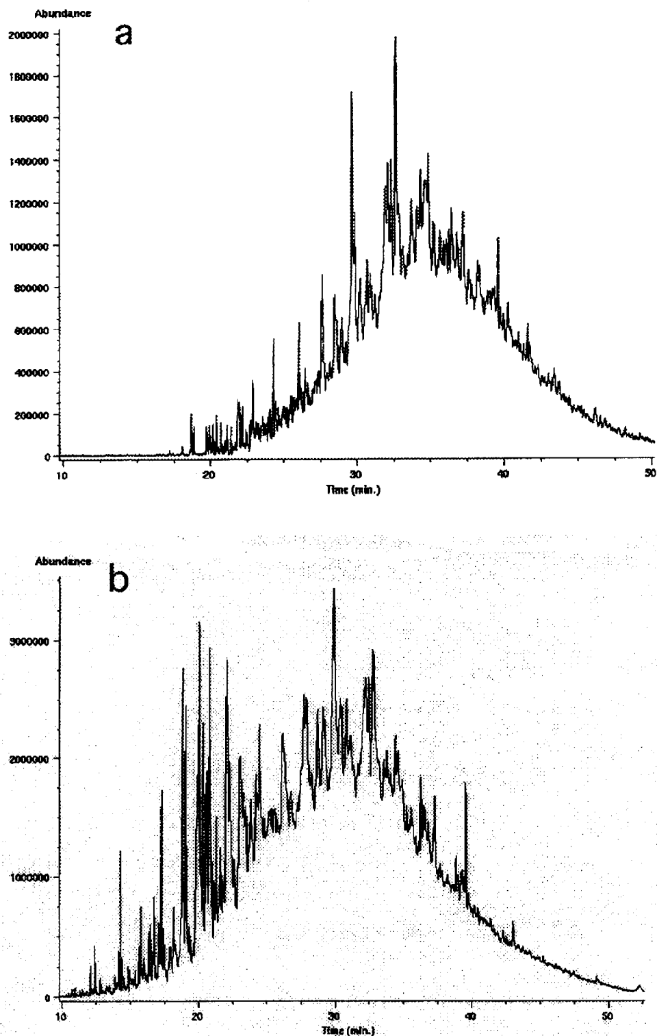
Fig. 4. GC/MS thermogram of the organic compounds present in the aqueous extracts obtained by interactions, at 70°C during 10 days, of Furiel crude oils with HCl (Fig. 4a) and Citric acid (Fig. 4b).
