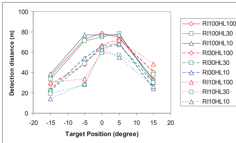
Figure 5.10. Results of detection distance. RI: ambient roadway illuminance (%), HL: headlamp intensity (%) (after Akashi et al., 2003)
