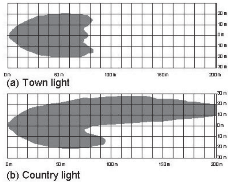
Figure 5.9. Beam patterns of an adaptive forward headlamp system (after Kalze, 2001).
