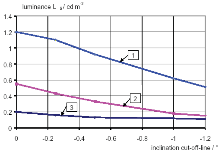
Figure 5.18. Fog luminance distribution as a function of aiming position, for a visibility distance of 50 m (after Rosenhahn, 2001).
