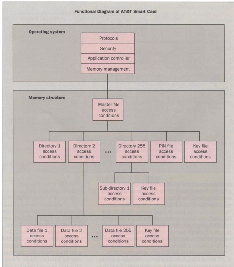
Figure 2. The AT&T Smart Card has an operating system that implements a hierarchical file system. The physical separation of files is possible using different branches of the hierarchy. Access permissions, such as read, write, and execute, can be assigned on a per-file or per-directory basis. The hierarchical structure permits a card provider to offer various levels of access and functionality, as well as permitting multiple applications providers to offer a variety of services—all on a single card.
