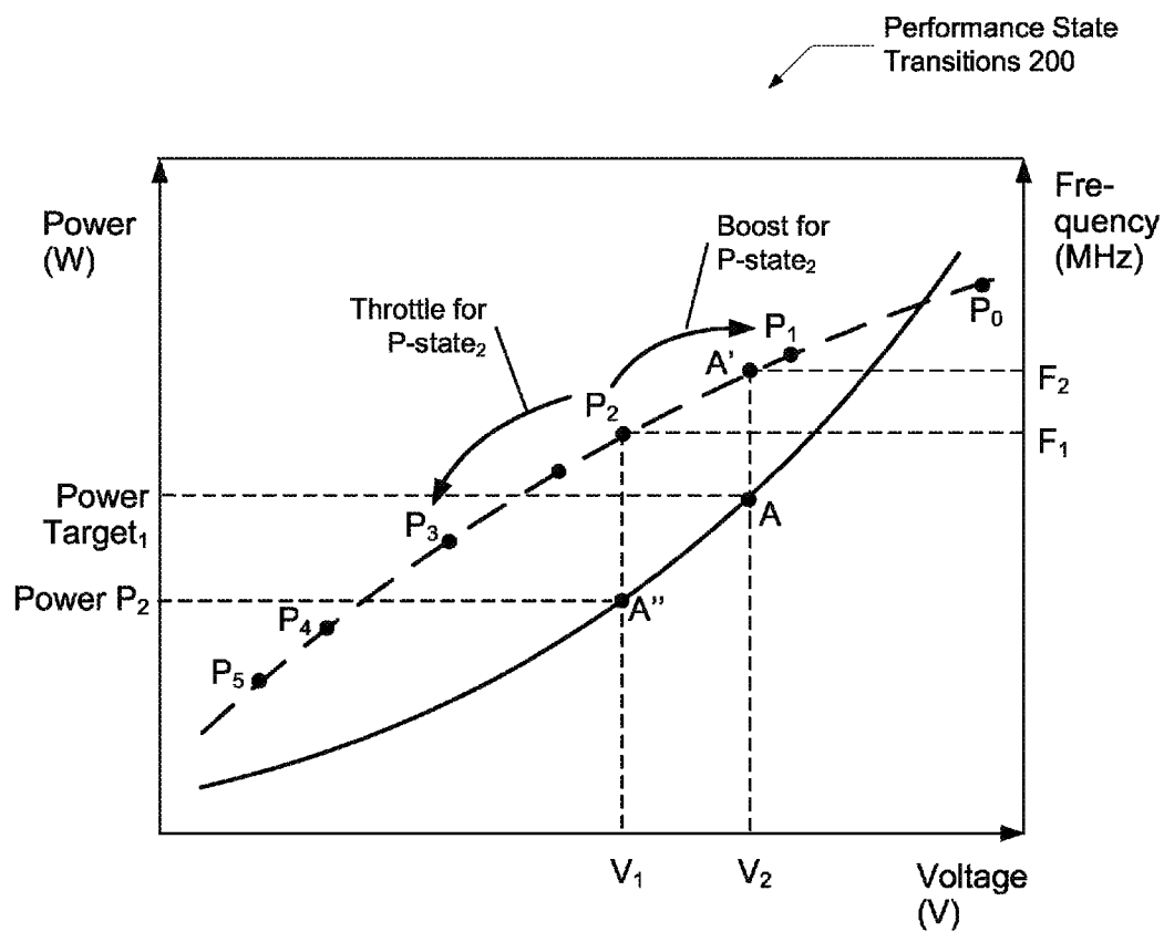
Sample P-State Table 210
