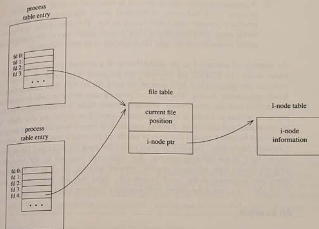
Figure 6.13 Sharing a file table entry between two processes.
