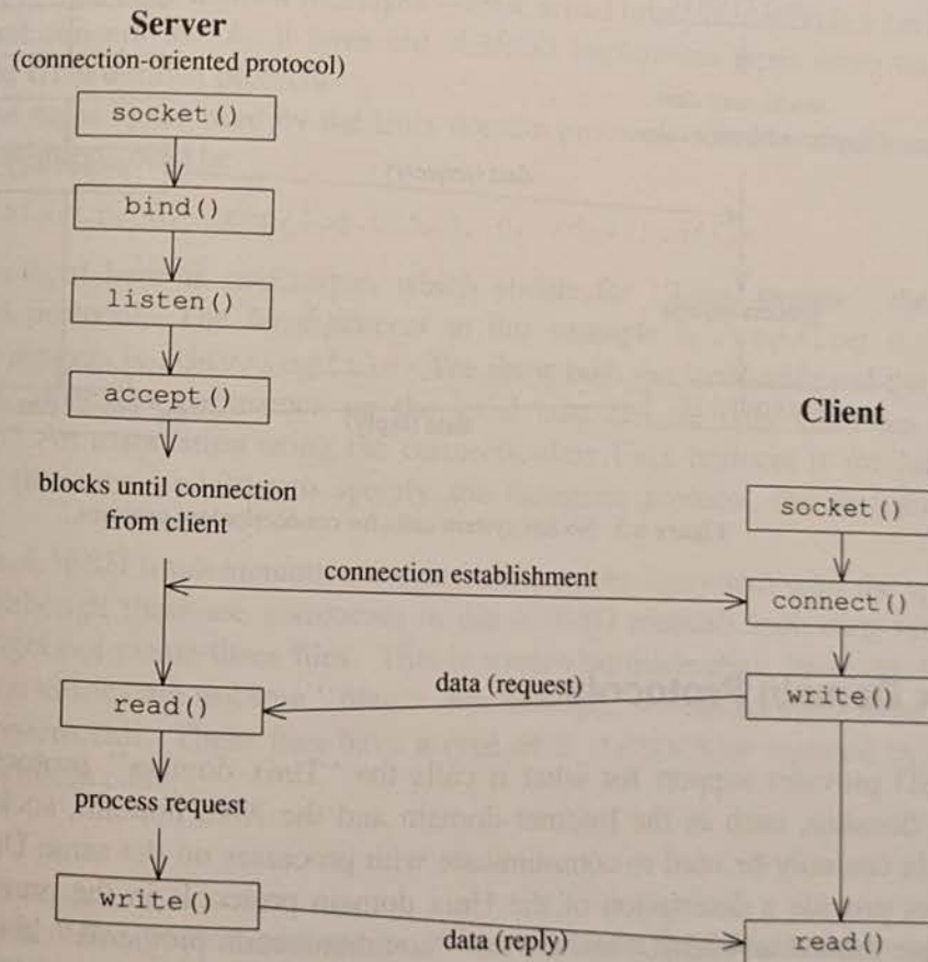
Figure 6.2 Socket system calls for connection-oriented protocol.
