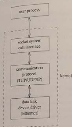
Figure 6.19 Networking implementation in 4.3BSD.
