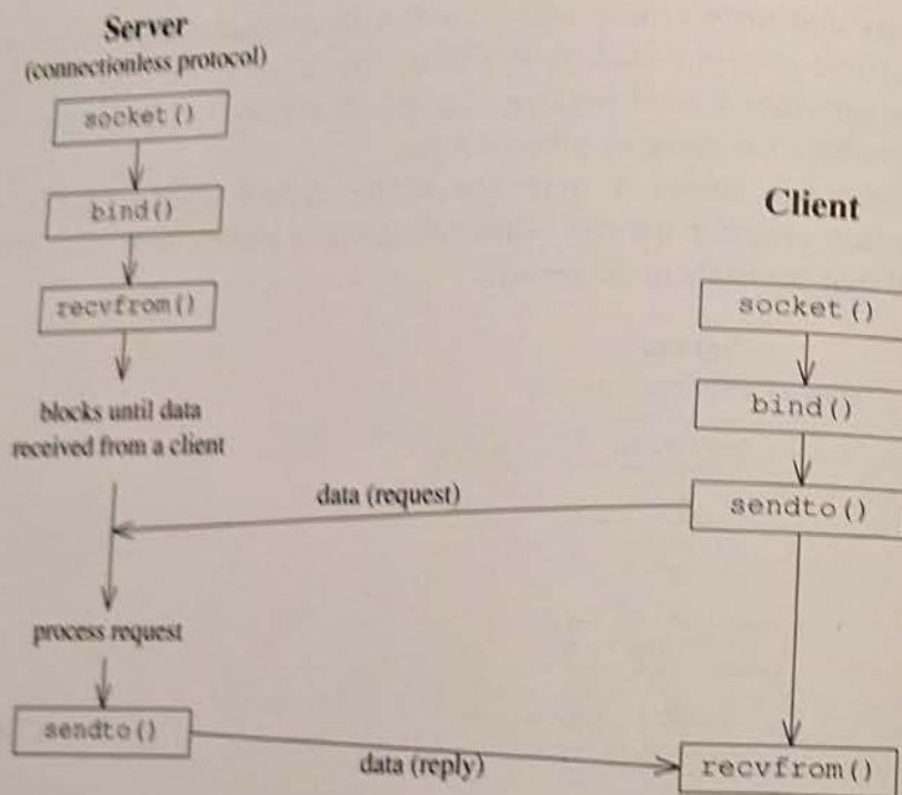
Figure 6.3 Socket system calls for connectionless protocol.
