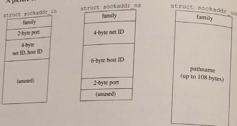
Figure 6.5 Socket address structures for Internet, XNS and Unix families.
