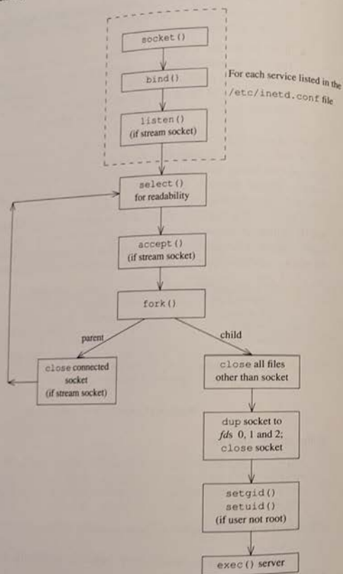
Figure 6.18 Steps performed by inetd.
