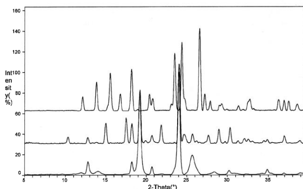
Figure 2. PXRD patterns for forms I (top), II (middle), and III (bottom) of acetaminophen.
