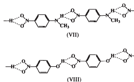
Fig. 2. Isographic hydrogen-bond patterns of a secondary aniline and a phenol. Both sets of molecules have the same first- and second-order graph sets: N_1 = R_1^2(4) and N_2 = C_1^2(8) .
