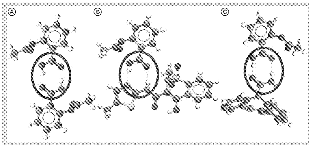
Figure 2. Synthon examples in pharmaceutical cocrystals involving carboxylic acids and amides. (A) The carboxylic acid-carboxylic acid supramolecular homosynthon as seen in aspirin. (B) The carboxylic acid-weakly basic nitrogen atom supramolecular heterosynthon as exemplified by the aspirin: meloxicam cocrystal. (C) The carboxylic acid-amide supramolecular heterosynthon observed in the cocrystals of aspirin and carbamazepine. The blue ovals highlight each supramolecular synthon.
