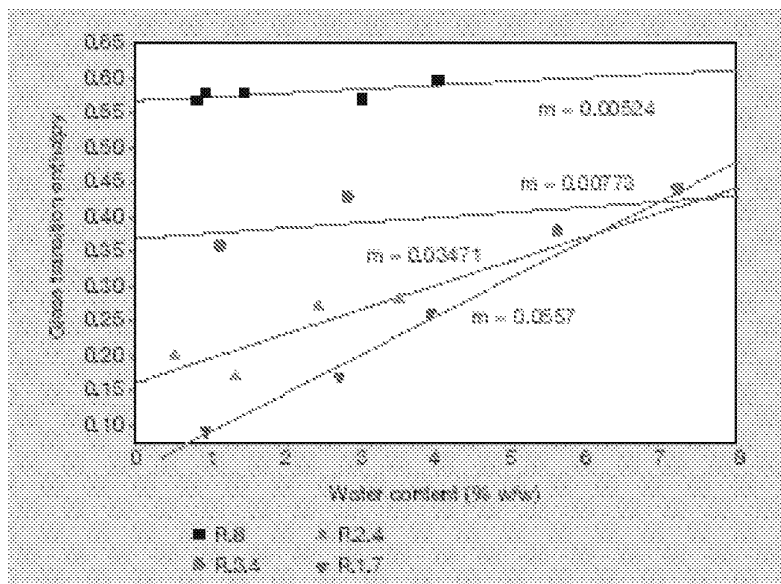
Figure 1: Effect of water content on glass-transition enthalpy. Plot of enthalpy versus water content for four formulations having various sugar/lipid ratios ( R ).
