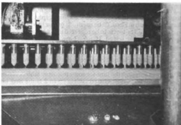
Fig 40. Manufacture of hard gelatin capsules by dipping stainless-steel pins into gelatin solutions (courtesy, Lilly).
