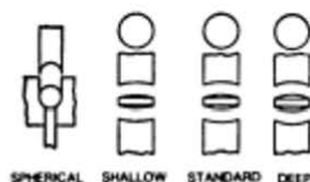
Fig 17. Concave punches.
