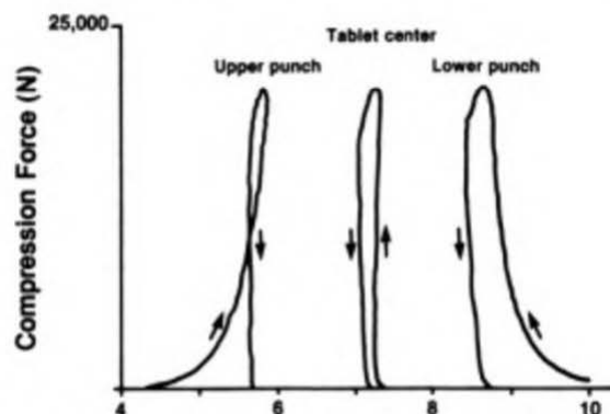
Fig 30. Plot showing the upper and lower punch forces as functions of the position of the punch face within the die. A biaxial force/displacement curve also shown is a plot of the position of the tablet center as a function of the compression force.
