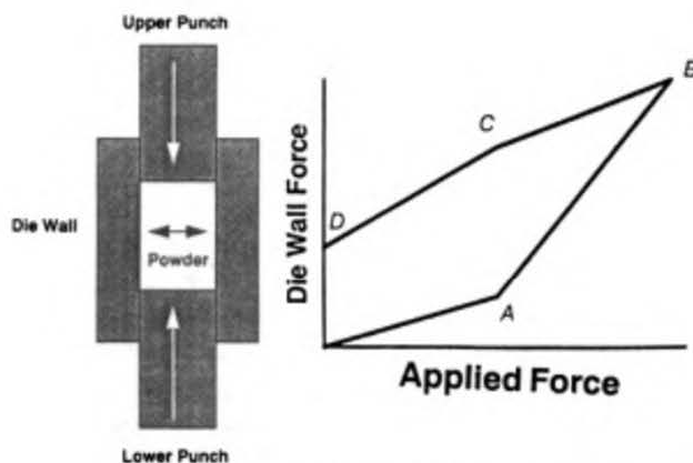
Fig 6. Transmitted stresses during tablet compaction.
