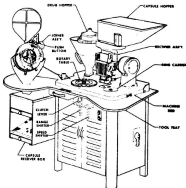
Fig 44. Schematic of Type 8 capsule-filling machine (courtesy, Parke-Davis).
