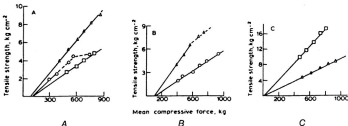
Fig 4. Tensile strength of compacts prepared from different crystal forms. A: Barbitone (104–152 μm)—○, Form I; □, Form II; △, Form III. B: Sulphathiazole (104–152 μm)—○, Form I; △, Form II. C: Aspirin (250–353 μm)—△, Form I; □, Form IV (courtesy, Summers et al 27 ).
