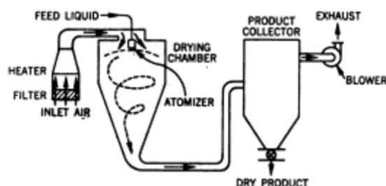
Fig 16. Typical spray-drying system (courtesy, Bowen Eng).
