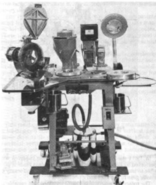
Fig 45. Type 8 capsule-filling machine (courtesy, Lilly).
