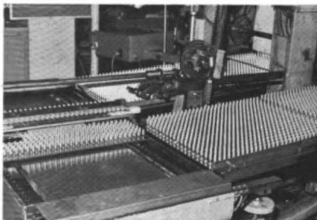
Fig 41. Formed capsules being dried by rotating through a drying kiln (courtesy, Lilly).
