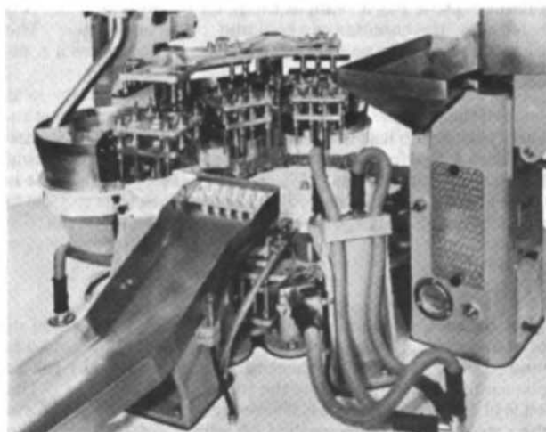
Fig 47. Zanasi automatic filling machine, Model AZ-60. The set of filling heads shown at the left collects the powder from the hopper, compresses it into a soft slug and inserts it into the bottom half of the capsule (courtesy, United Machinery).
