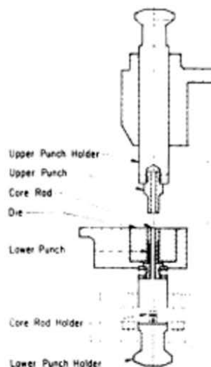
Fig 52. Core-rod tooling for compressing troches or candy pieces with hole in center (courtesy, Vector/Colton).
