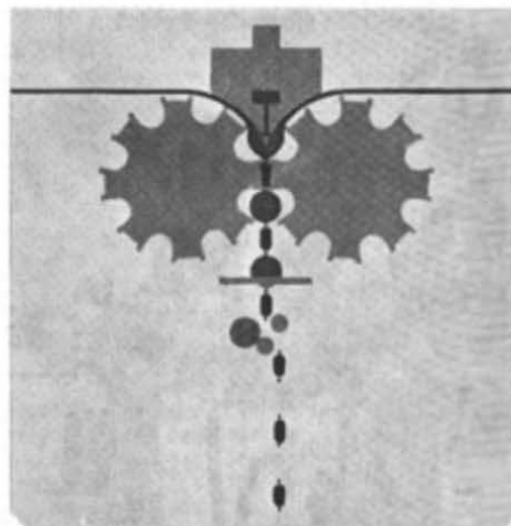
Fig 49. Rotary-die elastic capsule filler.
