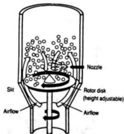
Fig 12. Three versions of fluidized-bed granulation and drying. A: Top-spray method used in conventional fluid-bed granulation coaters; B: bottom-spray method used in Wurster air-suspension columns; C: tangential-spray method used in rotary fluid-bed coaters/granulators (courtesy, Aster Publ, adapted from Ref 31).
