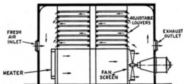
Fig 11. Cross section of tray dryer.
