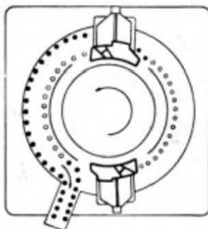
Fig 26. The movement of tablets on die table of a double rotary press (courtesy, Vector/Colton).
