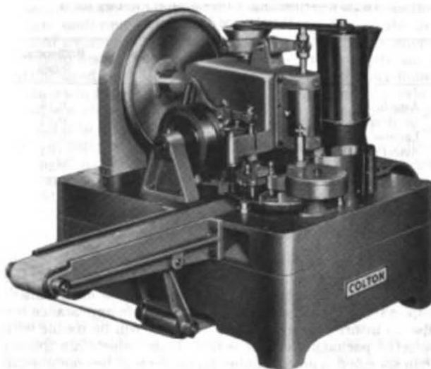
Fig 35. Automatic tablet triturate machine (courtesy, Vector-Colton).
