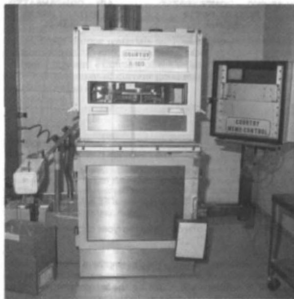
Fig 27. Courtney R-100 with computer-controlled operation.
