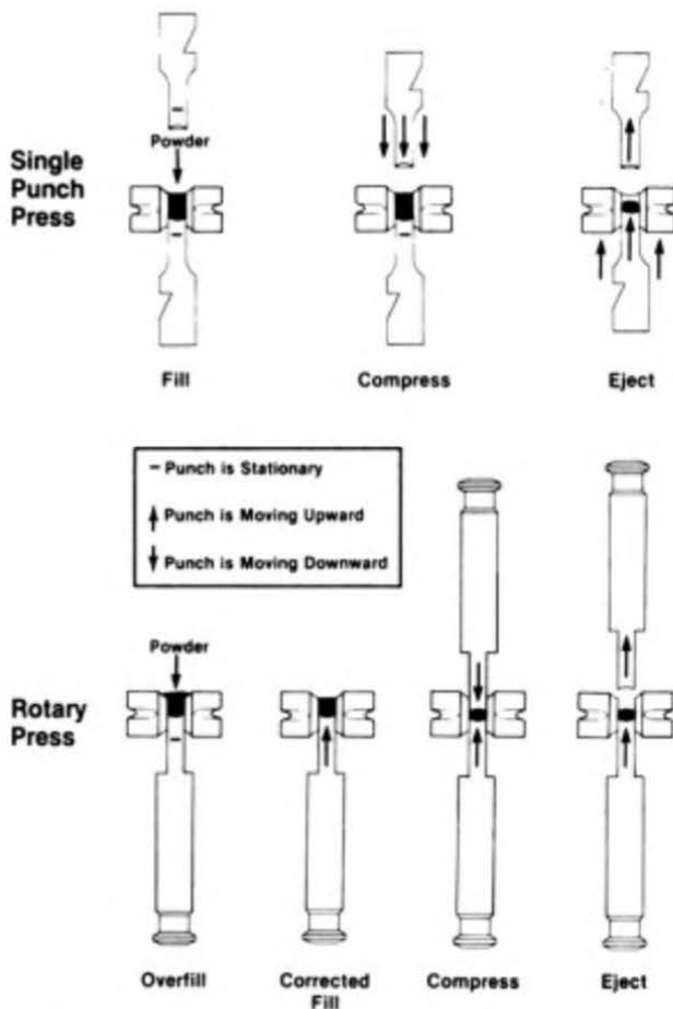
Fig 21. The steps associated with single-punch and rotary tablet machines.
