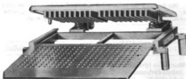
Fig 34. Tablet triturate mold (courtesy, Vector/Colton).
