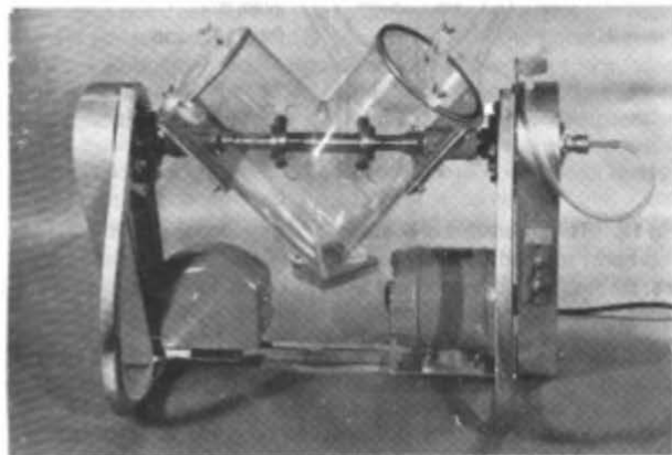
Fig 8. Twin-shell blender for solids or liquid-solids blending (courtesy, Patterson-Kelley).
