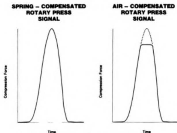
Fig 29. Force-time curves for two types of tablet press.
