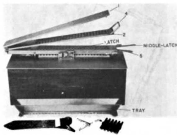
Fig 42. Hand-operated capsule machine (courtesy, Chemi-Pharm).
