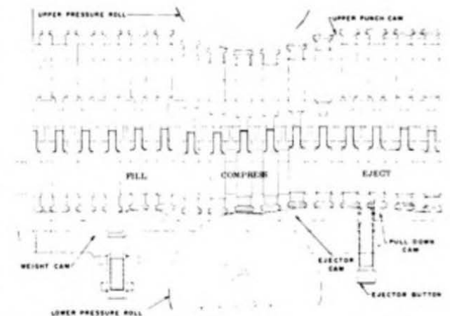
Fig 23. Tooling for a 16-station rotary press showing positions of the cycle required to produce 1 tablet per set of tooling (courtesy, Vector/Colton).
