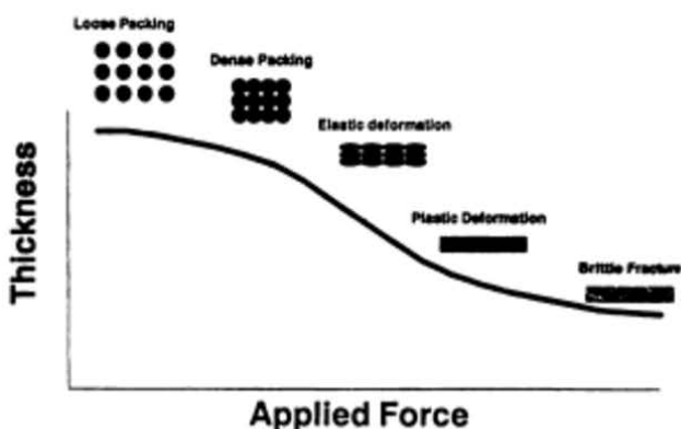
Fig 3. The stages of powder compaction.
