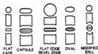
Fig 18. Specially shaped punches.
