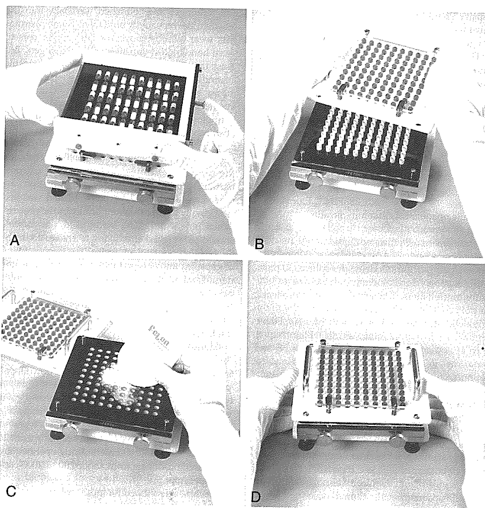
Fig. 7.9 The Feton capsule filling machine. A, with empty capsules in the loader tray, the tray placed on top of the filler unit; B, the loader inserts the capsules into the filling unit and is removed and the top plate is lifted to separate the caps from the bodies; C, the powder is placed on the unit and the capsule bodies filled; D, the top plate then is returned to the unit and the caps placed on filled capsule bodies. (Courtesy of Chemical and Pharmaceutical Industry Company)
