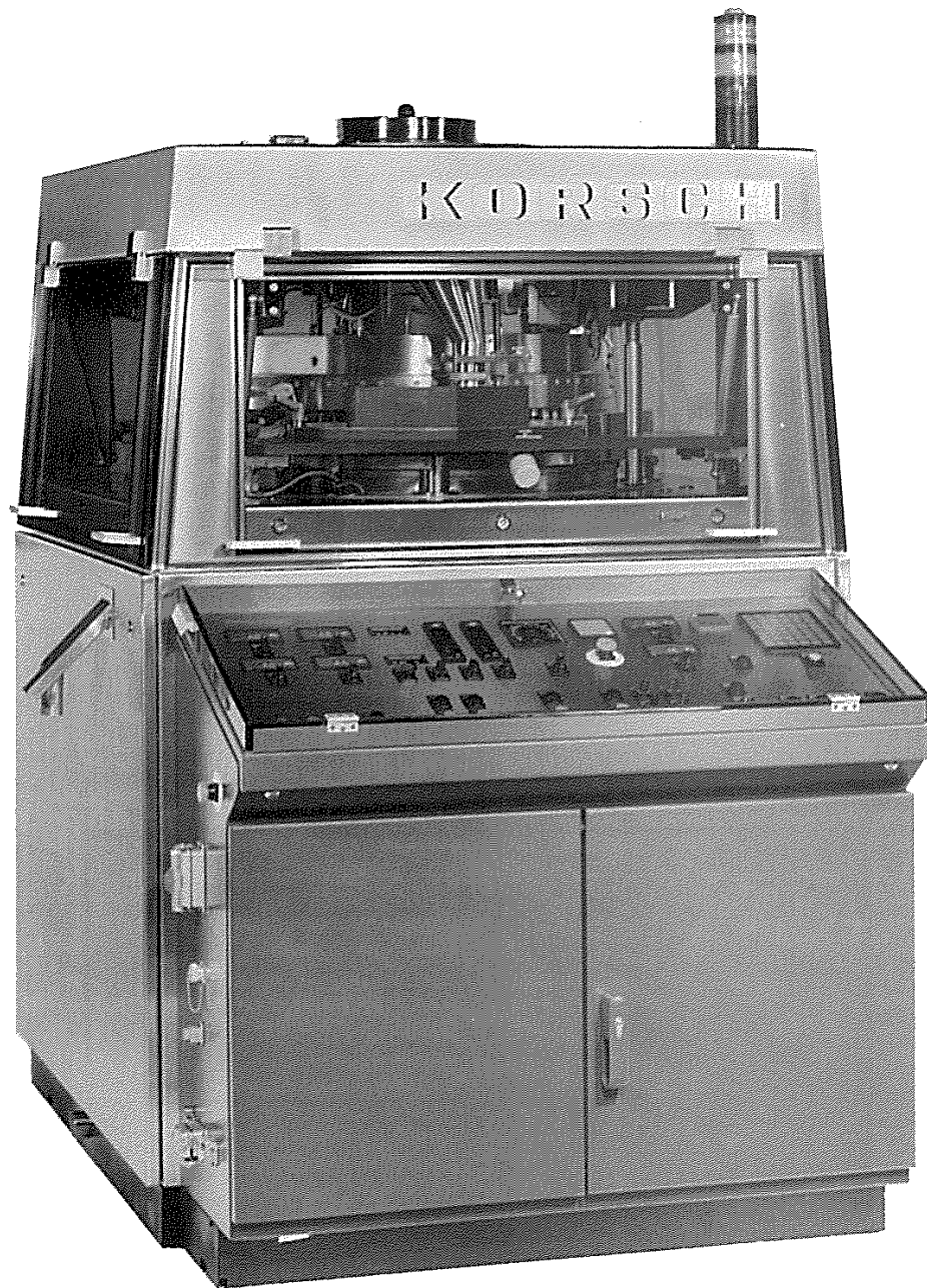
Fig. 7.22 Example of a high-performance double rotary tablet press. The Korsch PharmapressR has a maximum output of 1 million tablets per hour but for continuous operation it is generally run to produce 600,000 to 800,000 tablets per hour. (Courtesy of Korsch Tableting, Inc.)
