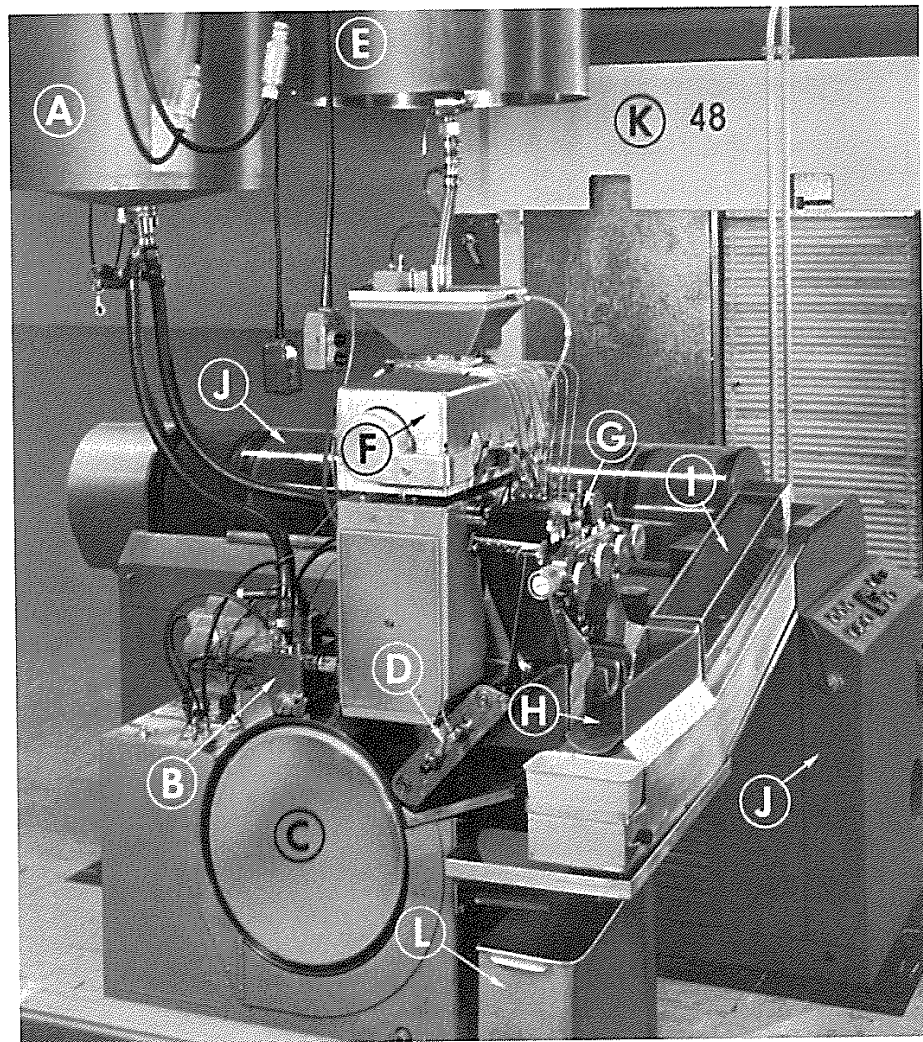
Fig. 7.15 Rotary die process equipment. A, Gelatin tank; B, spreader box; C, gelatin ribbon casting drum; D, mineral oil lubricant bath; E, medicine tank; F, filling pump; G, encapsulating mechanism; H, capsule conveyor; I, capsule washer; J, infrared dryer; K, capsule drying tunnel; L, gelatin net receiver. (Courtesy of R.P. Scherer Corporation.)
