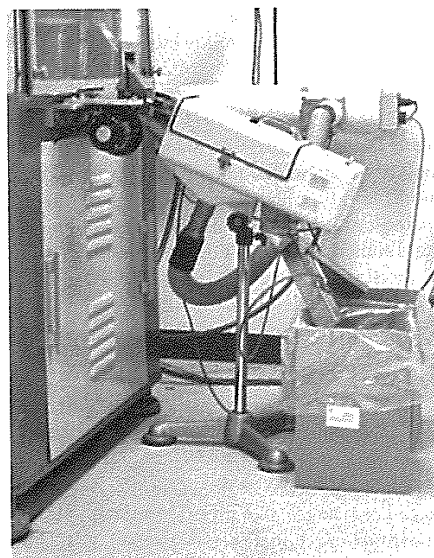
Fig. 7.47 Model 25 Manesty Tablet Deduster. Tablets leaving tableting machine are dedusted and passed into collection containers. (Courtesy of Eli Lilly and Company.)
