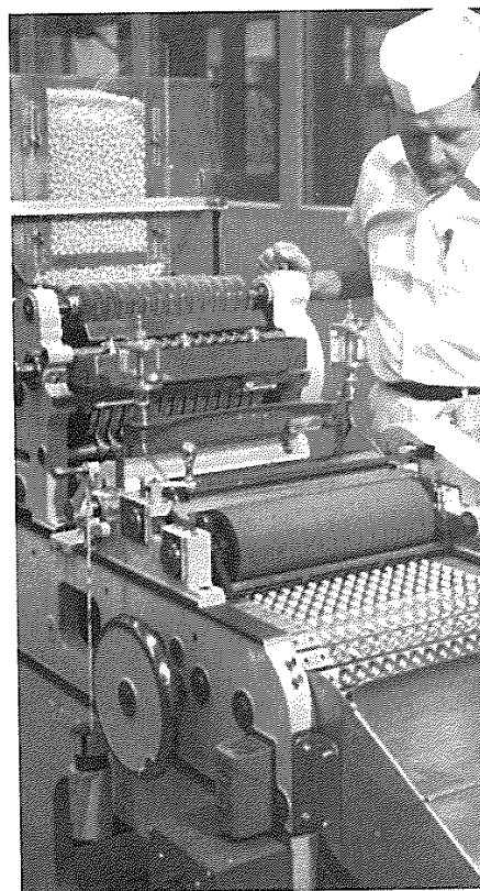
Fig. 7.52 Branding of coated compression tablets on a Hartnett branding machine. (Courtesy of The Upjohn Company.)
