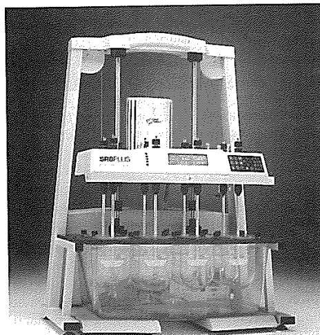
Fig. 7.35 Hanson SR8-Plus Dissolution Test System. Features microprocessor and templates to create, edit, store, and validate dissolution protocols, graphical displays with menus and icon-based program controls. (Courtesy of Hanson Research Corporation).
