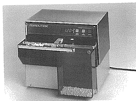
Fig. 7.32 CompuTest hardness tester, tests in Newtons, Kilopond, and Strong Cobb. Automatic or manually operated. tests up to 100 tablets per run. Integrated software stores product test programs. (Courtesy of Vector Corporation.)
