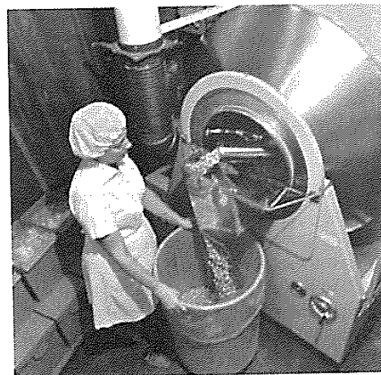
Fig. 7.14 Cleaning and polishing hard filled capsules using the Accela-Cota apparatus. (Courtesy of Eli Lilly and Company.)
