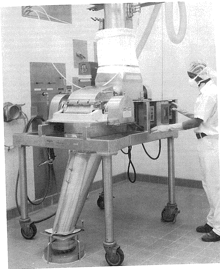
Fig. 7.42 Frewitt Oscillator or Fitz Mill utilized in the pulverization or granulation process. (Courtesy of Eli Lilly and Company.)
