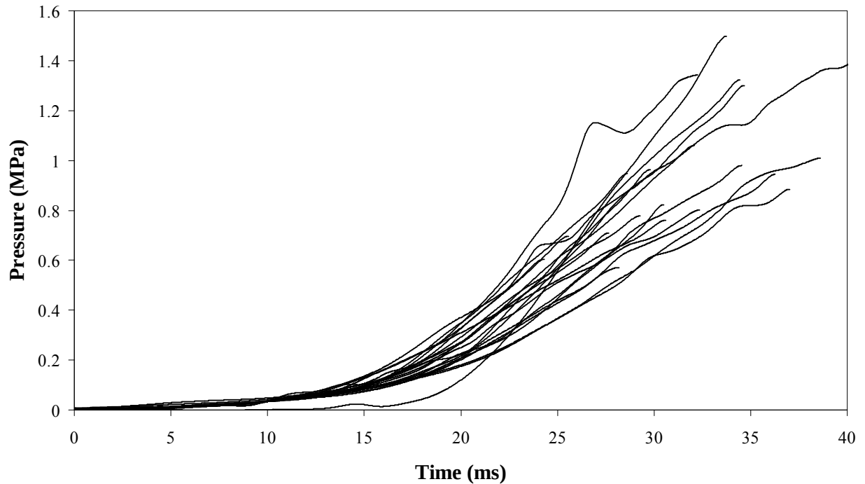
Figure 3: Rupture pressure with respect to time for 20 human eyes.
