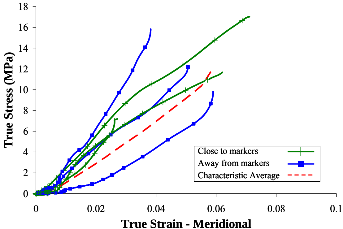
Figure 10: Stress and strain comparison for tests with rupture close to and away from optical markers in the meridional direction.
