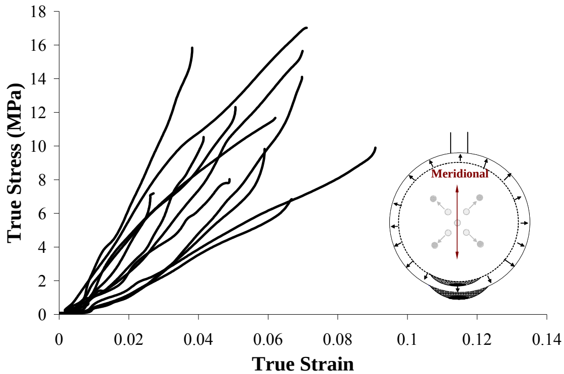
Figure 8: Stress-strain curve response in the meridional direction of 12 eye rupture tests.
