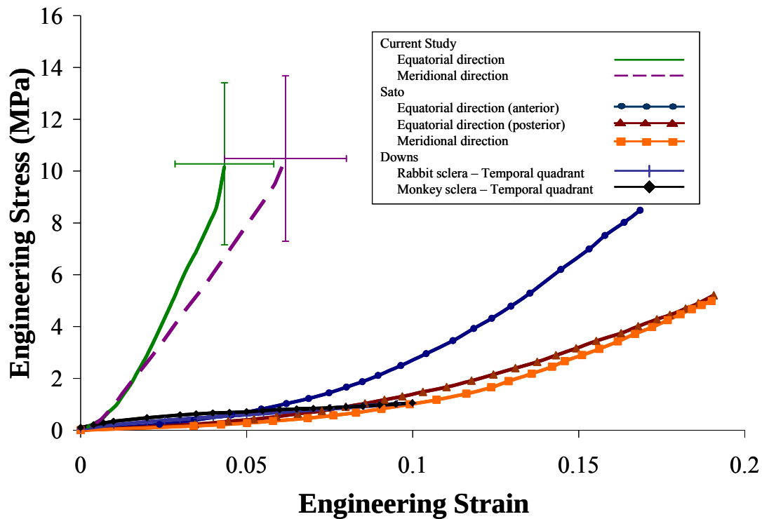
Figure 9: Comparison of previous stress-strain curves to current study.
