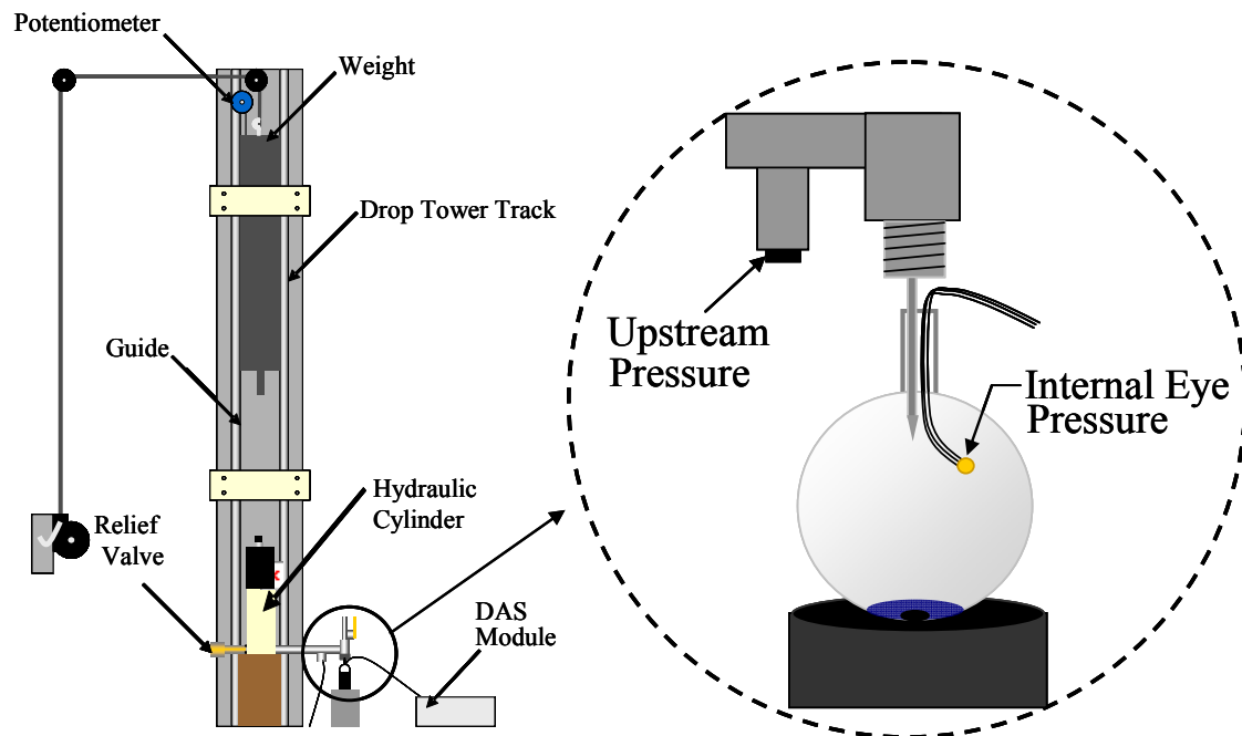
Figure 2: Schematic of pressure system used to examine high rate rupture pressures of human eyes.
