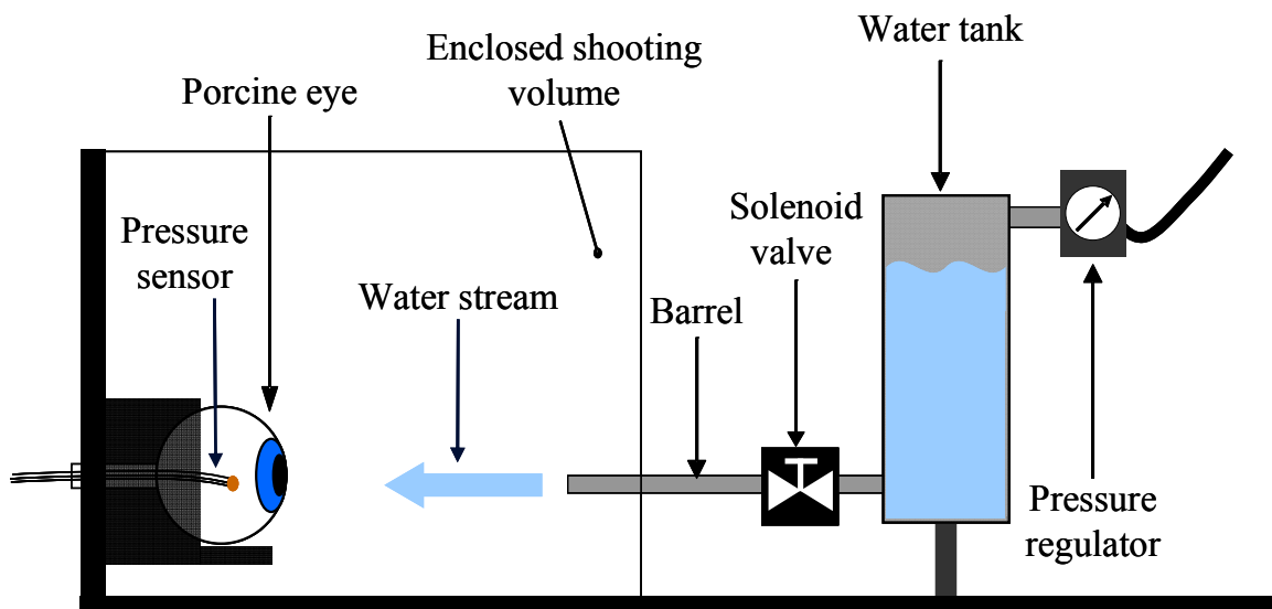
Figure 16: Water stream system used to impact porcine eyes.
