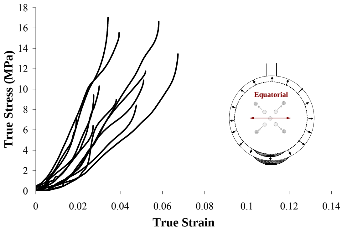
Figure 7: Stress-strain curve responses in the equatorial direction of 12 eye rupture tests.
