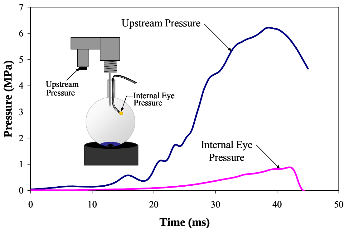
Figure 4: Pressure difference between upstream pressure and direct internal eye pressure.
