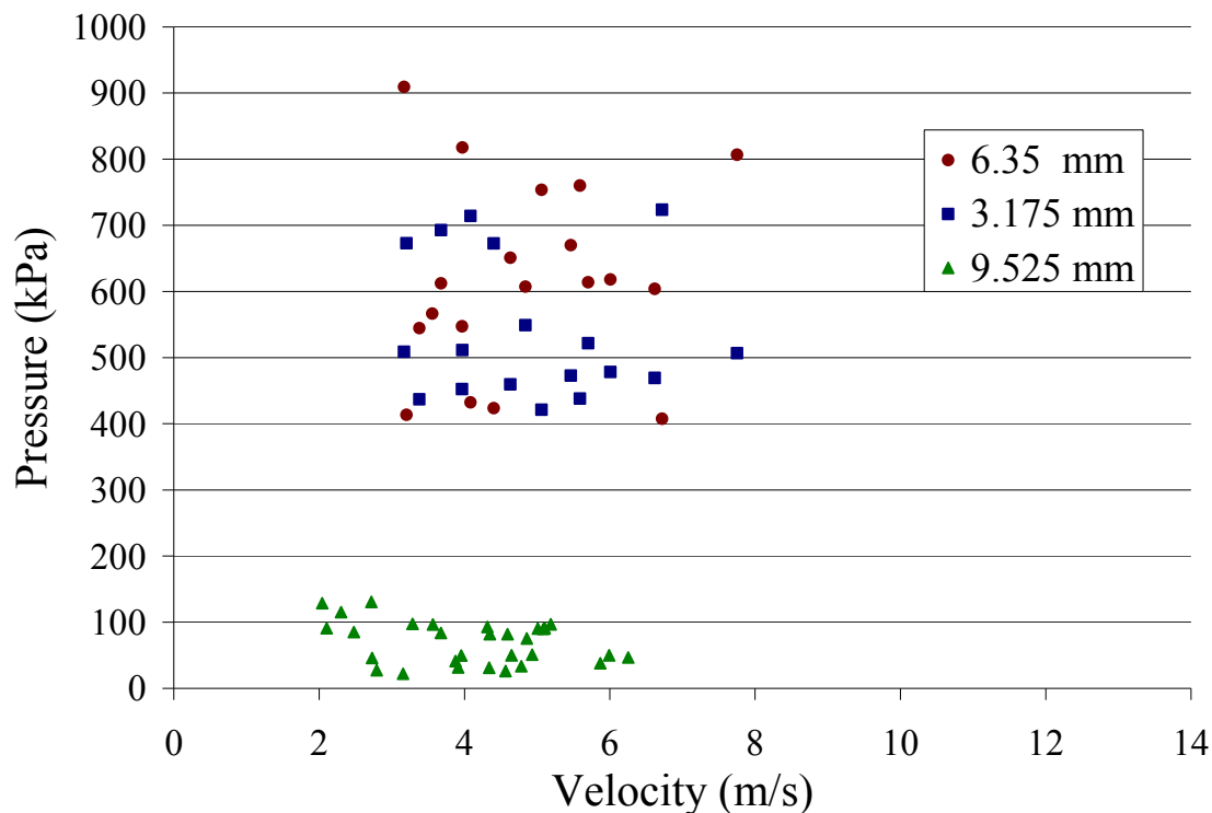
Figure 19: Influence of nozzle diameter and velocity based on intraocular pressure.
