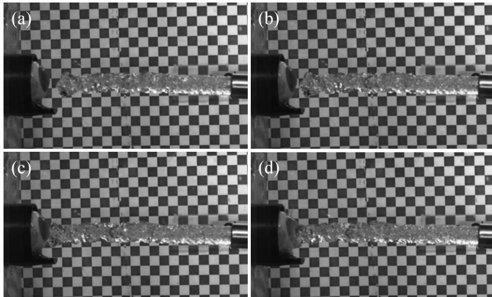
Figure 18: High speed video of a test with a 9.525 mm water stream at 4.23 m/s.
