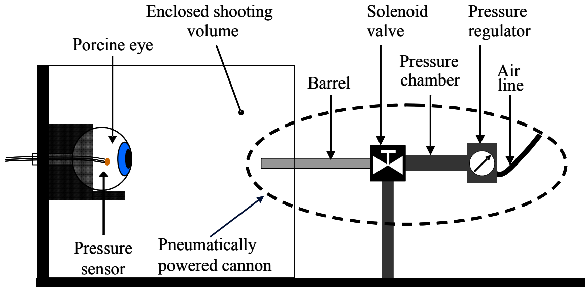
Figure 11: Experimental testing was performed used a pneumatically powered cannon in an enclosed shooting volume to impact porcine eyes.
