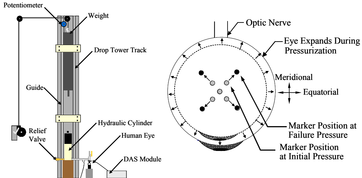
Figure 5: Schematic of high rate pressurization system (left) used to determine material properties and the expansion of a human eye shown with optical markers (right).
