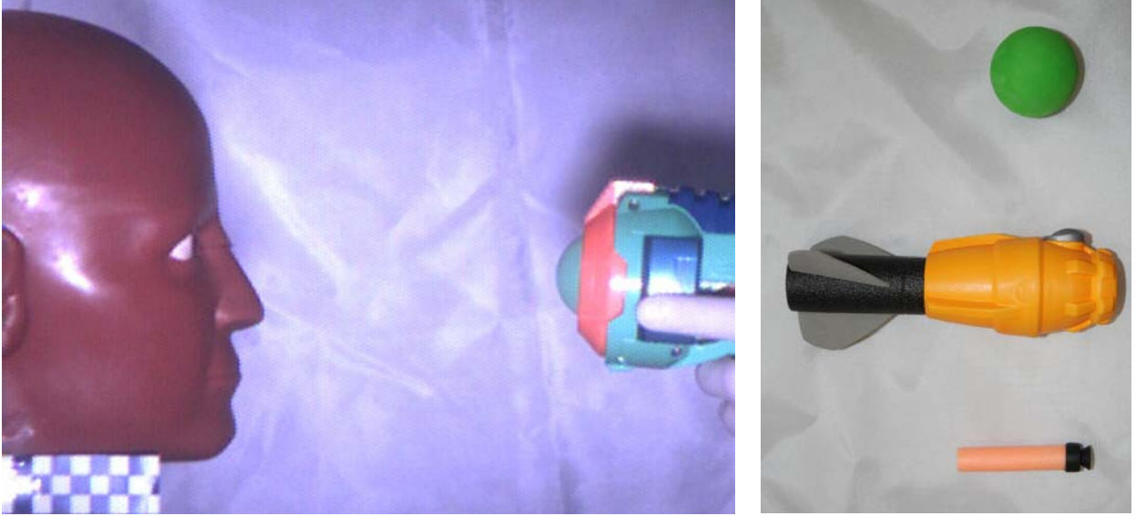
Figure 20: (Left) Experimental setup with the FOCUS headform and the ball launcher. (Right) Relative size comparison of the three projectiles. Top to bottom: ball, foam launcher, dart.
