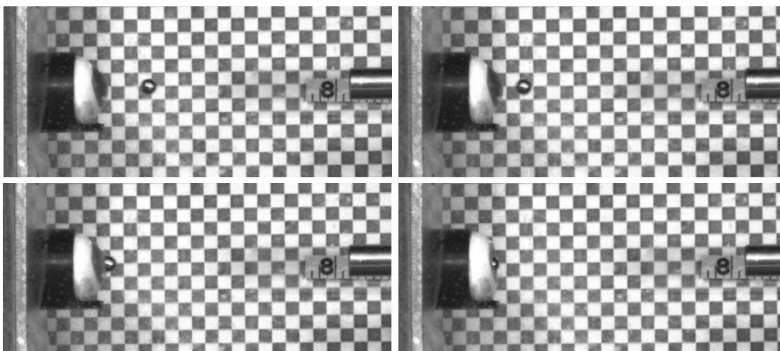
Figure 13: High speed video documentation of a test with the 6.35 mm metal ball projectile.
