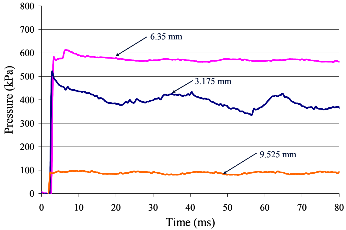
Figure 17: Intraocular pressure response for the three nozzle sizes at a water velocity of 3 m/s.
