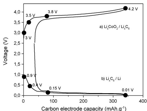
Fig. 1. (a) First cycle of charge/discharge of the operating cell ( \text{LiCoO}_2/\text{Li}_x\text{C}_6 ) studied in this work, (b) corresponding potential of the negative electrode vs. \text{Li}^+/\text{Li} .
