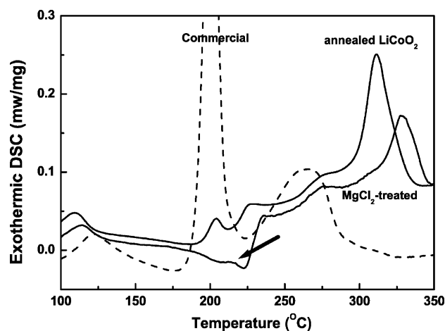
Fig. 5. DSC traces of commercial before (6.6 mg) and after (7.2 mg) 750 °C/2 h processed and 10% MgCl 2 -treated LiCoO 2 (5.9 mg) charged to 4.7 V (the arrow is for the exothermic peak of 10% MgCl 2 -modified LiCoO 2 ).
