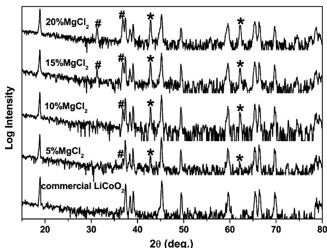
Fig. 2. Logarithm-scaled XRD patterns of LiCoO 2 before and after molten salt process at 750 °C for 2 h (*MgO, #Co 3 O 4 ).
