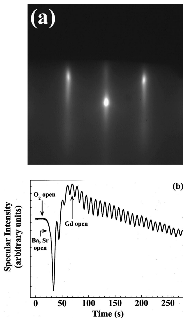
FIG. 9. (a) RHEED image along the [110] azimuth of silicon after the growth of 25 ML of 16% Gd-doped Ba_{0.70}Sr_{0.30}O ( Ba_{0.59}Sr_{0.25}Gd_{0.16}O_y ) grown at 25 °C and 3 \times 10^{-8} Torr and (b) corresponding RHEED intensity oscillations from the specularly reflected reflection.
