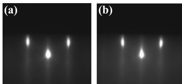
FIG. 6. (a) RHEED image along the [110] azimuth of silicon after the growth of 3 ML of Ba_{0.70}Sr_{0.30}O grown following PATH 1 as shown in Fig. 2. (b) RHEED image along the [110] azimuth of silicon after the growth of 3 ML of Ba_{0.70}Sr_{0.30}O grown following PATH 2 as shown in Fig. 2. The epitaxial relationship is described as (001) Ba_{0.70}Sr_{0.30}O \parallel (001) Si and [100] Ba_{0.70}Sr_{0.30}O \parallel [100] Si . These two images demonstrate the ability to grow epitaxial alkaline-earth oxides using various deposition paths.
