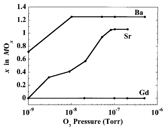
FIG. 5. Plot showing degree of oxidation for strontium, barium, and gadolinium metal as a function of O_2 partial pressure. This plot was generated directly from the data shown in Fig. 4.
