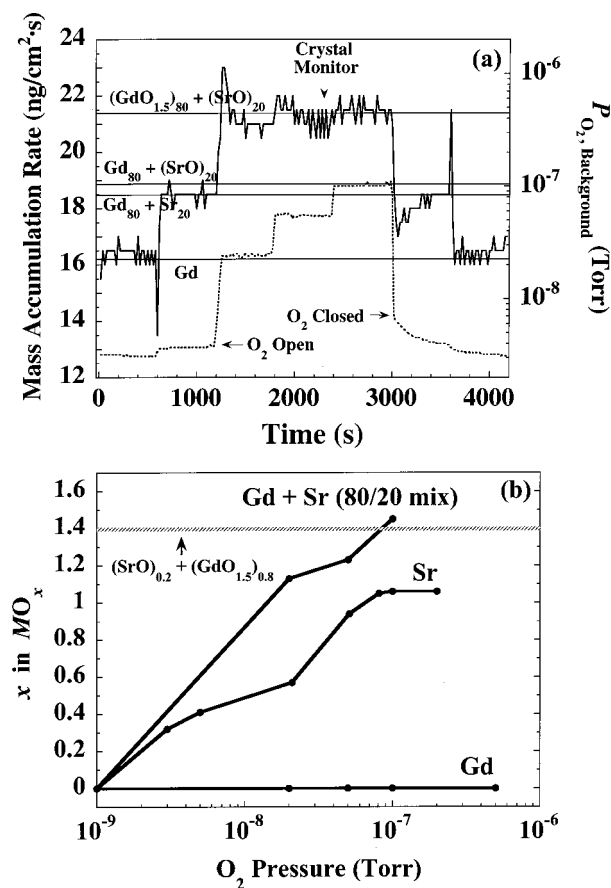
FIG. 8. (a) Graph similar to the plots shown in Fig. 4 showing mass accumulation rate on the QCM as a function of time for varying O_2 partial pressures for a 80% Gd/20% Sr mix. (b) Plot showing degree of oxidation for strontium, gadolinium, and a 80% Gd/20% Sr mix as a function of O_2 partial pressure. The plot demonstrates the catalytic nature of the alkaline earth and indicates that full oxidation occurs orders of magnitude lower than for the deposition of the pure gadolinium metal alone.
