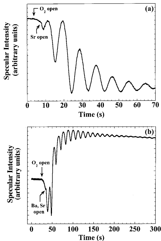
FIG. 7. RHEED intensity oscillations of the specularly reflected spot along the [110] azimuth of silicon at 25 °C during deposition in 3 \times 10^{-8} Torr O 2 for: (a) SrO and (b) lattice-matched (Ba, Sr)O. The oscillations of the mismatched SrO show a decreasing intensity and dampening of oscillations.
