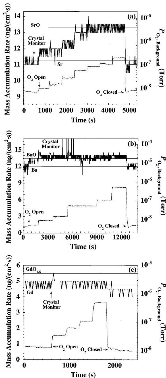
FIG. 4. Graphs showing mass accumulation rate on the QCM as a function of time for varying O_2 partial pressures for (a) strontium, (b) barium, and (c) gadolinium. The labeled, horizontal lines indicate the positions corresponding to the deposition of the pure metal and fully oxidized metals. From the plots one can see the general ease of oxidation of the strontium and barium in contrast with the general difficulty in oxidizing the gadolinium. All experiments were conducted at room temperature with a metallic flux of (2-7) \times 10^{13} atoms/cm 2 s.
