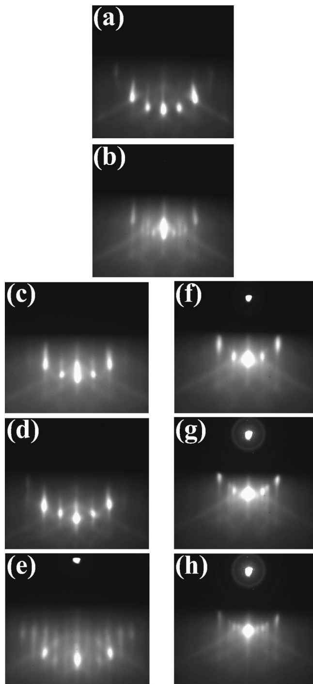
FIG. 3. RHEED images along the [110] azimuth of silicon taken at various stages of the growth for two distinct paths as outlined in Fig. 2. (a) (2 \times 1) reconstructed silicon surface after heating in vacuum to temperatures above 840^\circ\text{C} for 20 min. (b) After the deposition of a 1/6 ML strontium dose at 700^\circ\text{C} , showing the evolution to a 3 \times pattern. PATH 1 (c) after the deposition of a 1/2 ML strontium dose at 700^\circ\text{C} , showing the return to the 2 \times pattern with a maximum intensity. (d) Same film shown in Fig. 3(c) after cooling to 120^\circ\text{C} . Note the lack of change in the pattern. (e) After the deposition of a 1/2 ML strontium dose deposited at 120^\circ\text{C} showing the formation of the 3 \times metal overlayer. PATH 2 (f) after the deposition of a 1/4 ML strontium dose at 700^\circ\text{C} . (g) Same film shown in Fig. 3(f) after cooling to 120^\circ\text{C} . Note the change from the previous pattern. (h) After the deposition of a 3/8 ML strontium dose deposited at 120^\circ\text{C} while following PATH 2. It should be noted that the RHEED images shown are all before the introduction of oxygen into the chamber. The flux of strontium for these two growths was 2 \times 10^{13} atoms/ \text{cm}^2 s.
