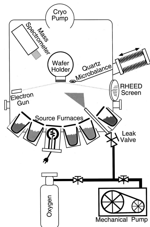
FIG. 1. Schematic of the MBE growth chamber used for the deposition of alkaline-earth oxides on silicon.
