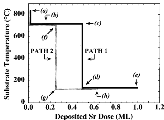
FIG. 2. Process flow diagram showing the temperature and deposited strontium dose for two different growth paths. The diagram indicates that although the RHEED signature may vary slightly, some latitude exists in terms of strontium dosages that lead to epitaxial alkaline-earth oxide in subsequent steps. The letter labels correspond to the respective RHEED images in Fig. 3.
