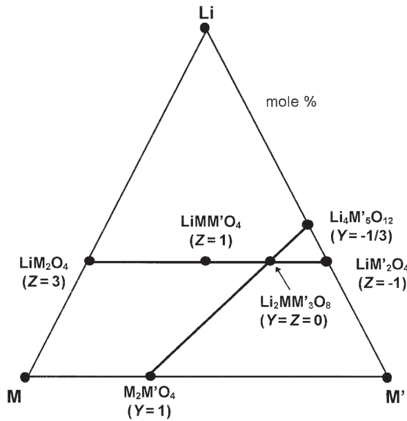
Fig. 1. Possible formation of spinel solid solutions \text{Li}_{2-2Y}\text{M}_{1+3Y}\text{M}'_{3-Y}\text{O}_8 and \text{Li}_2\text{M}_{1+Z}\text{M}'_{3-Z}\text{O}_8 in the systems \text{Li}-\text{M}-\text{M}'-\text{O} . Oxygen contents are not specified.
