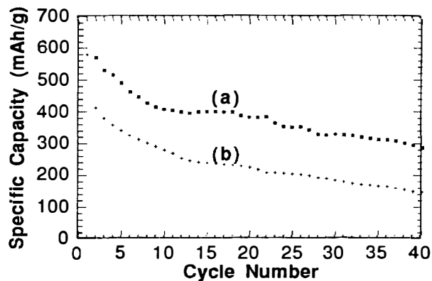
Fig. 4. Influence of the first discharge rate on the further cycleability of a \text{Li}_x\text{CoVO}_4 composite electrode (mass ratio = (79:16.5)), cycled at a rate corresponding to 1 Li per \text{LiCoVO}_4 per h, between 0.02 and 2.6 V. The first discharge rate was either (a) C/100 or (b) C/15 .
