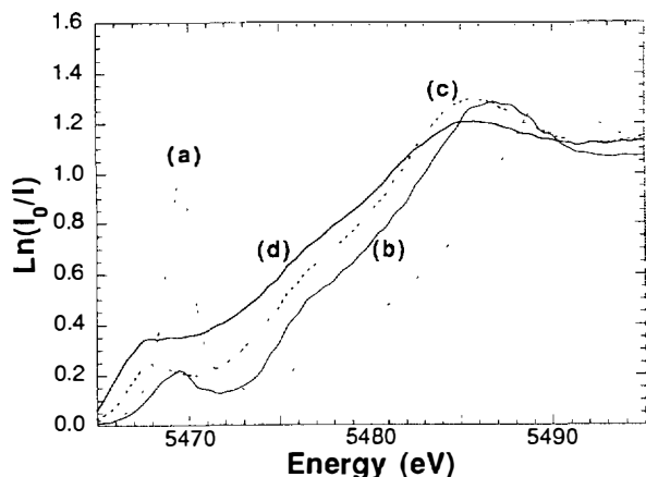
Fig. 7. Comparison of the vanadium k -edge XANES spectra of (a) \text{LiNiVO}_4 and (b) \text{Li}_x\text{NiVO}_4 compounds electrochemically prepared during the first discharge, with: (b) \lambda = 3 , \lambda = 5.5 , and \lambda = 8
