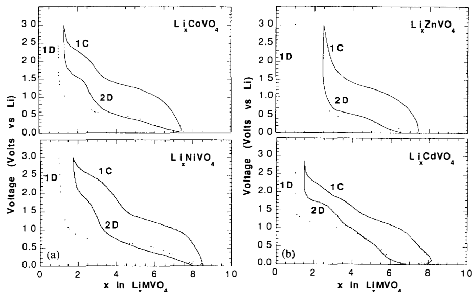
Fig. 2 (a), (b) Voltage vs. Li composition curves, intrinsic to \text{Li}_x\text{MVO}_4 materials, at the three first half-cycles, measured by cyclic voltammetry at 10 mV/h between 0.02 and 3 V. The n th discharge and charge are respectively denoted nD and nC .
