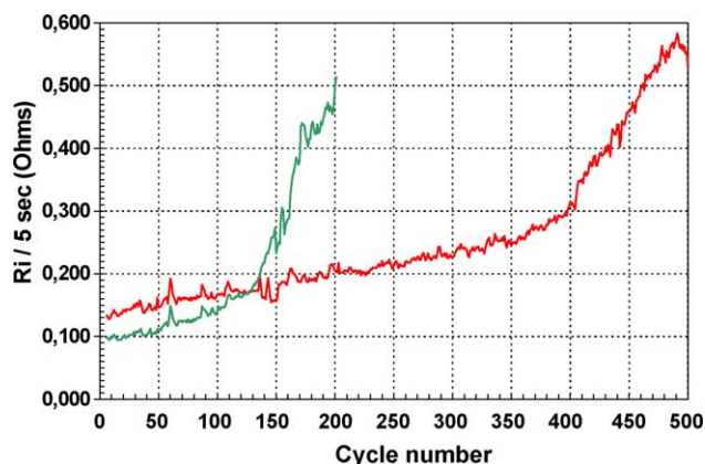
Fig. 3. Example of resistance evolutions during 100% DOD cycling. \text{LiCoO}_2 /graphite pouch cells, charge at C, discharge at C/2, 20 °C (see Fig. 2).
