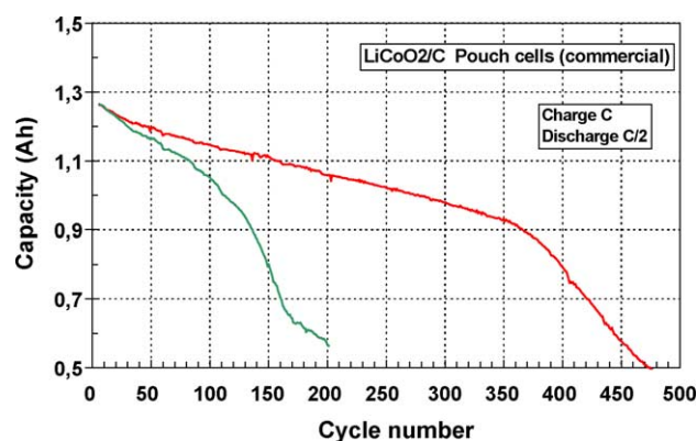
Fig. 2. Example of capacity evolutions during 100% DOD cycling. \text{LiCoO}_2 /graphite pouch cells, charge at C, discharge at C/2, 20 °C).
