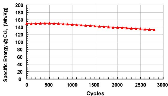
Fig. 4. Example of deep cycling (80% DOD, EV type) of Saft VLE 45 Ah Li ion cells. 100% DOD C/3 diagnostic test every 100 cycles at 20 °C.
