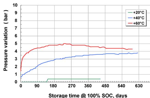
Fig. 14. Long-term pressure evolution of Li ion \text{LiNi}_x\text{Co}_y\text{Al}_z\text{O}_2 /natural graphite cells at 100% SOC (4 V), for several temperatures.
