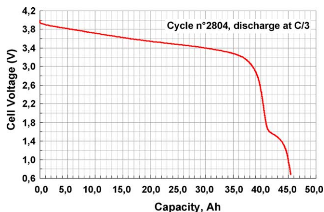
Fig. 6. Full discharge to 0.7 V of VLE 45 Ah cell after 2804 cycles at 80% DOD (see Fig. 4).
