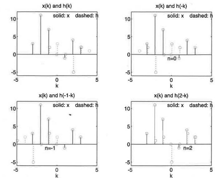
FIGURE 2.7 Graphical convolution in Example 2.6
