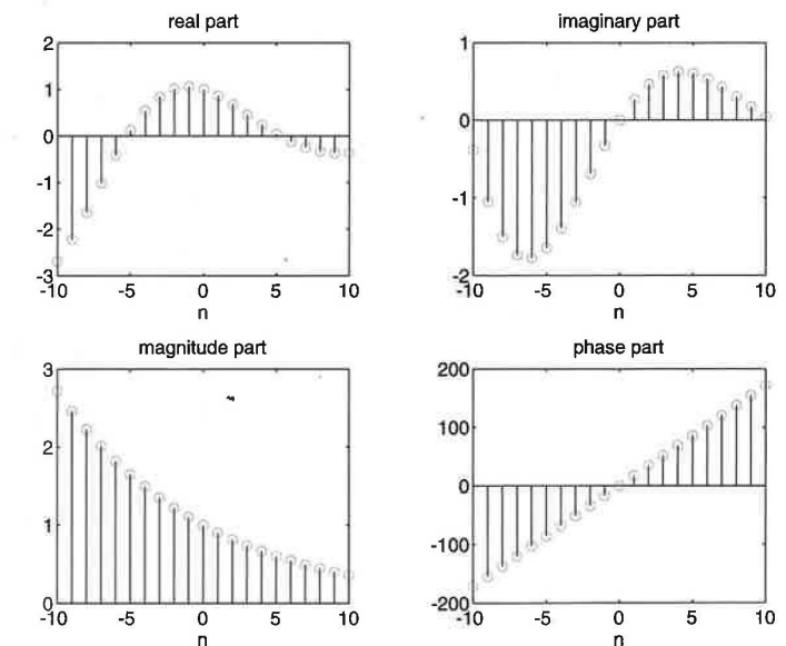
FIGURE 2.3 Complex-valued sequence plots in Example 2.3
