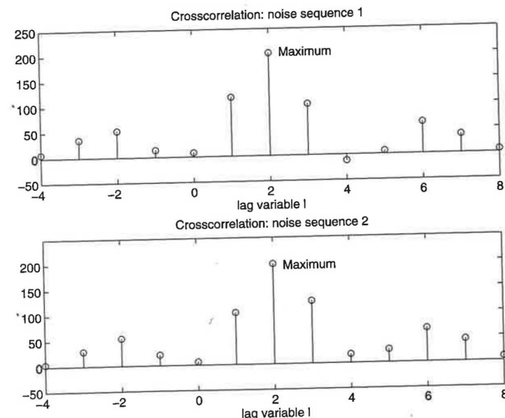
FIGURE 2.8 Crosscorrelation sequence with two different noise realizations
