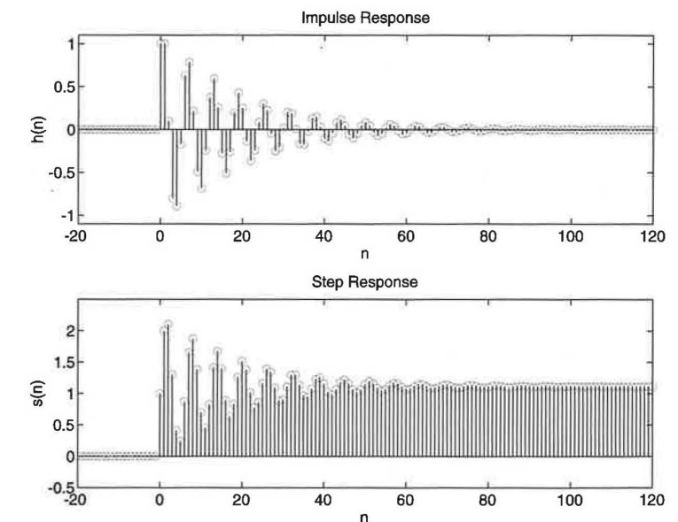
FIGURE 2.9 Impulse response and step response plots in Example 2.9
