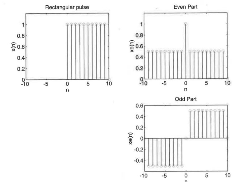
FIGURE 2.4 Even-odd decomposition in Example 2.4
