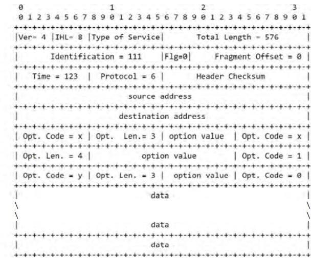
Example Internet Datagram
