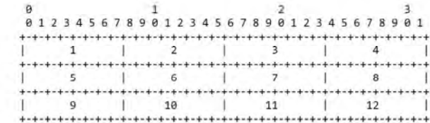
Transmission Order of Bytes
