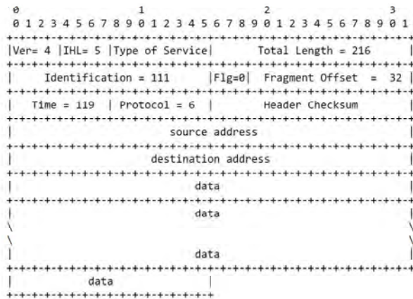
Example Internet Fragment
