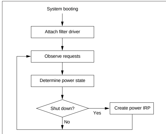
Figure 4. Power management by filter driver.
