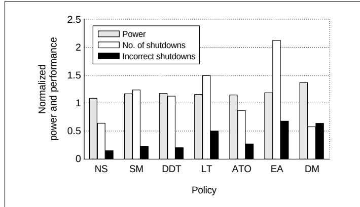
Figure 7. Power, number of shutdowns, and percentage of incorrect shutdowns for each policy. The power and number of shutdowns are normalized to the oracle policy. Shorter bars are better.
