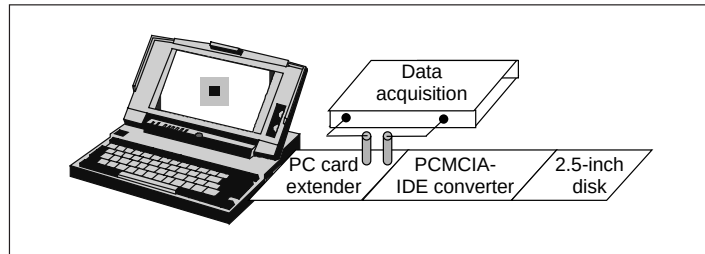
Figure 5. Setup for measuring disk power through the PCMCIA interface.
