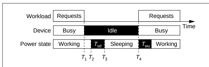
Figure 1. Power management from the workload, device, and power state points of view.
