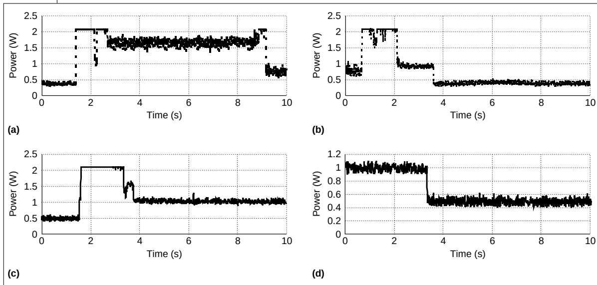
Figure 6. State transitions of two hard disks: Hitachi disk (a) wake up and (b) shut down; and Fujitsu disk (c) wake up and (d) shut down.
