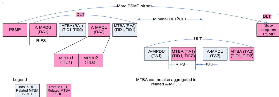
Figure 33 – PSMP sequence
