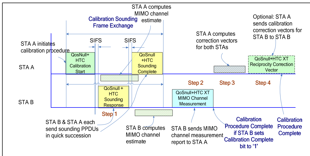
Figure 40 – Calibration Procedure
