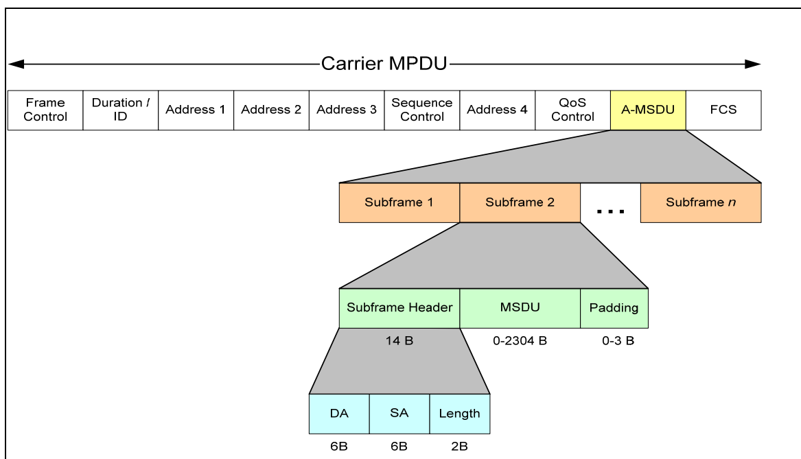
Figure 28 – A-MSDU Structure
