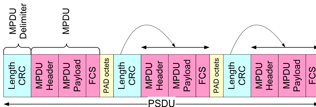
Figure 27 – A-MPDU format
