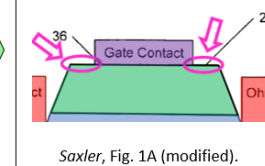
Modified Saxler Fig. 1A Gate Structure
