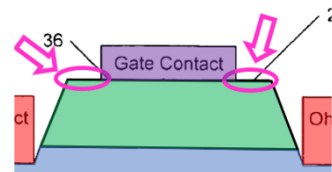
Saxler, Fig. 1A (modified).
