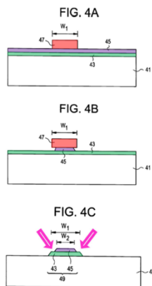
Ahn, Figs. 4A-4C.
