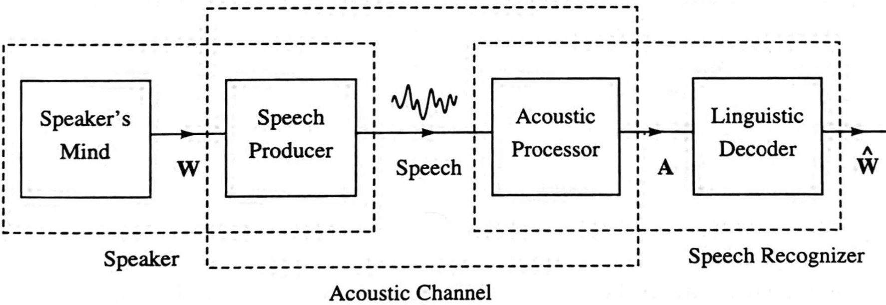
Figure 1.3 Source-channel model of speech recognition
