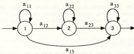
Fig. 16. An example of a three-state HMM.
