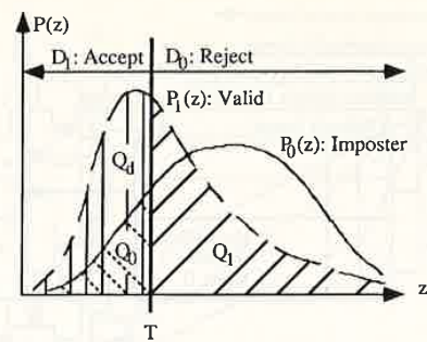
Fig. 17. Valid and impostor densities.
