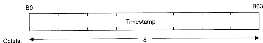
Figure 33—Timestamp fixed field
