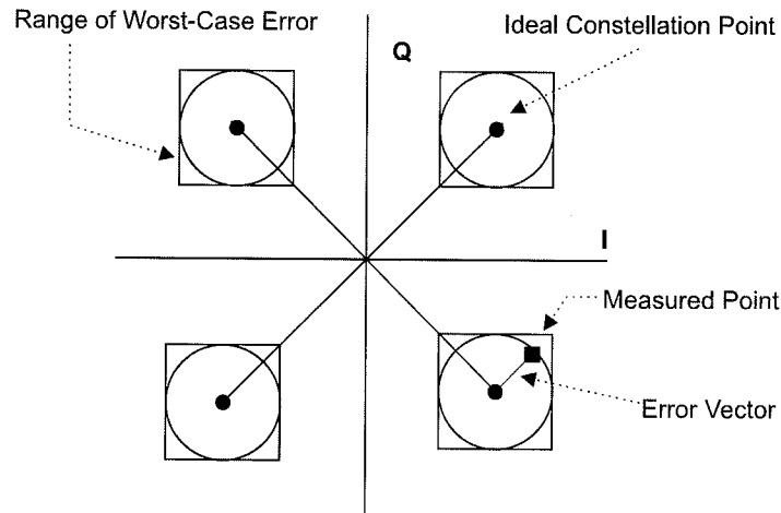
Figure 99—Modulation accuracy measurement example
