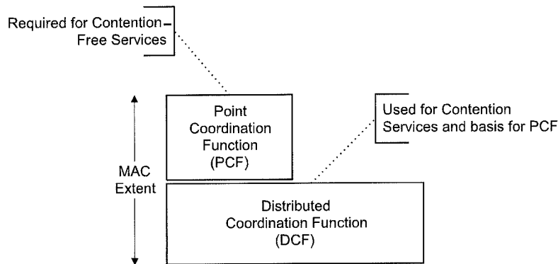
Figure 47—MAC architecture
