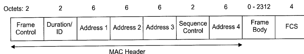
Figure 12—MAC frame format
