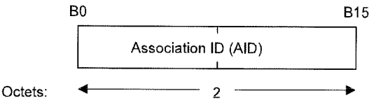
Figure 31—AID fixed field
