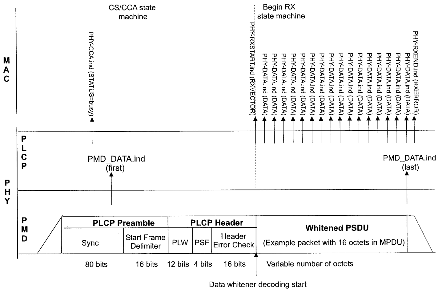
Figure 81—Receive timing
