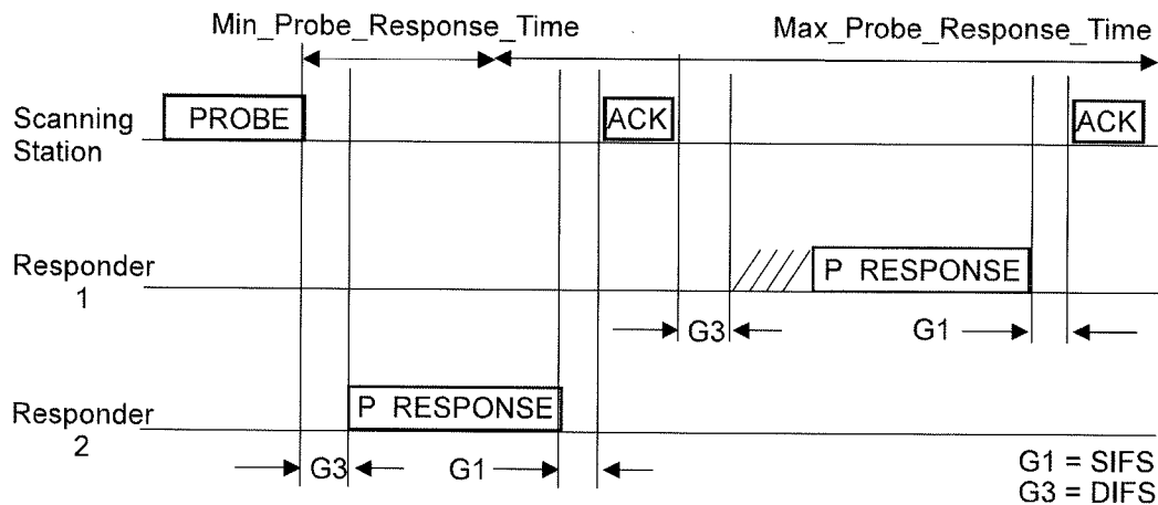
Figure 66—Probe response
