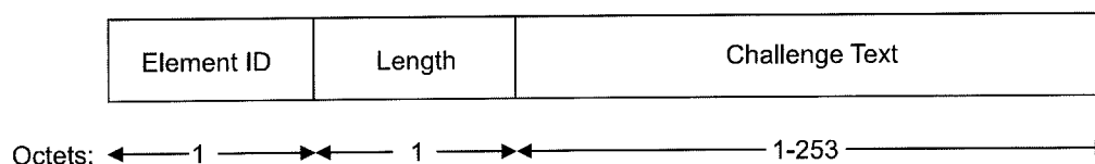
Figure 42—Challenge Text element format
