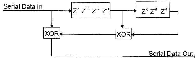
Figure 90—Data descrambler
