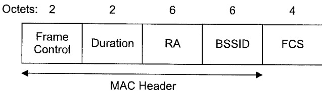
Figure 20—CF-End frame
