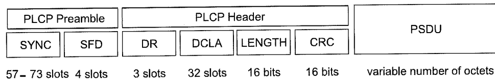
Figure 101—PLCPDU frame format
