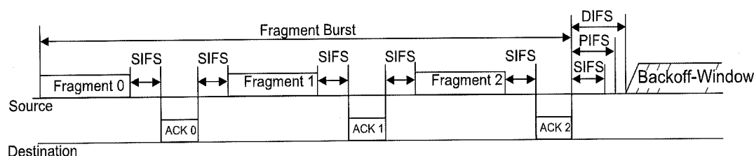
Figure 54—Transmission of a multiple-fragment MSDU using SIFS
