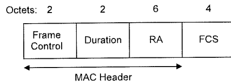
Figure 17—CTS frame
