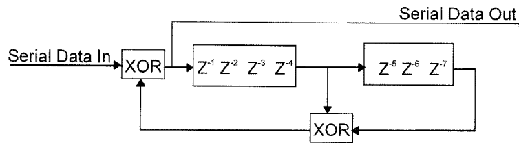
Figure 89—Data scrambler
