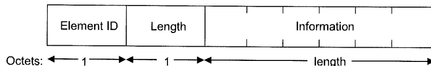
Figure 34—Element format
