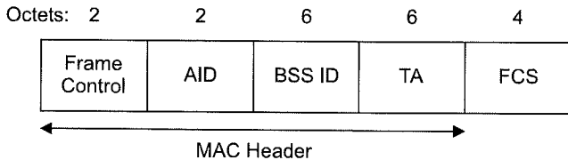
Figure 19—PS-Poll frame
