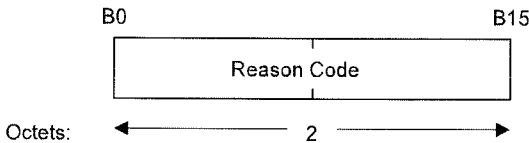
Figure 30—Reason Code fixed field
