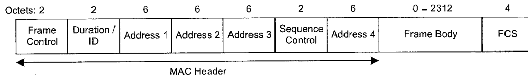
Figure 22—Data frame
