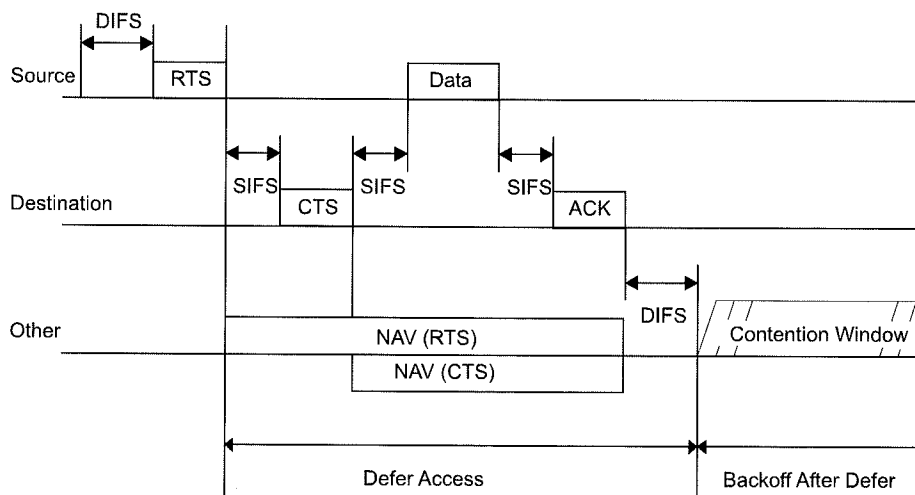
Figure 53—RTS/CTS/data/ACK and NAV setting
