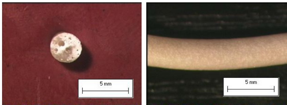
Void in PP-kaolin composites extrudates cross section
