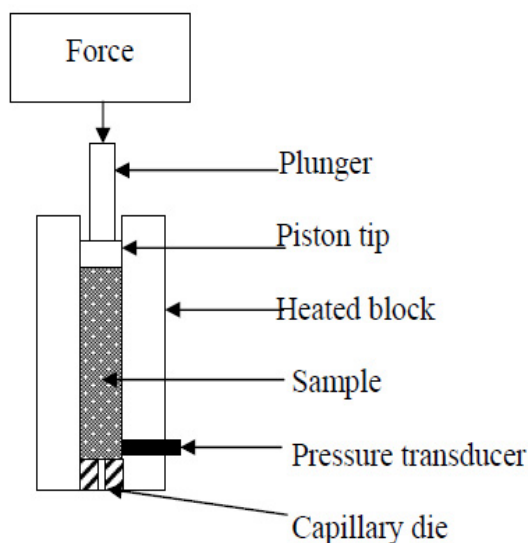
Fig. 2. Schematic diagram for capillary rheometer
