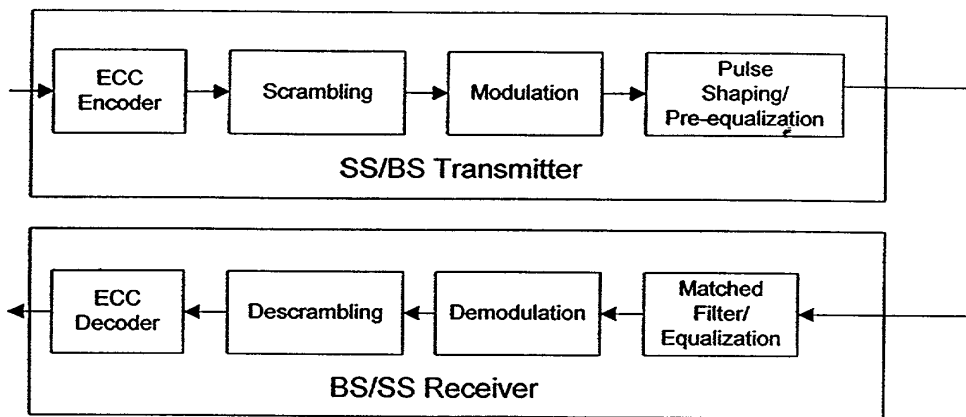
PHY Reference Model Showing Data Flow
