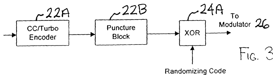
PHY Reference Model Showing Data Flow
