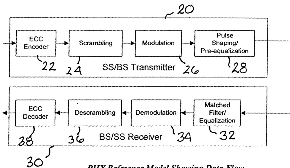
PHY Reference Model Showing Data Flow
