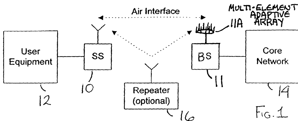
Wireless Access Reference Model
