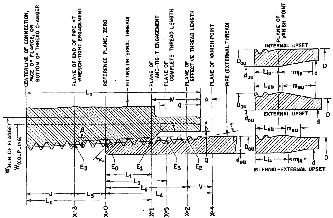
FIGURE 1.5. Pipe and pipe thread symbols (see table 1.6).
