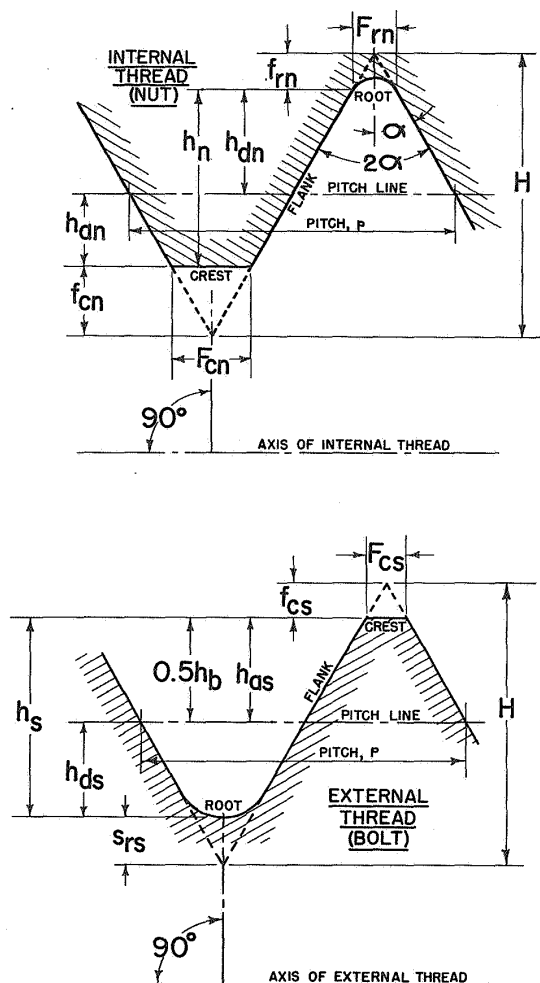
FIGURE 2.4. Symbols for thread data in table 2.1.
