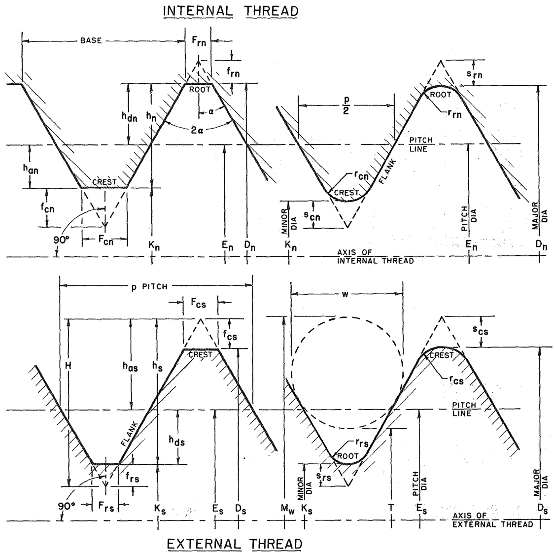
FIGURE 1.3. General screw thread symbols (see table 1.4).
