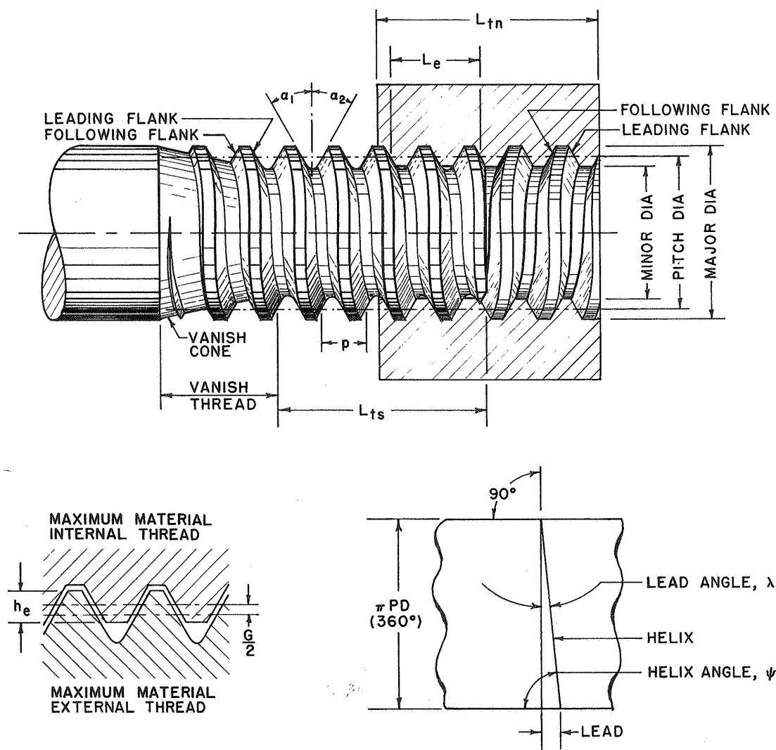
FIGURE 1.2. General screw thread symbols (see table 1.4).
