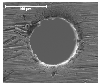
Figure 5. An eroded orifice edge – diameter = 127 μ Source: NCRC
