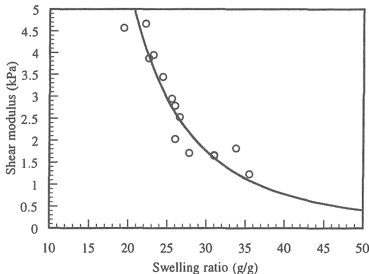
Figure 1.4. The correlation of shear modulus to the swelling ratio for superabsorbent polymers swollen to equilibrium in 0.9% NaCl solution. The samples vary in crosslink density. The shear modulus scales as the -2.83 power of the swelling ratio in this figure.
