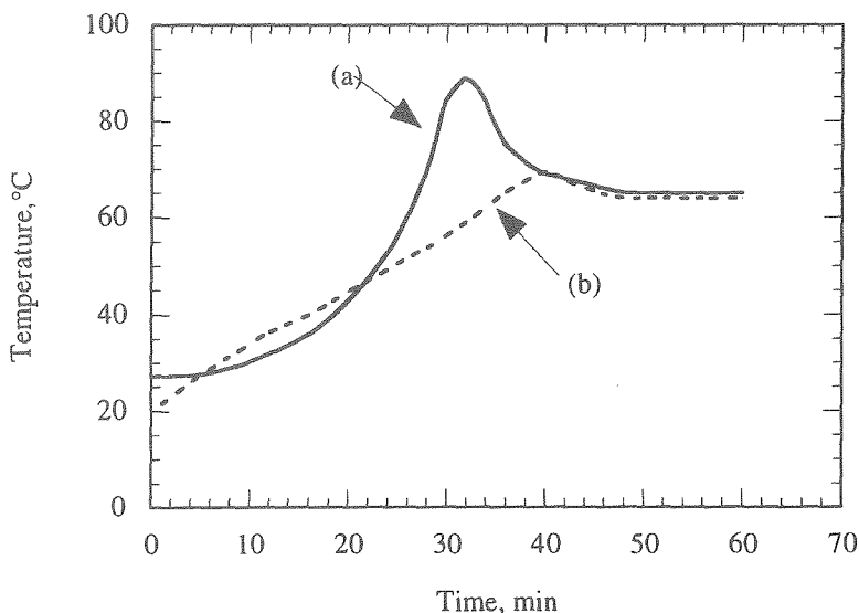
Figure 3.3. Temperature versus time for polymerizations in a 2-L laboratory reactor with no cooling except through heat losses to the atmosphere. Monomer solution 1,200 g was loaded to the reactor: (a) 32 wt%, 65% neutralized acrylic acid 28 ; (b) 20 wt% acrylic acid. 35
