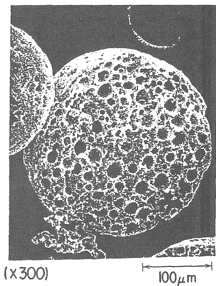
Figure 3.13. Cross-sectional view of porous beads prepared by o/w/o suspension polymerization.
