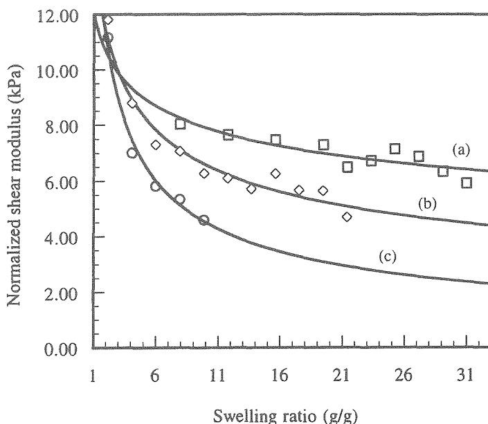
Figure 5.4. Shear modulus of partially neutralized poly(acrylic acid) gel, normalized to the volume of preparation, as a function of the swelling ratio in three different concentrations of sodium chloride, 0.0325% (a), 0.125% (b), and 0.9% (c).
