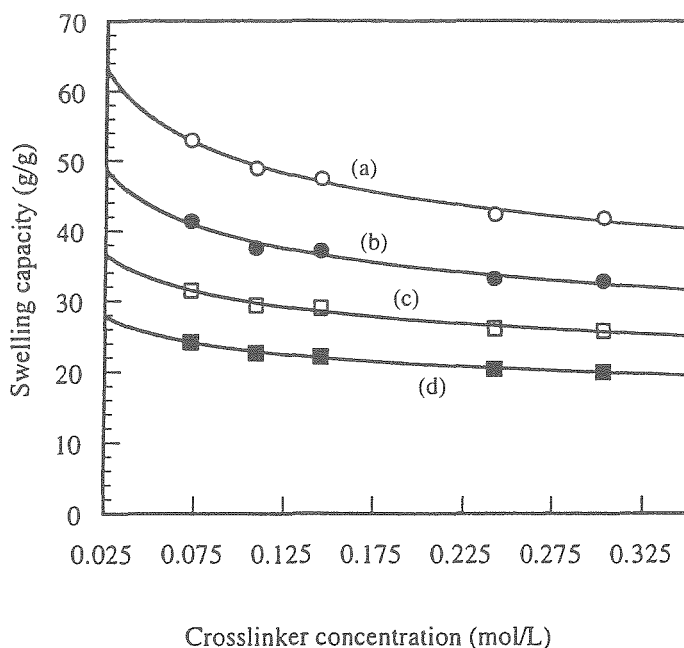
Figure 5.7. The dependence of the swelling capacity on the concentration of crosslinks during preparation of the gel and on the concentration of NaCl in the swelling liquid: (a) 0.225%, (b) 0.45%, (c) 0.90%, (d) 1.80%. The gels were polymerized at identical concentrations of monomer, using 1,3-butylene glycol diacrylate as the crosslinker and with 65% of the carboxylic acid groups neutralized.
