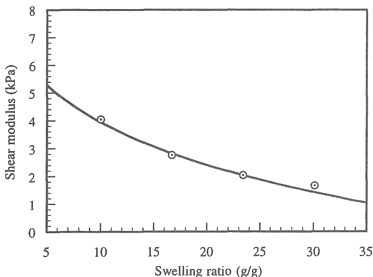
Figure 5.3. The shear modulus dependence on the swelling ratio of the sample. A single sample of superabsorbent polymer was swollen to less than equilibrium by limiting the fluid available. The modulus scales with the -0.37 power of the swelling ratio.
