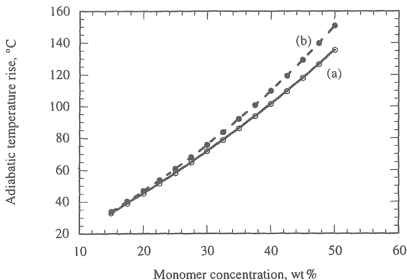
Figure 3.2. Adiabatic temperature rise for polymerizations of crosslinked partially neutralized acrylic acid as a function of monomer concentration. The heat of polymerization of acrylic acid was taken as 77.4 kJ/mol, and the heat capacity of the polymer was taken as either 0.50 (a) or 0.35 cal/g°C (b).
