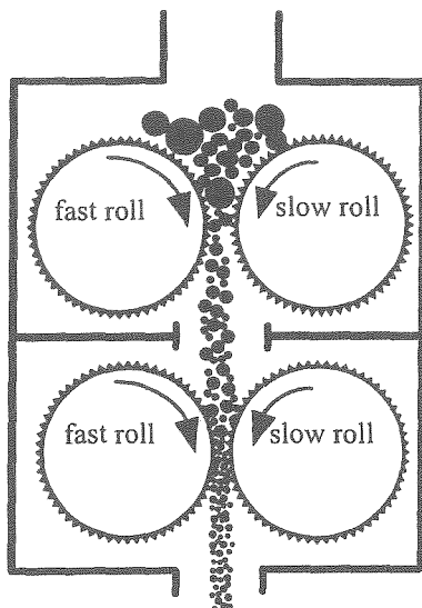
Figure 3.8. Schematic diagram of a two-pair high roll crusher.
