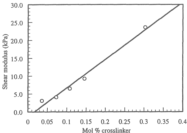
Figure 5.1. The shear modulus of sodium polyacrylate gels as a function of the stoichiometric ratio of crosslinker used in the polymerization, per mole of acrylic acid. The moduli have been normalized to the preparation volume according to Eq. 5.7.
