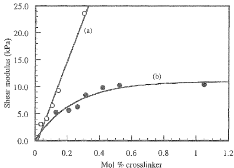
Figure 4. Impact of crosslinker loading per mole of monomer on the shear modulus of a SAP using (a) 1,3-butyleneglycol diacrylate and (b) triallylamine as crosslinking agents. 30
