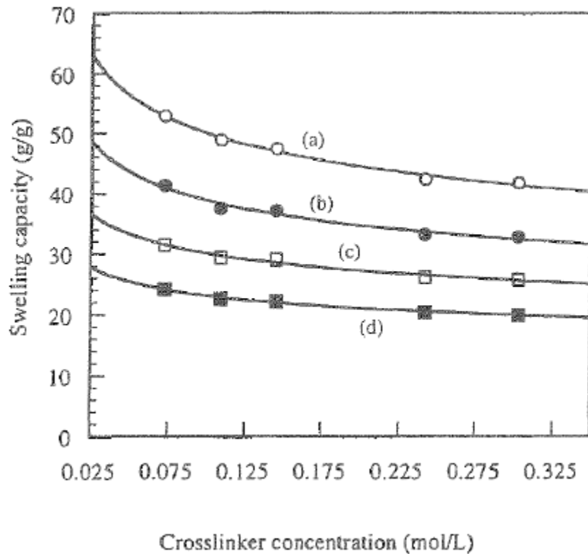
Figure 5. Swelling capacity as a function of crosslinker concentration when a SAP series is swollen in various salt solutions: (a) 0.225% NaCl, (b) 0.45% NaCl, (c) 0.9% NaCl, (d) 1.8% NaCl. 37
