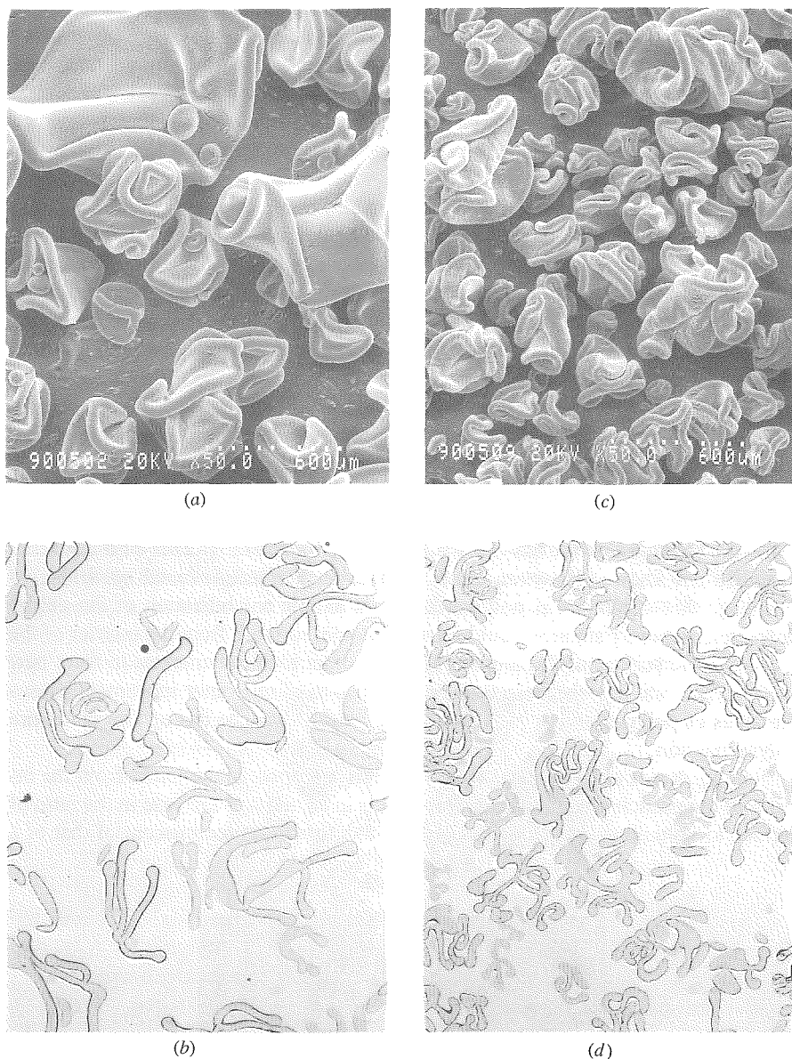
Figure 3.15. (a–d) Highly convoluted superabsorbent particles prepared by suspension polymerization: (b) and (d) are cross-sectional views of (a) and (c), respectively.
