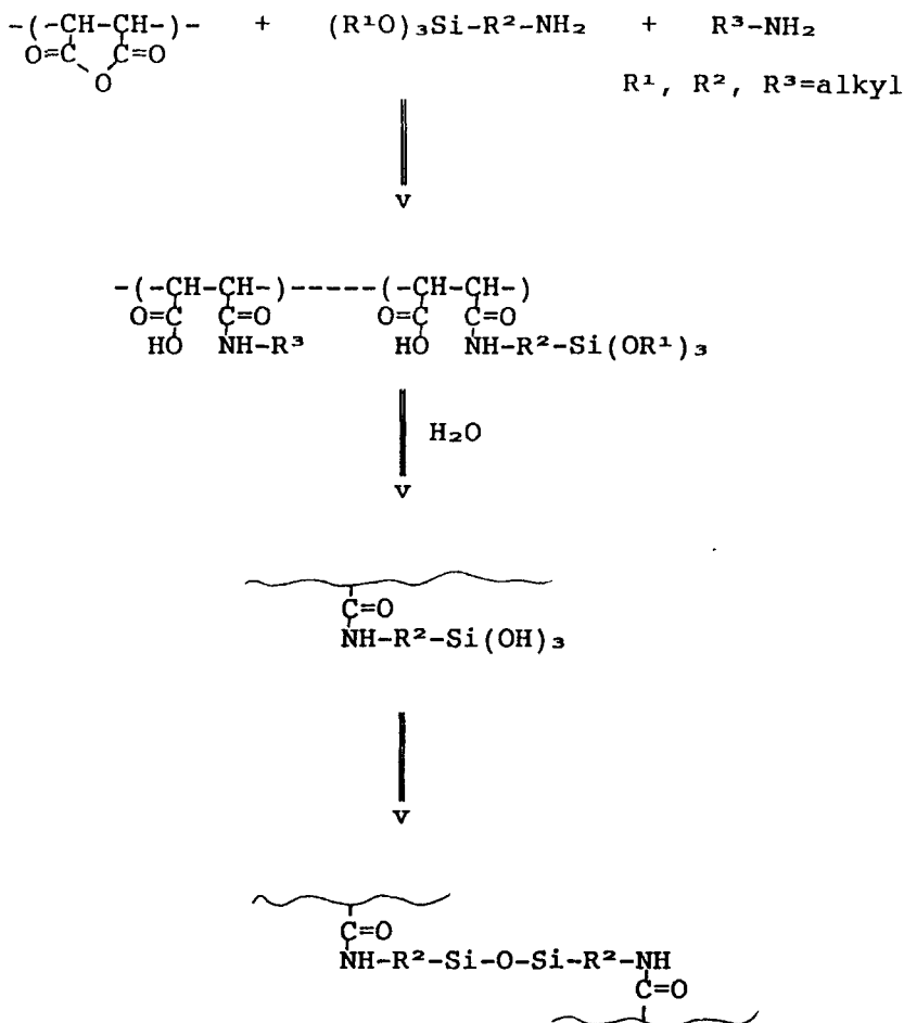
SCHEME 3.
