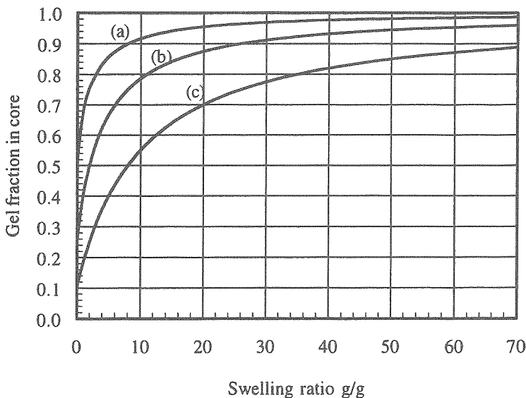
Figure 7.2. The fraction of gel in the absorbent core as a function of the swollen volume of the polymer for three different initial weight ratios of polymer to fluff: (a) f_{SAP} = 0.5 , (b) f_{SAP} = 0.25 , and (c) f_{SAP} = 0.1 .
