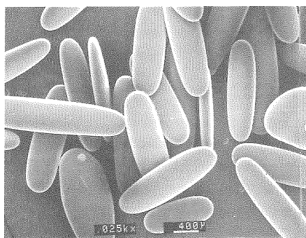
Figure 3.14. Elongated superabsorbent particles prepared by viscosifying the aqueous phase of a suspension polymerization. (Sample courtesy of Nippon Shokubai Co. Ltd.)
