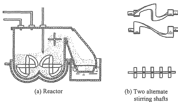
Figure 3.4. Dual-shaft jacketed kneader reactor and two other possible rotary stirring shafts. (Drawn from Tsubakimoto and Shimomura 32 ).
