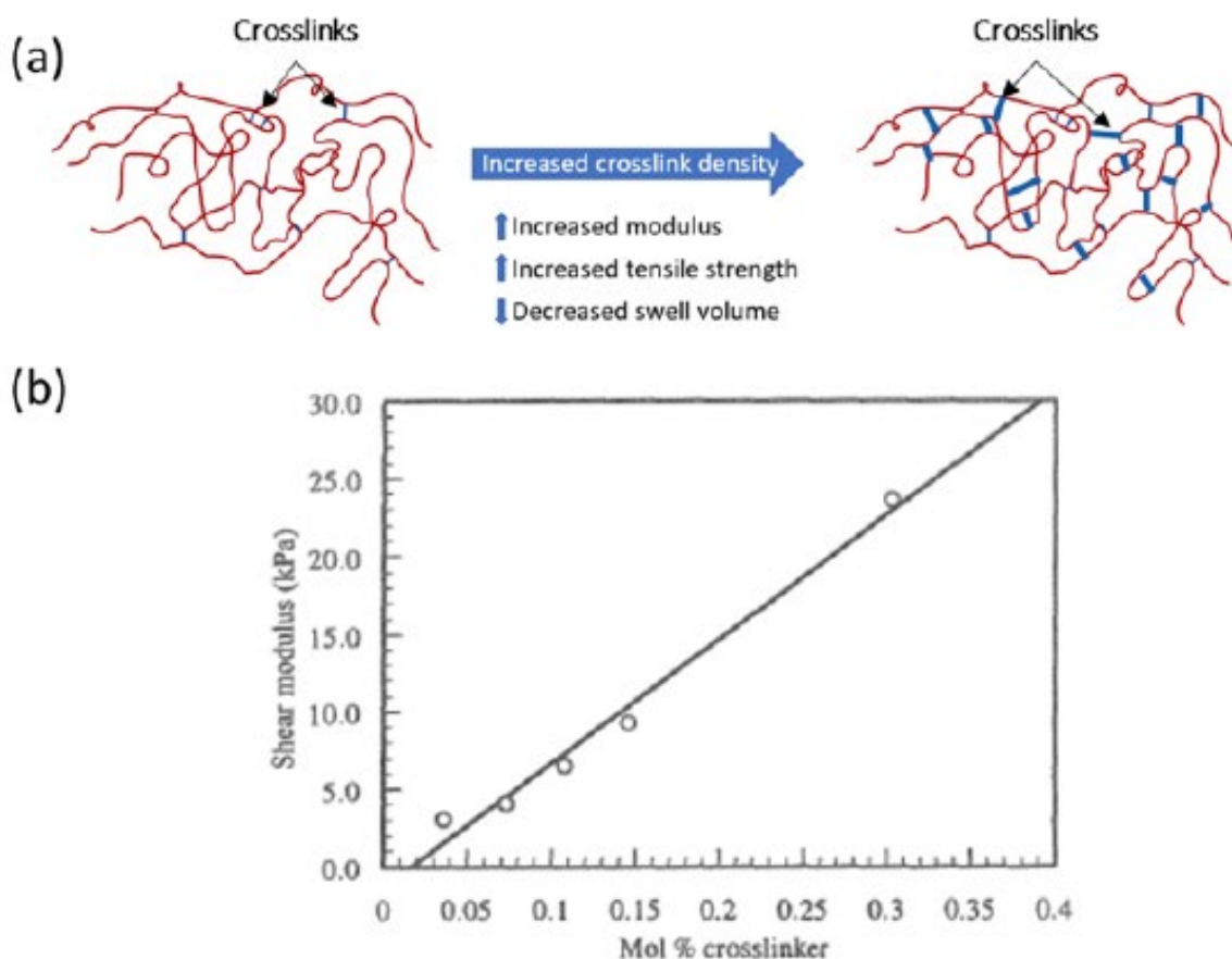
Figure 2. (a) Schematic representation of crosslinked polymer chain molecules with different crosslink densities. A crosslinked polymer network with an increased crosslink density would have an increased modulus, increased tensile strength, and decreased swell volume. 5 (b) Graphical representation of the
