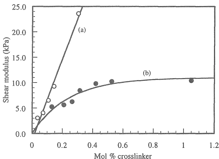
Figure 5.2. Shear modulus as a function of the amount of crosslinker used per mole of acrylic acid, for two structurally different crosslinkers, 1,3-butyleneglycol diacrylate (a) and triallylamine (b).
