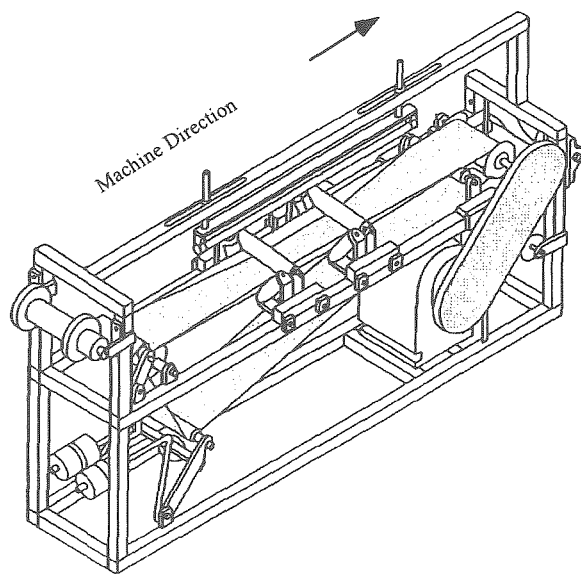
Figure 3.5. Continuous belt reactor with trough to contain liquid monomer. (Drawn from Chmelir and Paven 27 ).
