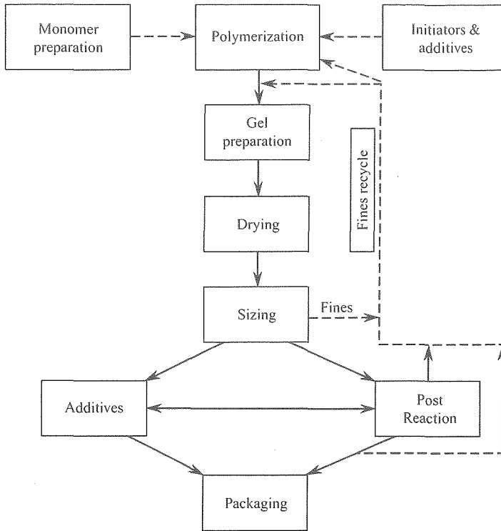
Figure 3.1. A block flow diagram of a generic solution polymerization process.
