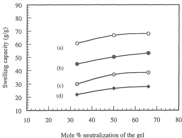
Figure 5.8. The dependence of swelling capacity on the extent of neutralization of the carboxylic acid groups and on the NaCl concentration (by weight) of the swelling liquid: (a) 0.225%, (b) 0.45%, (c) 0.9%, (d) 1.8%. The data are for one prepared gel that was neutralized to different extents after network formation.
