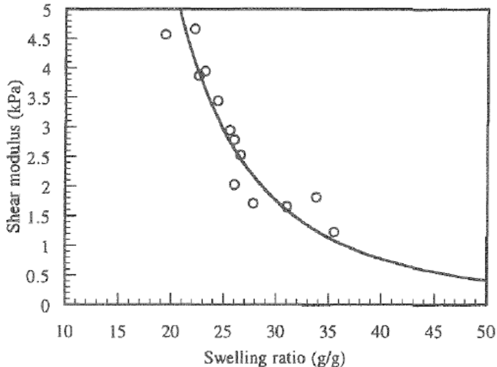
Figure 6. An example of shear modulus as a function of swelling ratio for SAP samples at equilibrium after swelling in a 0.9% NaCl solution. 41 Changes in gel strength relative to swelling ratio are specific to the analyzed SAPs.
