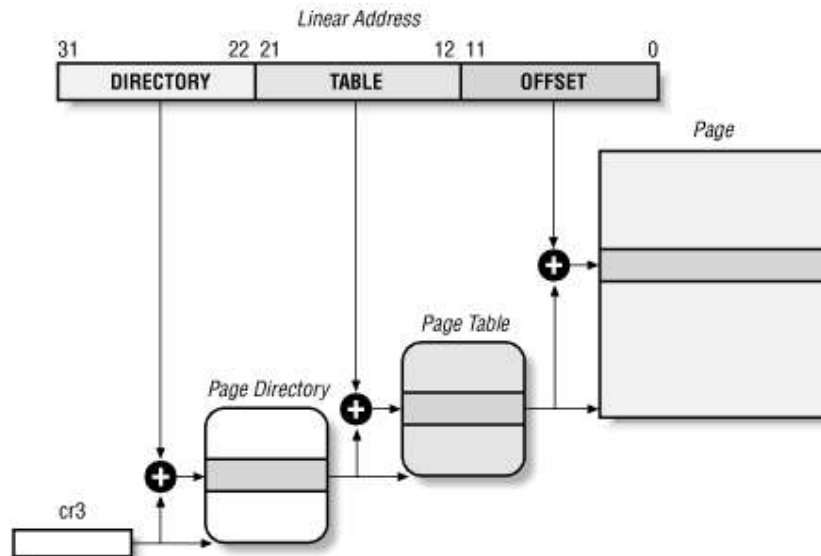
Figure 2-5. Paging by Intel 80x86 processors
