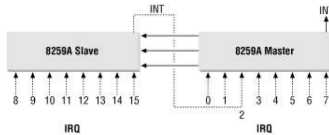
Figure 4-1. Connecting two 8259A PICs in cascade
