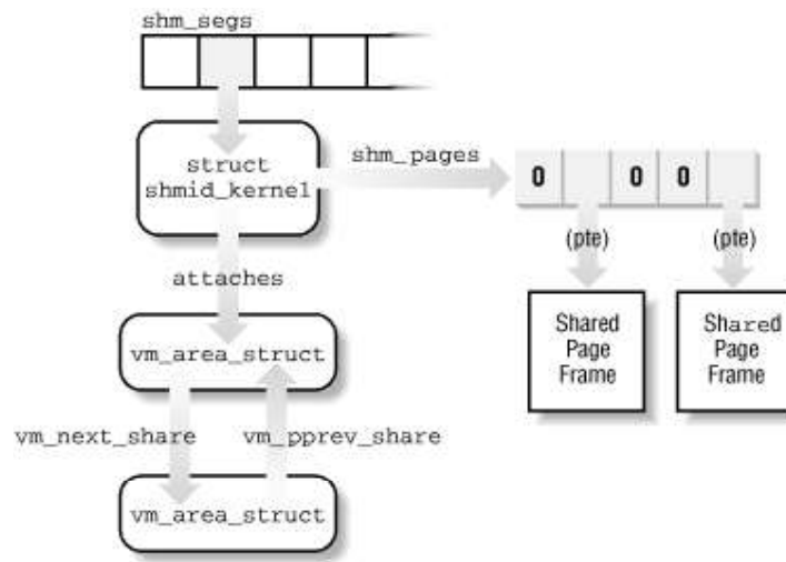
Figure 18-3. IPC shared memory data structures
