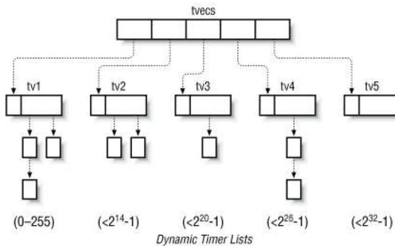
Figure 5-1. The groups of lists associated with dynamic timers
