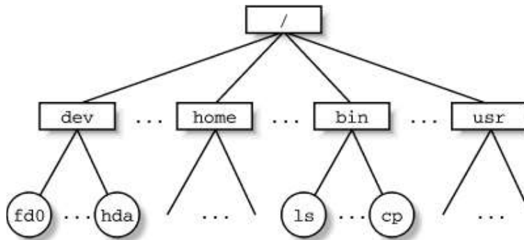
Figure 1-2. An example of a directory tree
