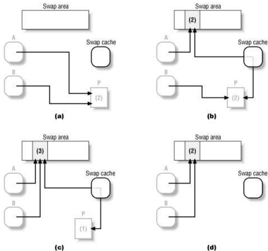
Figure 16-4. The role of the swap cache
