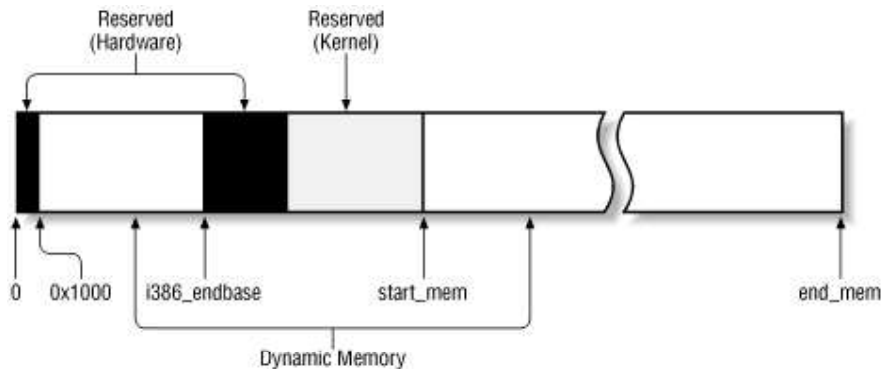
Figure 6-1. Memory layout
