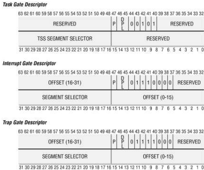
Figure 4-2. Gate descriptors's format
