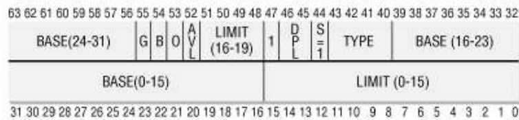
Figure 2-2. Segment Descriptor format
