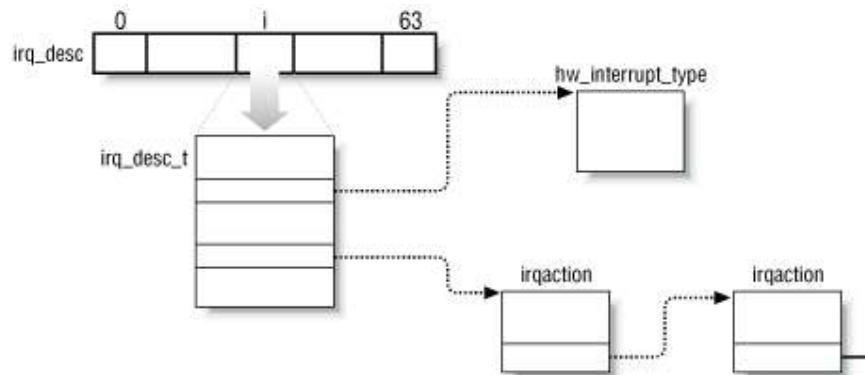
Figure 4-4. IRQ descriptors
