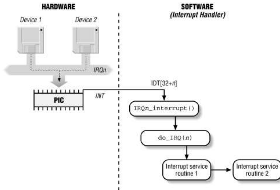
Figure 4-3. Interrupt handling
