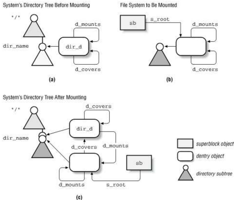
Figure 12-5. Mounting a filesystem
