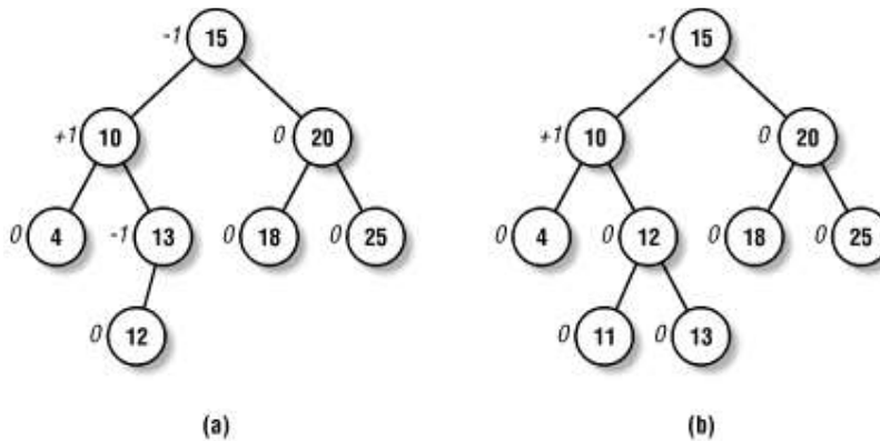
Figure 7-3. Example of AVL trees
