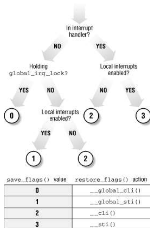
Figure 11-5. Actions performed by save_flags( ) and restore_flags( )
