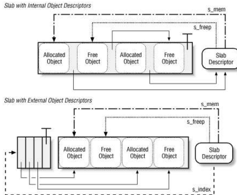
Figure 6-5. Relationships between slab and object descriptors
