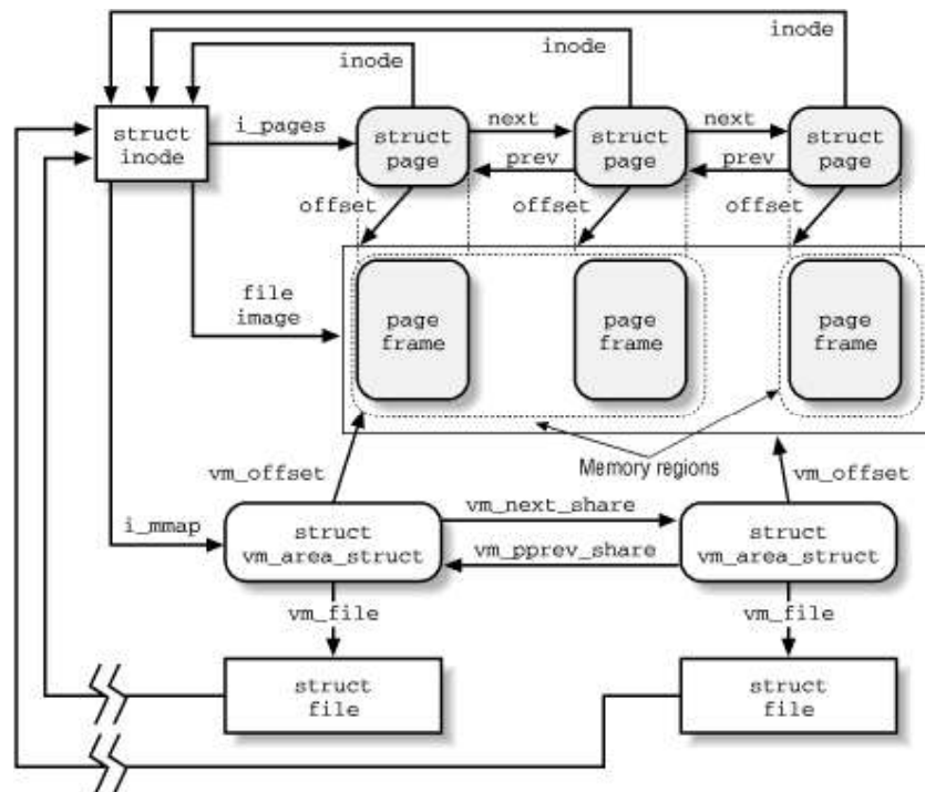
Figure 15-4. Data structures related to memory mapping
