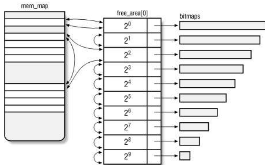
Figure 6-2. Data structures used by the buddy system
