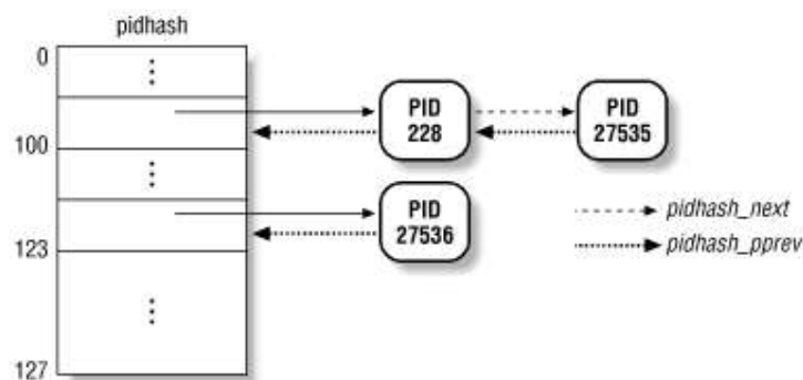
Figure 3-4. The pidhash table and chained lists
