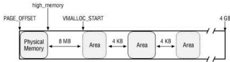
Figure 6-7. The linear address interval starting from PAGE_OFFSET
