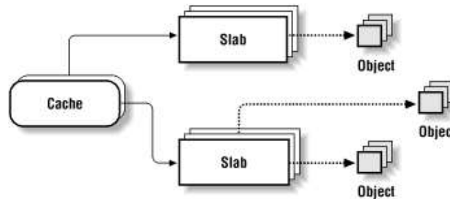
Figure 6-3. The slab allocator components
