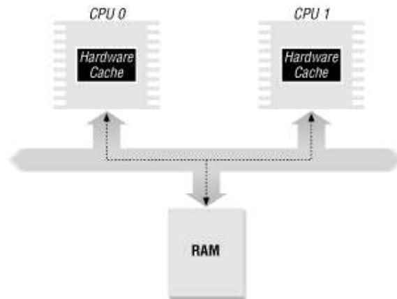
Figure 11-1. The caches in a dual processor
