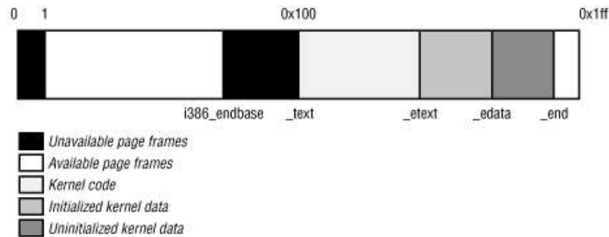
Figure 2-10. The first 512 page frames (2 MB) in Linux 2.2
