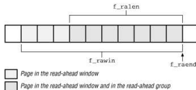
Figure 15-1. Read-ahead window and read-ahead group
