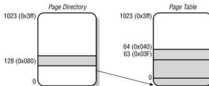
Figure 2-7. An example of paging
