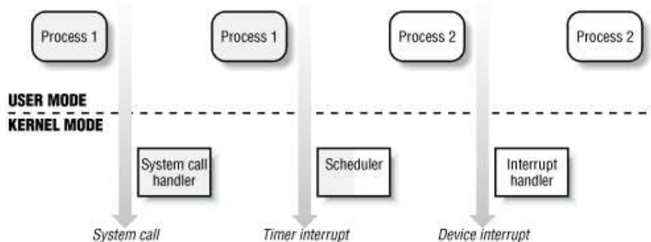
Figure 1-3. Transitions between User and Kernel Mode
