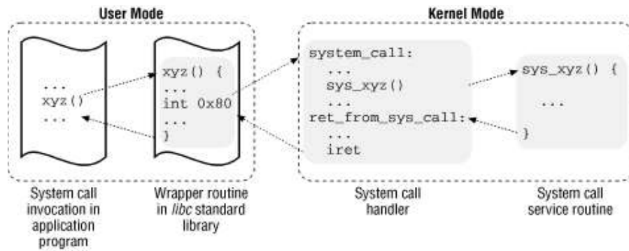
Figure 8-1. Invoking a system call
