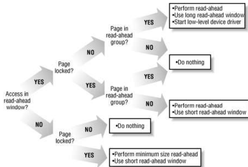
Figure 15-3. Read-ahead scheme
