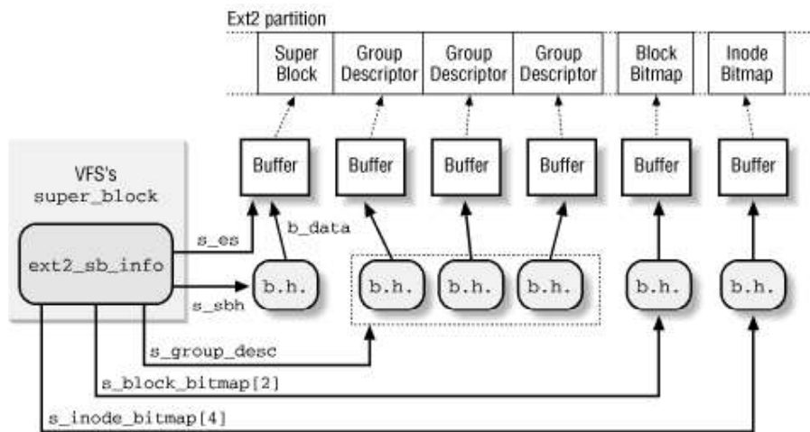
Figure 17-4. Ext2 memory data structures
