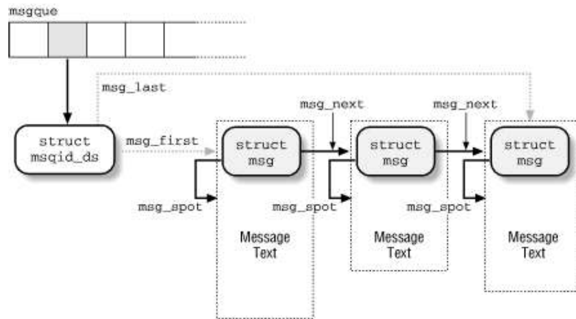
Figure 18-2. IPC message queue data structures
