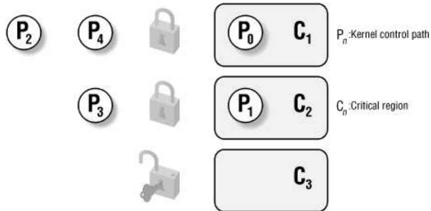
Figure 11-3. Protecting critical regions with several locks
