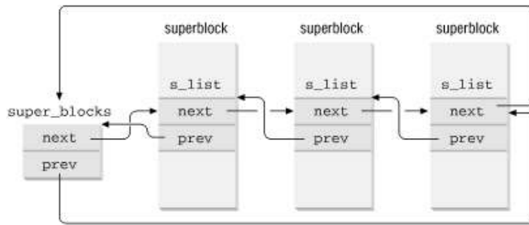
Figure 12-3. The superblock list
