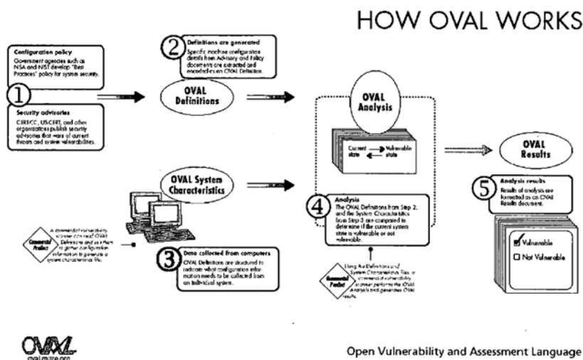
FIGURE 18: Open Vulnerability Assessment Language
